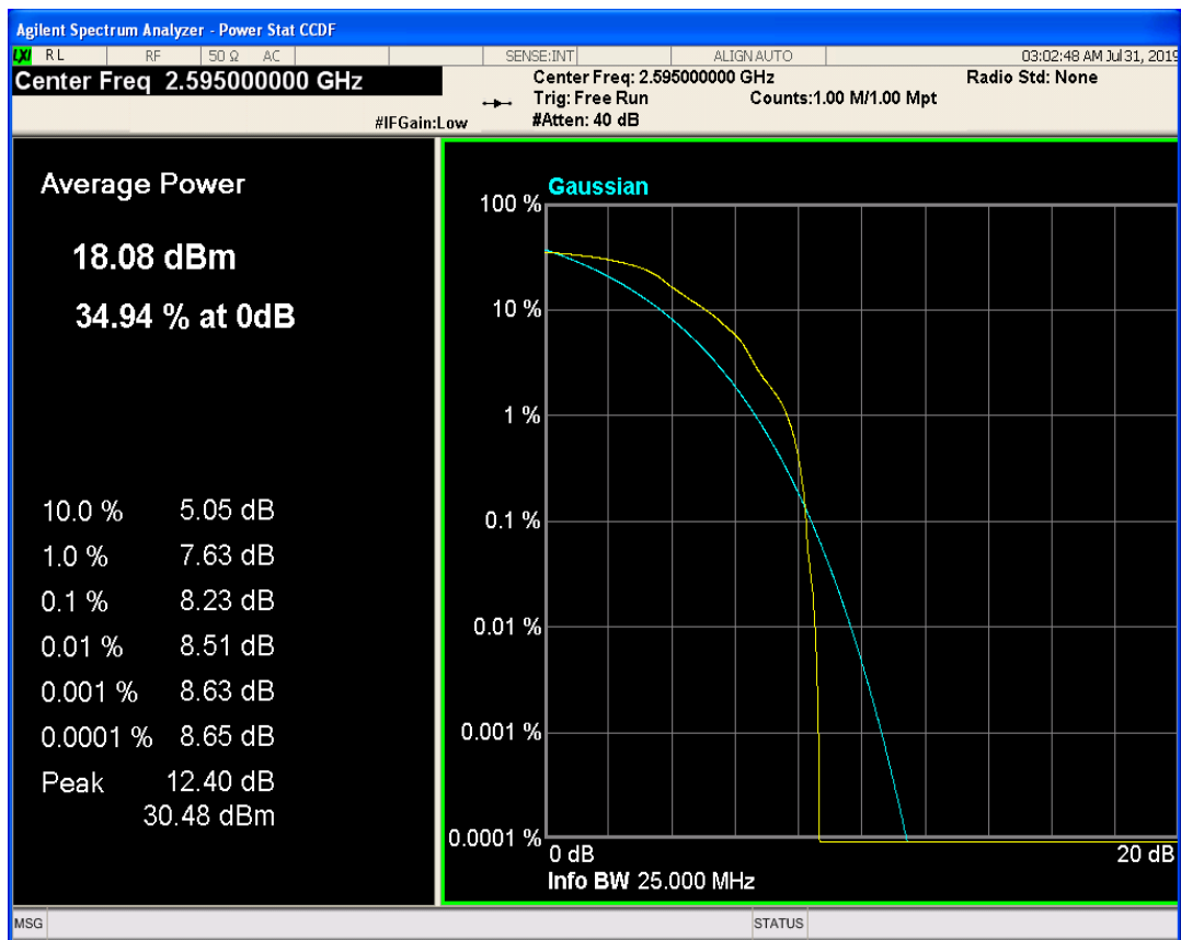
LTE Band41 QAM16 BW=10MHz Channel=40640 RB Size=1 Position=#0
