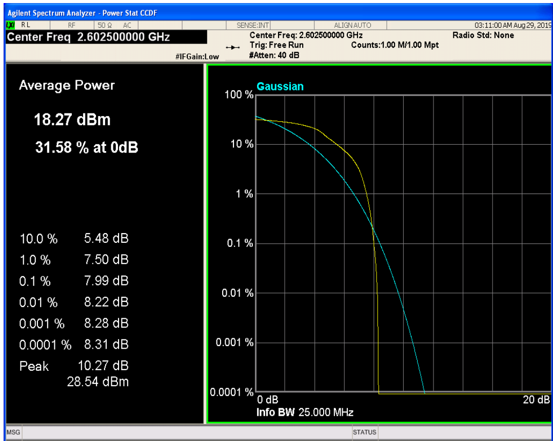
LTE Band41 QPSK BW=15MHz Channel=40715 RB Size=1 Position=#0
