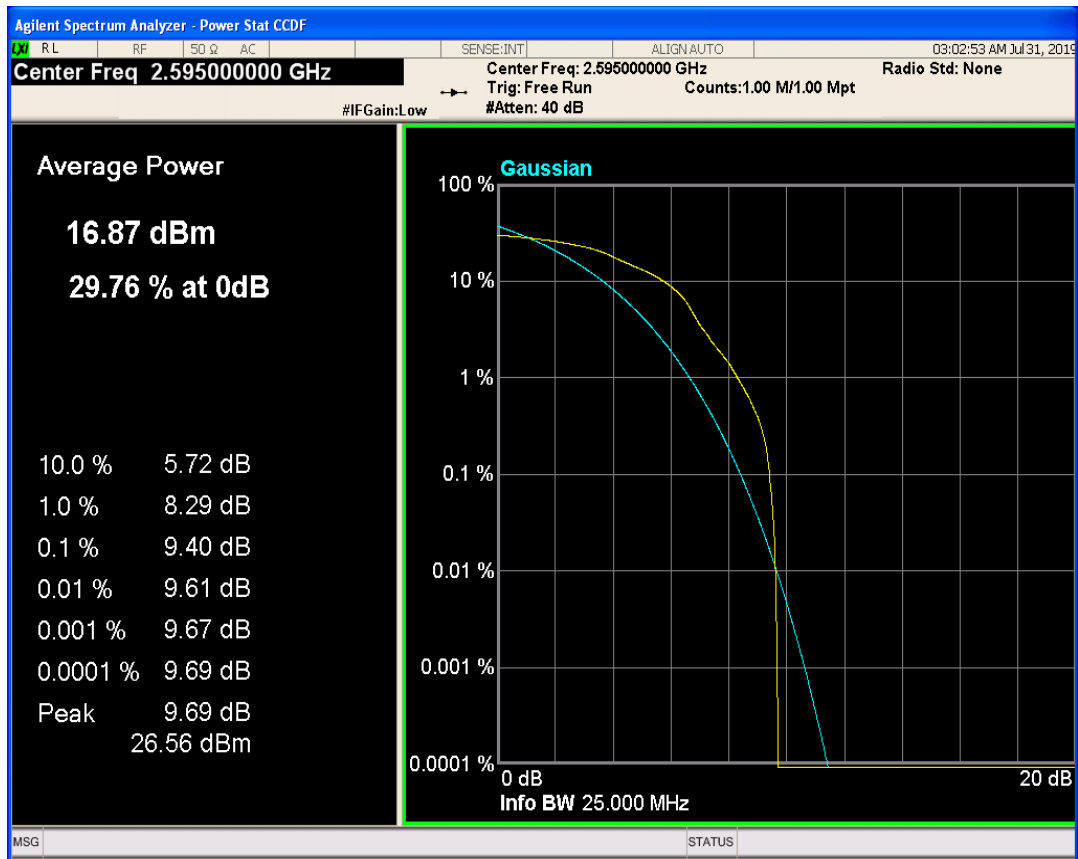
LTE Band41 QPSK BW=5MHz Channel=40640 RB Size=1 Position=#0
