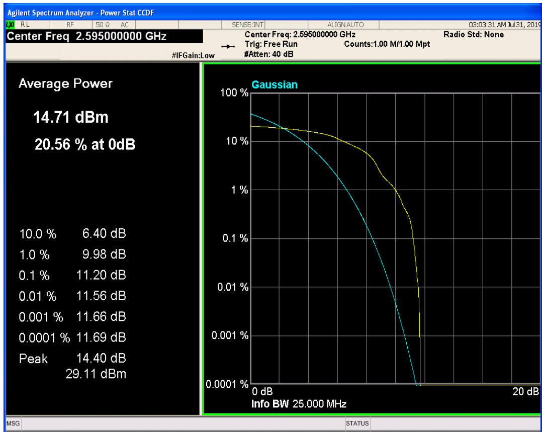
LTE Band41 QPSK BW=10MHz Channel=40640 RB Size=1 Position=#0
