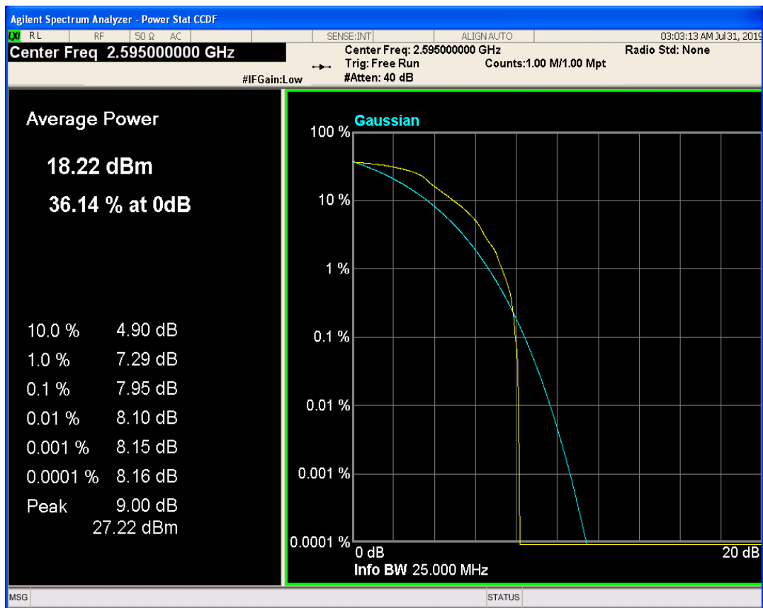
LTE Band41 QAM16 BW=20MHz Channel=40640 RB Size=1 Position=#0
