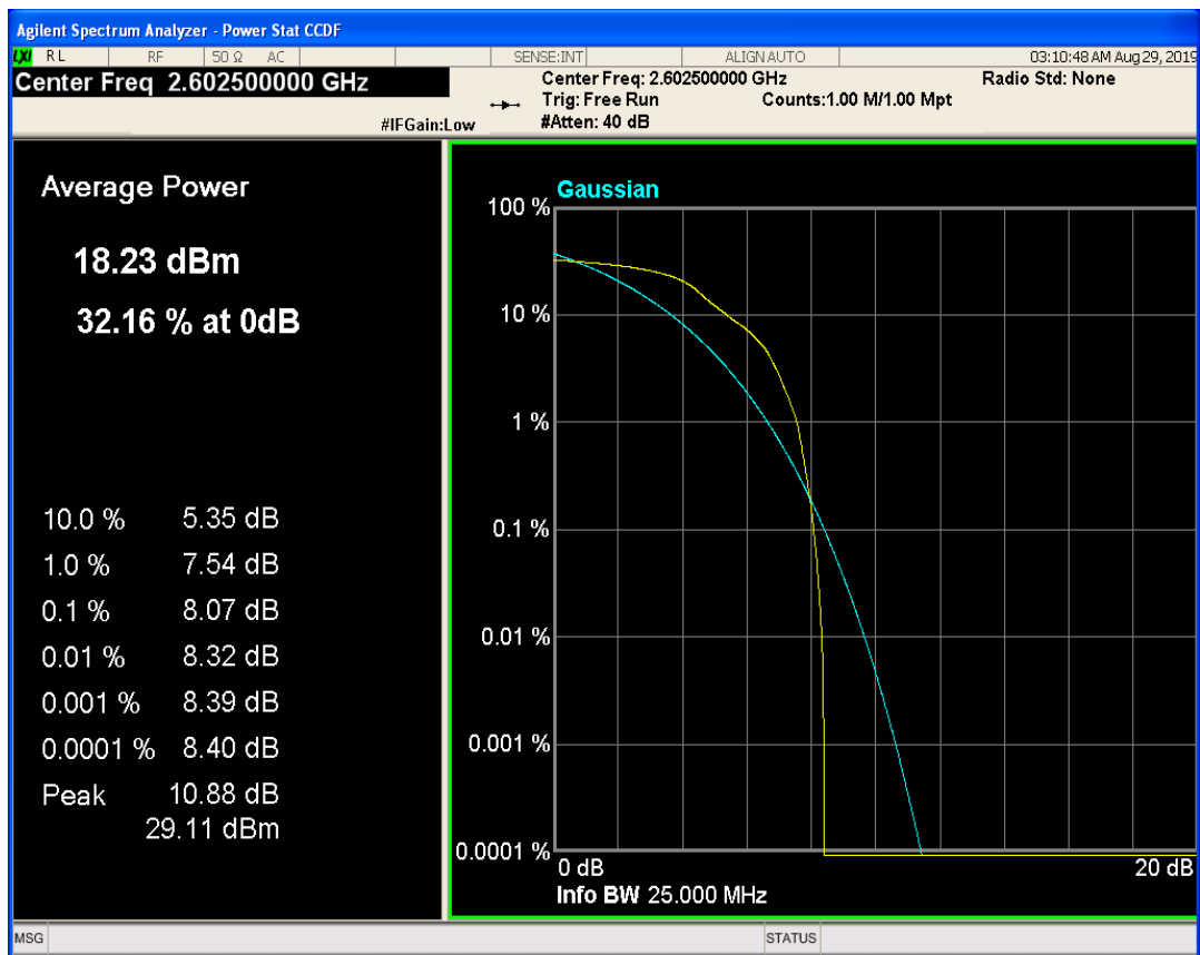
LTE Band41 QAM16 BW=5MHz Channel=40715 RB Size=1 Position=#0
