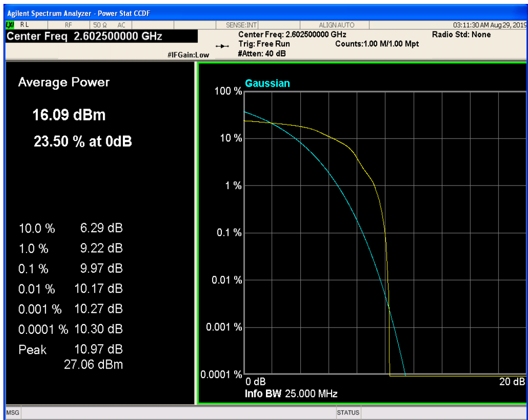
LTE Band41 QPSK BW=20MHz Channel=40715 RB Size=1 Position=#0
