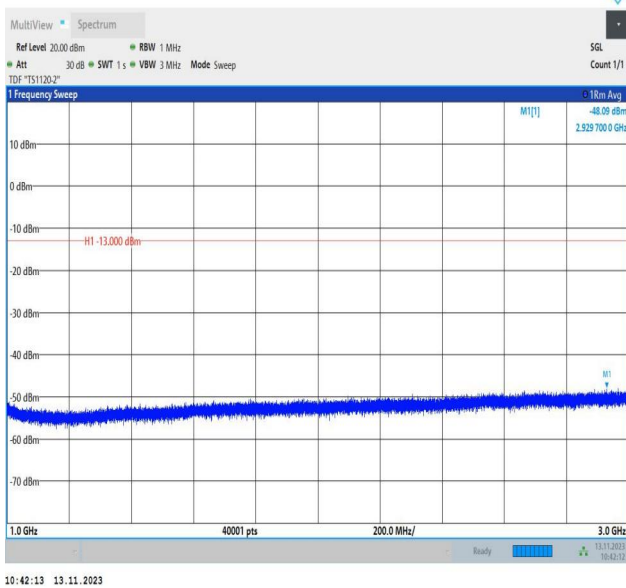
Band5_5MHz_16QAM_20525_1RB#0_1000~3000_1000~3000 0
