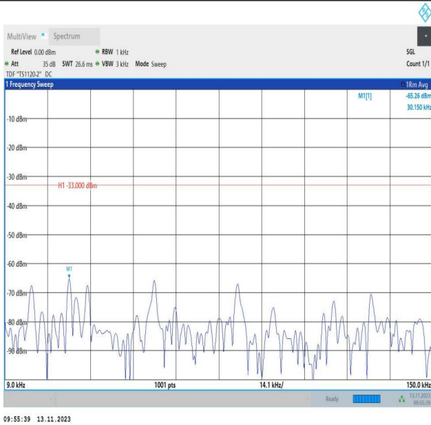
Band5_1.4MHz_QPSK_20525_1RB#0_0.009~0.15_0.009~0.15
