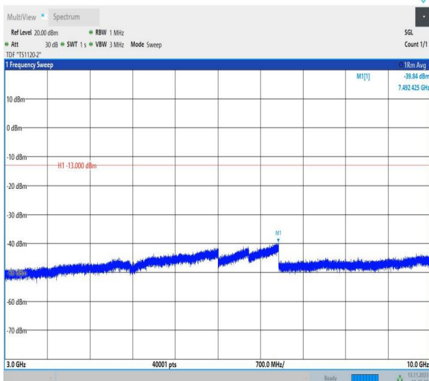
Band5_10MHz_QPSK_20600_1RB#0_3000~10000_3000~10000
