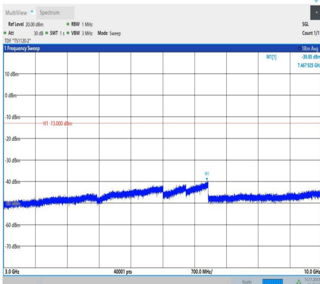
Band5_10MHz_QPSK_20450_1RB#0_3000~10000_3000~10000
