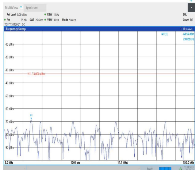
Band5_3MHz_QPSK_20635_1RB#0_1000~3000_1000~3000
