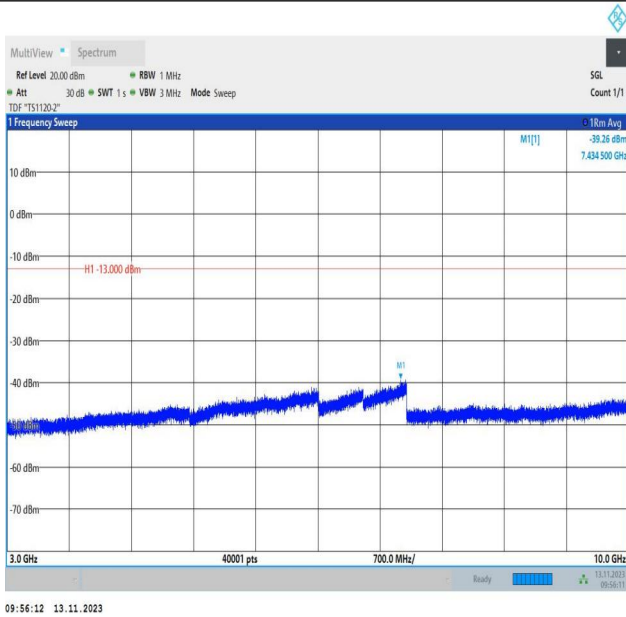
Band5_1.4MHz_QPSK_20525_1RB#0_3000~10000_3000~1 0000
