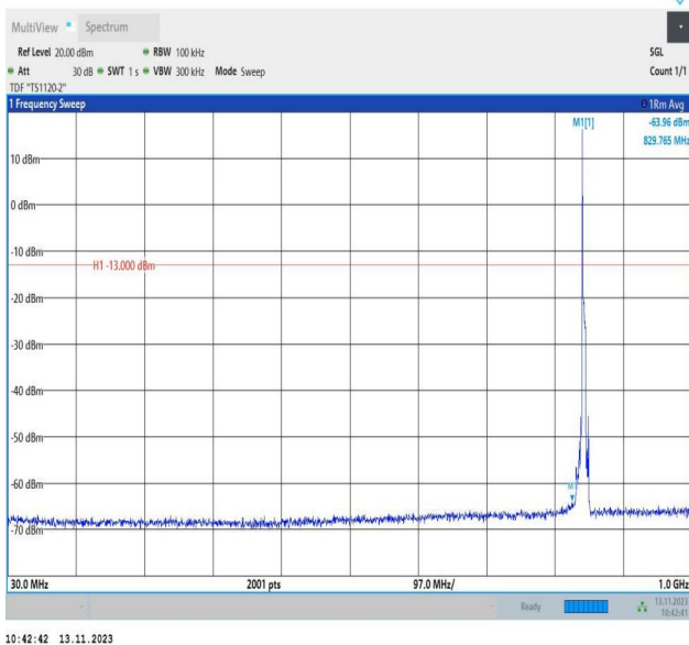
Band5_5MHz_QPSK_20625_1RB#0_30~1000_30~1000
