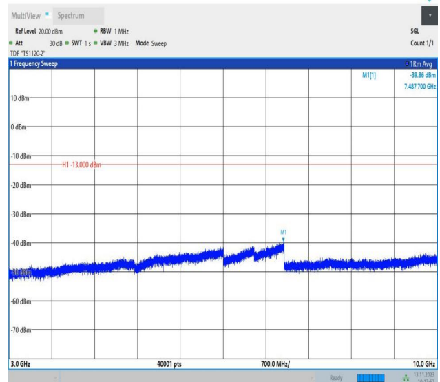
Band5_3MHz_16QAM_20415_1RB#0_3000~10000_3000~10000
