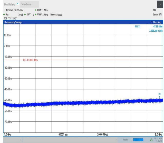
Band5_10MHz_QPSK_20600_1RB#0_1000~3000_1000~3000
