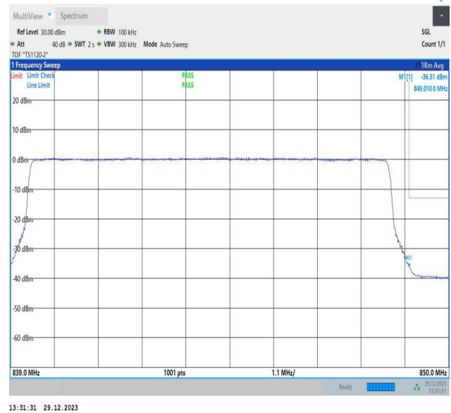
Band5_10MHz_64QAM_20600_50RB#0
