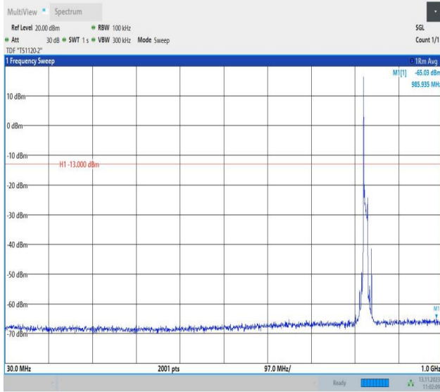
Band5_10MHz_QPSK_20450_1RB#0_30~1000_30~1000
