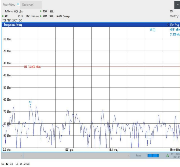
Band5_5MHz_QPSK_20625_1RB#0_0.009~0.15_0.009~0.15
