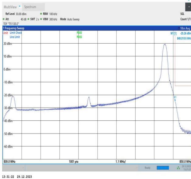
Band5_10MHz_64QAM_20600_1RB#49
