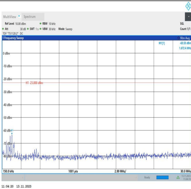
Band5_10MHz_16QAM_20525_1RB#0_0.15~30_0.15~30
