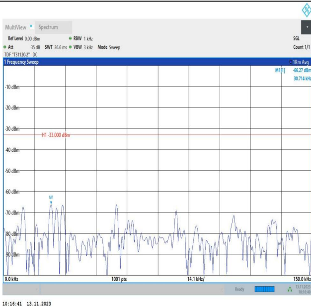
Band5_3MHz_QPSK_20415_1RB#0_0.009~0.15_0.009~0.15
