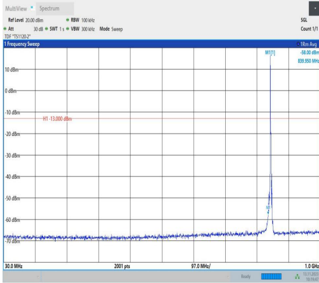
Band5_3MHz_QPSK_20635_1RB#0_30~1000_30~1000
