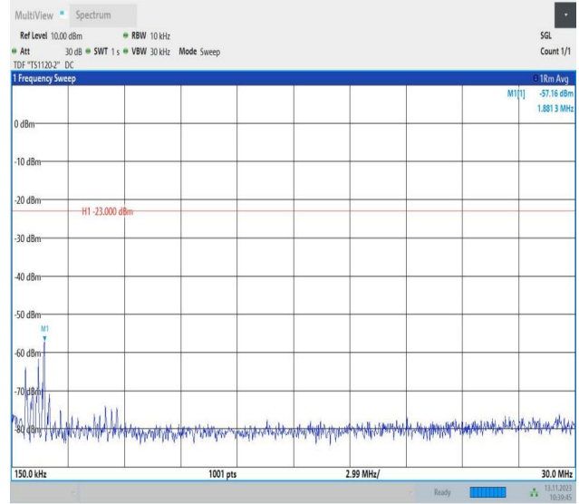
Band5_5MHz_QPSK_20425_1RB#0_0.15~30_0.15~30
