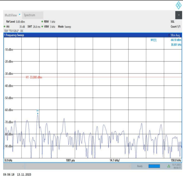
Band5_1.4MHz_16QAM_20525_1RB#0_0.009~0.15_0.009~0. 15
