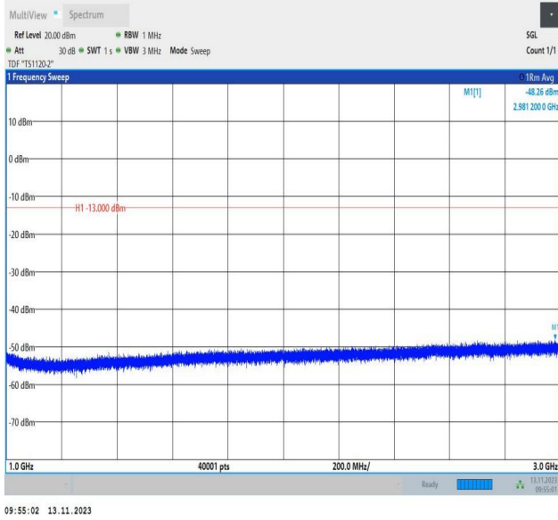
Band5_1.4MHz_16QAM_20407_1RB#0_1000~3000_1000~3000
