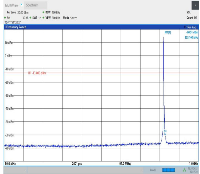
Band5_3MHz_16QAM_20415_1RB#0_30~1000_30~1000
