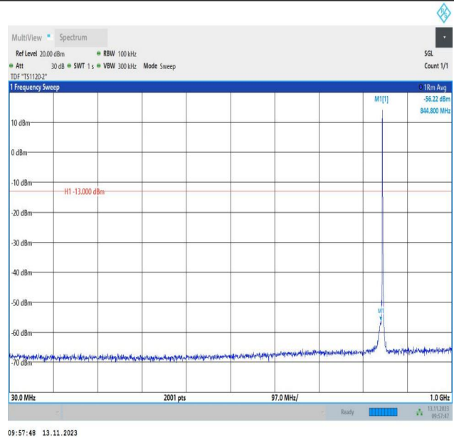
Band5_1.4MHz_16QAM_20643_1RB#0_30~1000_30~1000
