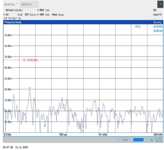
Band5_1.4MHz_16QAM_20643_1RB#0_0.009~0.15_0.009~0.15
