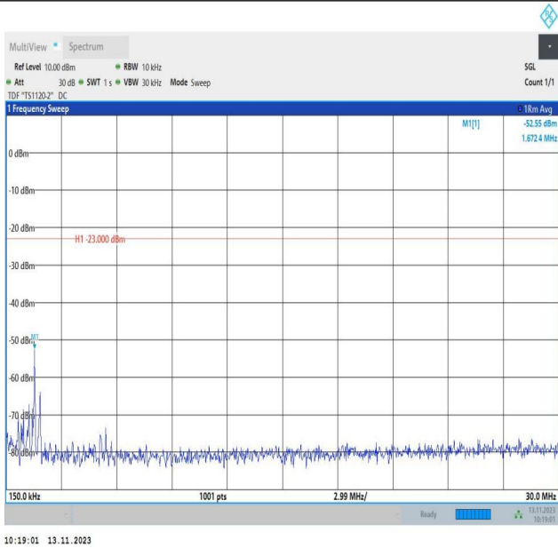
Band5_3MHz_16QAM_20525_1RB#0_0.15~30_0.15~30
