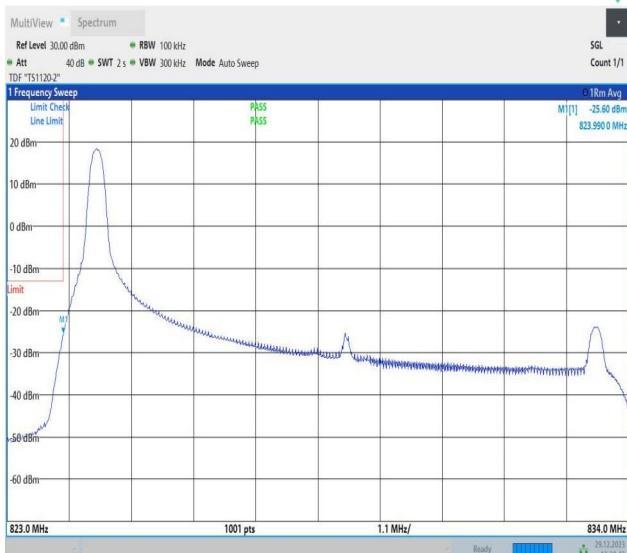
Band5_10MHz_64QAM_20450_1RB#0
