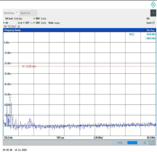
Band5_1.4MHz_QPSK_20525_1RB#0_0.15~30_0.15~30
