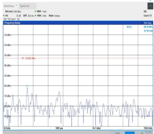
Band5_10MHz_16QAM_20600_1RB#0_0.009~0.15_0.009~0.15
