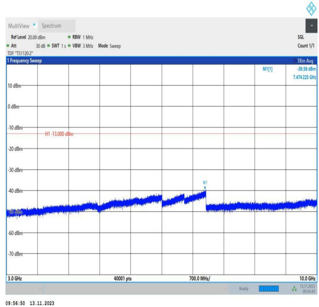
Band5_1.4MHz_16QAM_20525_1RB#0_3000~10000_3000~10000
