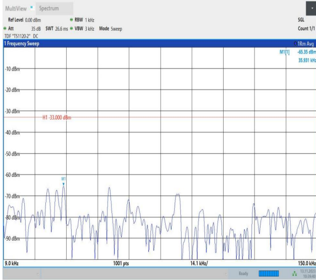
Band5_5MHz_QPSK_20425_1RB#0_0.009~0.15_0.009~0.15
