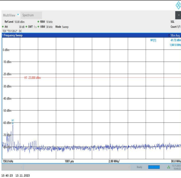
Band5_5MHz_16QAM_20425_1RB#0_0.15~30_0.15~30
