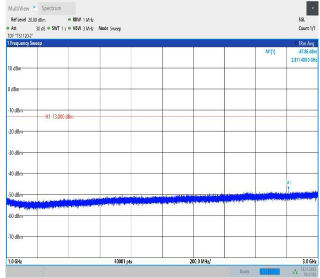
Band5_3MHz_QPSK_20415_1RB#0_1000~3000_1000~3000
