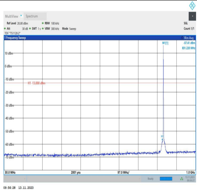
Band5_1.4MHz_16QAM_20525_1RB#0_30~1000_30~1000
