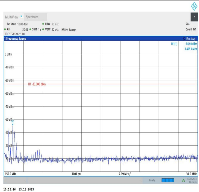
Band5_3MHz_QPSK_20415_1RB#0_0.15~30_0.15~30
