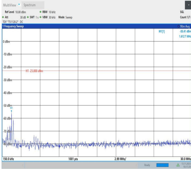
Band5_3MHz_16QAM_20415_1RB#0_0.15~30_0.15~30
