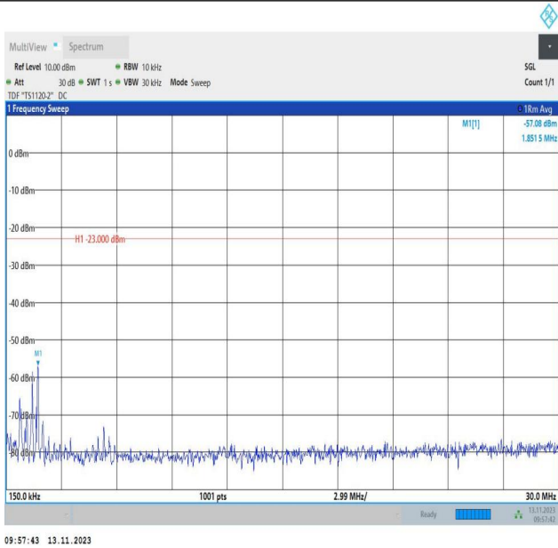
Band5_1.4MHz_16QAM_20643_1RB#0_0.15~30_0.15~30
