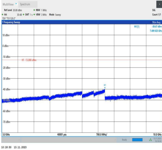
Band5_3MHz_QPSK_20525_1RB#0_3000~10000_3000~10000
