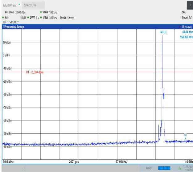
Band5_10MHz_QPSK_20600_1RB#0_30~1000_30~1000
