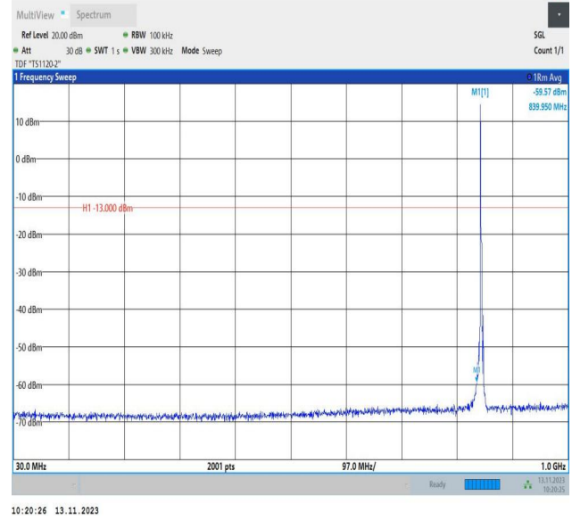
Band5_3MHz_16QAM_20635_1RB#0_30~1000_30~1000
