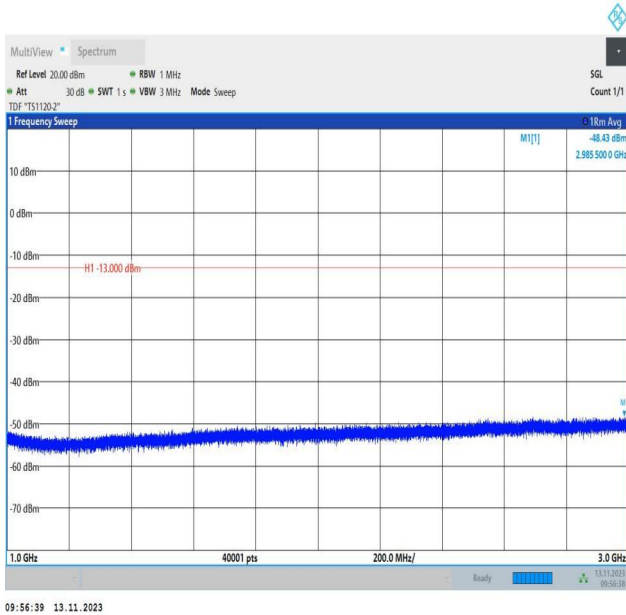
Band5_1.4MHz_16QAM_20525_1RB#0_1000~3000_1000~3000
