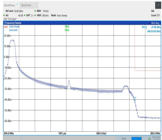
Band5_5MHz_64QAM_20625_1RB#0
