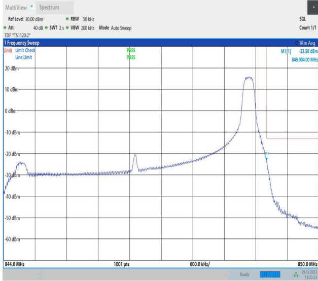
Band5_5MHz_64QAM_20625_1RB#24
