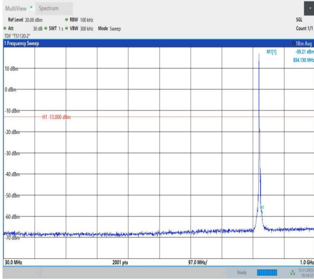
Band5_3MHz_QPSK_20415_1RB#0_30~1000_30~1000
