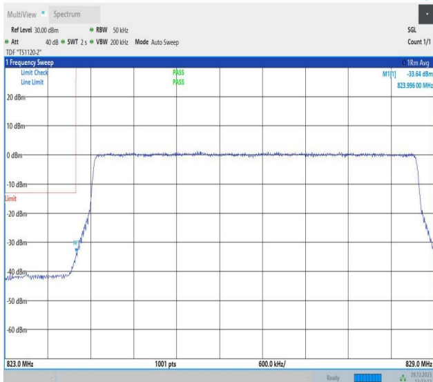
Band5_5MHz_64QAM_20425_25RB#0
