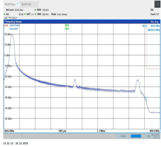
Band5_10MHz_64QAM_20600_1RB#0
