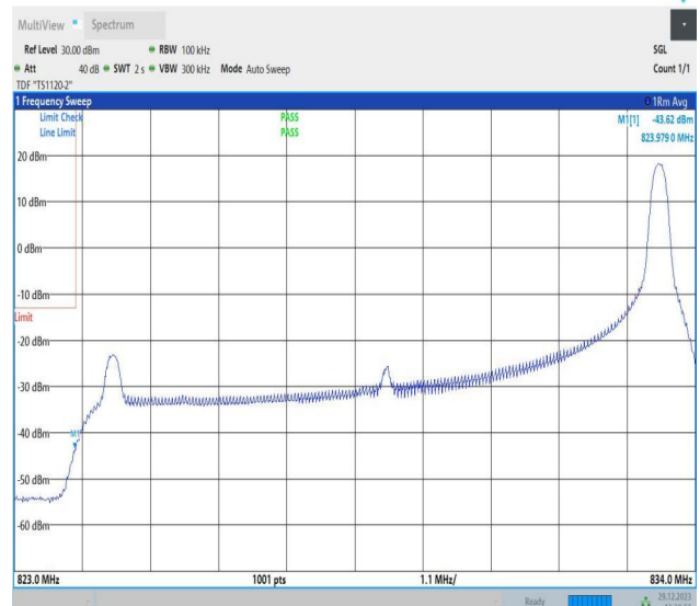
Band5_10MHz_64QAM_20450_1RB#49
