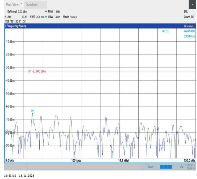
Band5_5MHz_16QAM_20625_1RB#0_0.009~0.15_0.009~0.15
