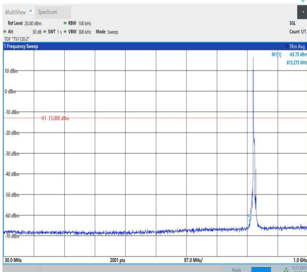
Band5_5MHz_QPSK_20425_1RB#0_30~1000_30~1000
