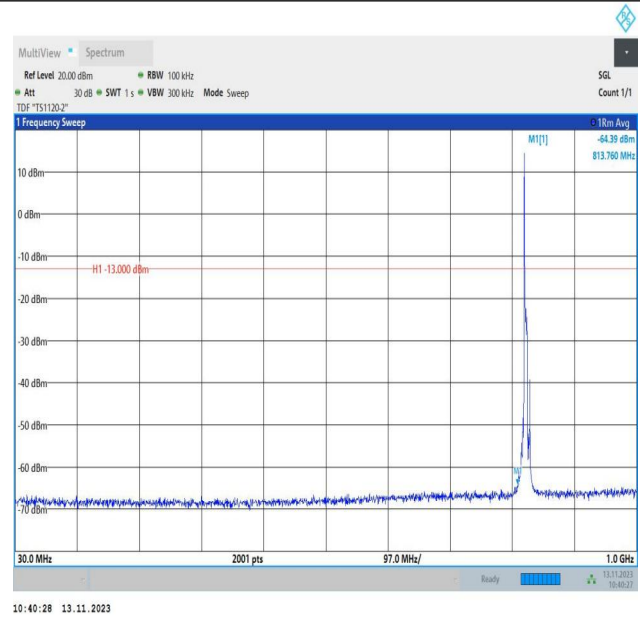
Band5_5MHz_16QAM_20425_1RB#0_30~1000_30~1000
