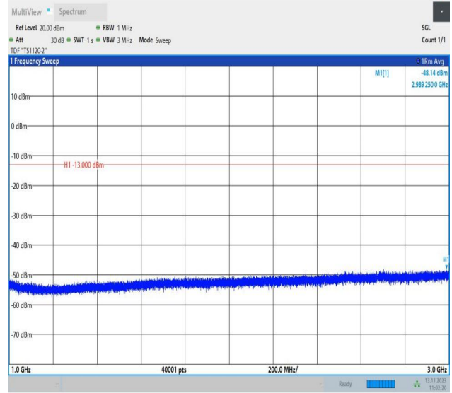
Band5_10MHz_QPSK_20450_1RB#0_1000~3000_1000~3000
