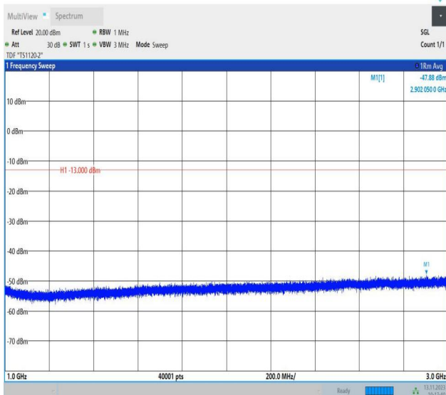
Band5_3MHz_16QAM_20415_1RB#0_1000~3000_1000~3000
