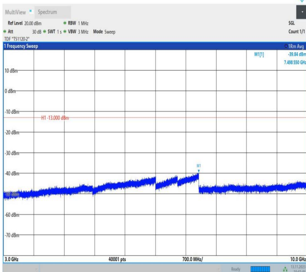
Band5_5MHz_QPSK_20525_1RB#0_3000~10000_3000~10000
