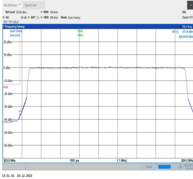
Band5_10MHz_64QAM_20450_50RB#0
