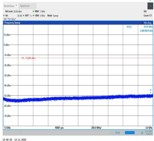
Band5_5MHz_QPSK_20625_1RB#0_1000~3000_1000~3000
