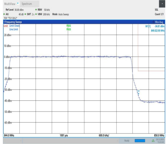
Band5_5MHz_64QAM_20625_25RB#0
