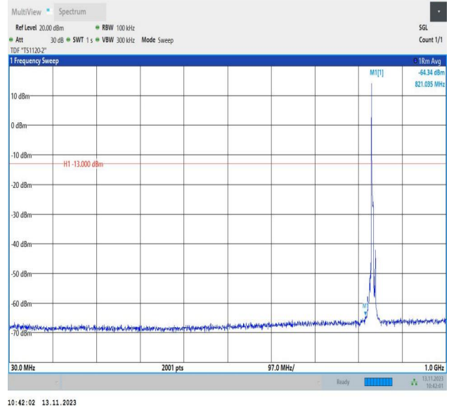
Band5_5MHz_16QAM_20525_1RB#0_30~1000_30~1000
