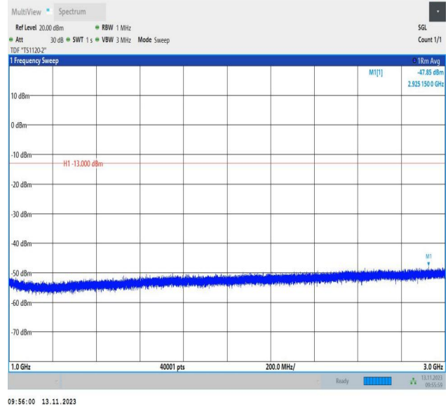
Band5_1.4MHz_QPSK_20525_1RB#0_1000~3000_1000~300 0
