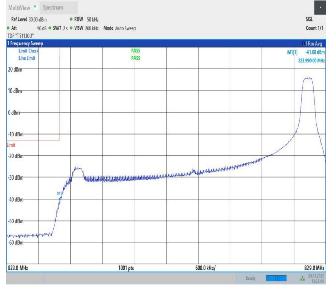
Band5_5MHz_64QAM_20425_1RB#24
