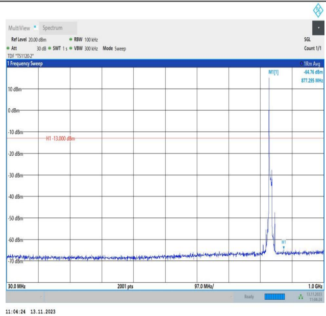
Band5_10MHz_16QAM_20525_1RB#0_30~1000_30~1000
