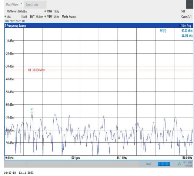
Band5_5MHz_16QAM_20425_1RB#0_0.009~0.15_0.009~0.15
