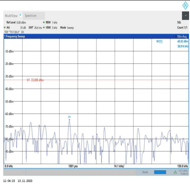
Band5_10MHz_16QAM_20525_1RB#0_0.009~0.15_0.009~0.15
