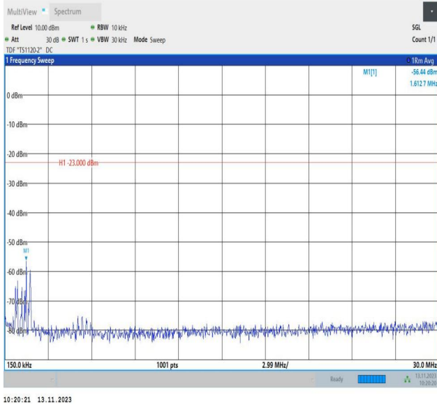
Band5_3MHz_16QAM_20635_1RB#0_0.15~30_0.15~30
