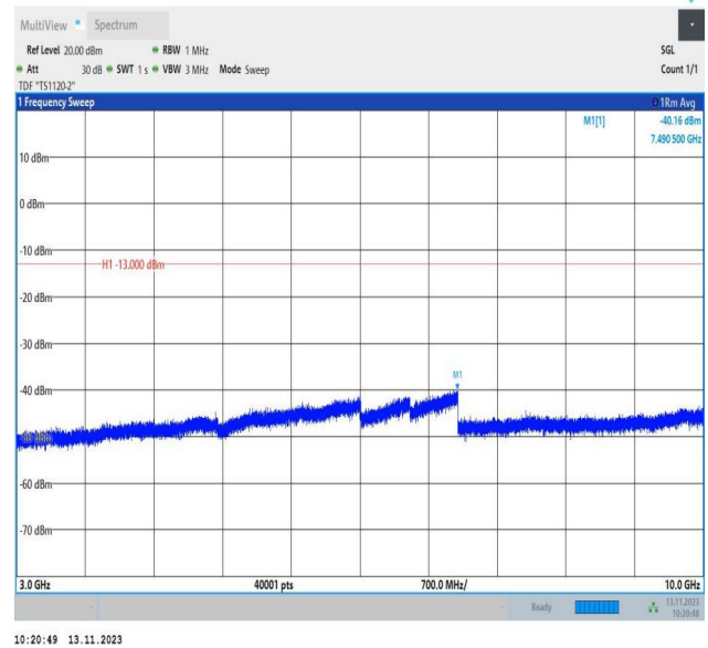
Band5_3MHz_16QAM_20635_1RB#0_3000~10000_3000~10000 00
