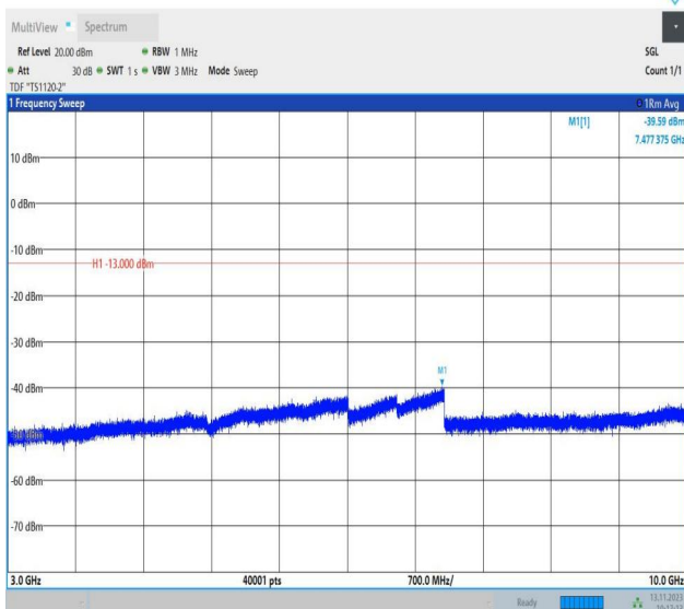
Band5_3MHz_QPSK_20415_1RB#0_3000~10000_3000~10000
