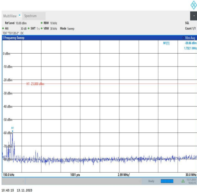
Band5_5MHz_16QAM_20625_1RB#0_0.15~30_0.15~30
