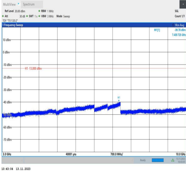
Band5_5MHz_QPSK_20625_1RB#0_3000~10000_3000~10000
