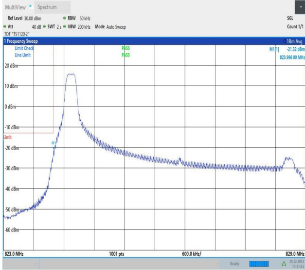
Band5_5MHz_64QAM_20425_1RB#0
