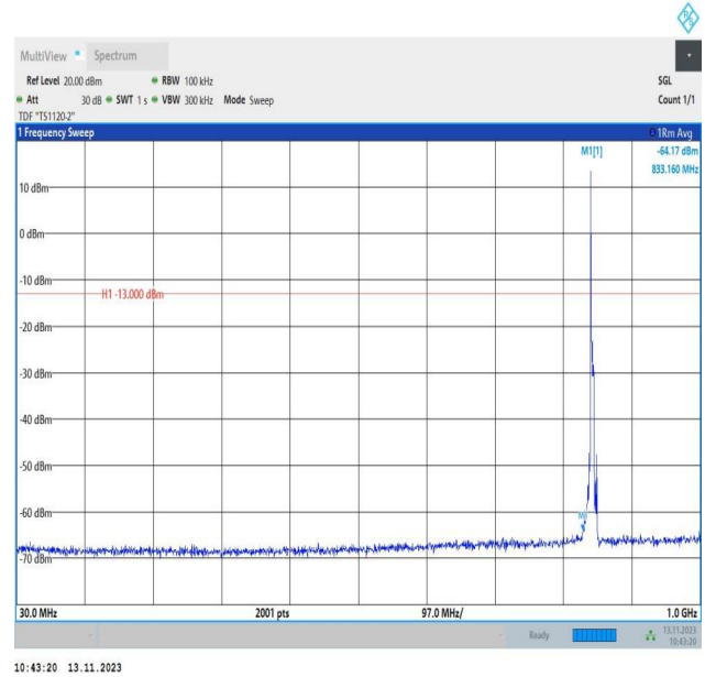
Band5_5MHz_16QAM_20625_1RB#0_30~1000_30~1000
