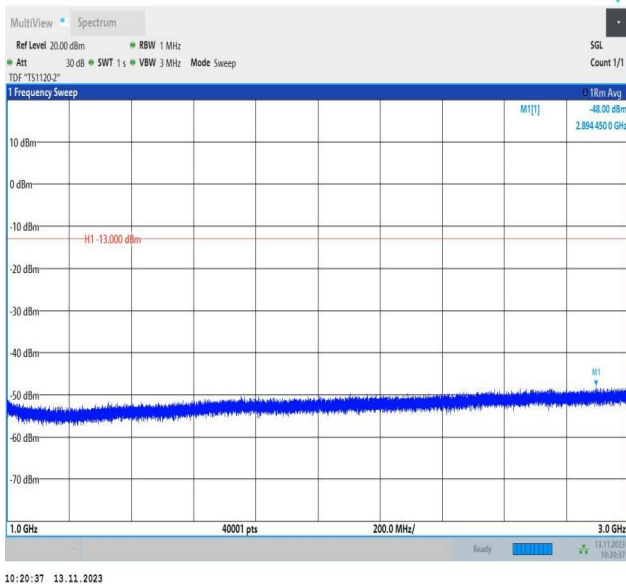
Band5_3MHz_16QAM_20635_1RB#0_1000~3000_1000~3000 0
