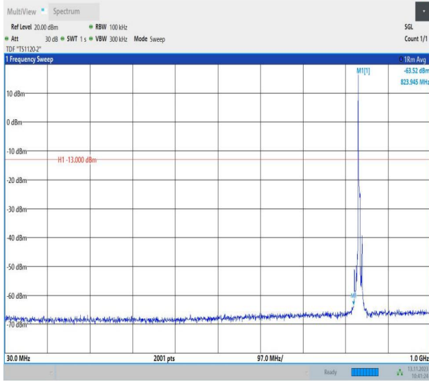
Band5_5MHz_QPSK_20525_1RB#0_30~1000_30~1000
