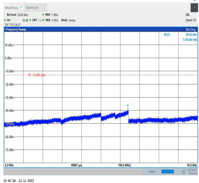
Band5_5MHz_16QAM_20525_1RB#0_3000~10000_3000~10000 00
