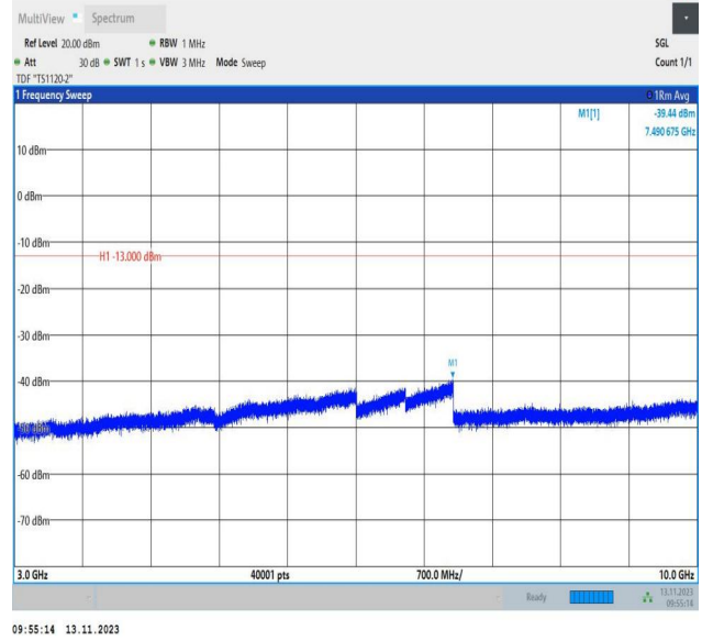
Band5_1.4MHz_16QAM_20407_1RB#0_3000~10000_3000~10000
