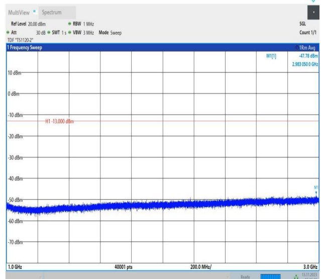
Band5_5MHz_QPSK_20425_1RB#0_1000~3000_1000~3000
