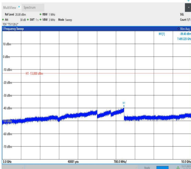
Band5_3MHz_QPSK_20635_1RB#0_3000~10000_3000~10000
