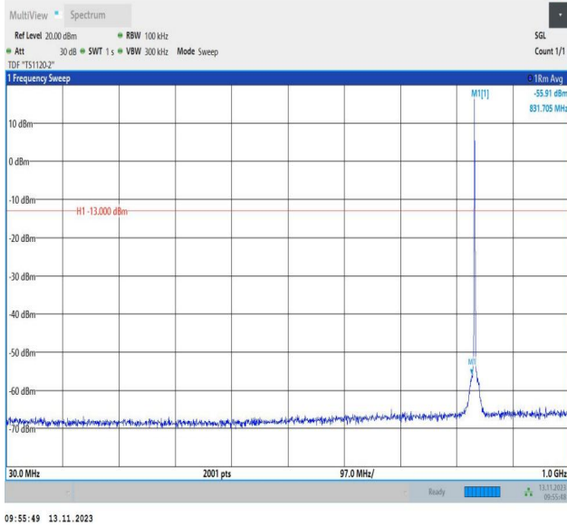
Band5_1.4MHz_QPSK_20525_1RB#0_30~1000_30~1000
