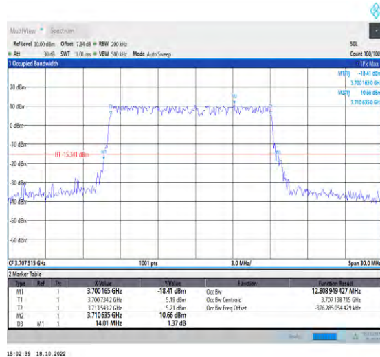
1-N77-3700-3980-PC2-30-15-L-5-DFT-256QAM-Outer_Full-36@0-Ant1-12.809-14.010-≤15-PASS
