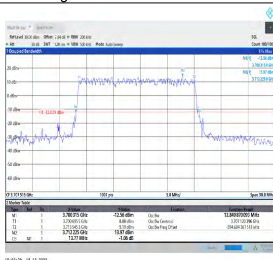
1-N77-3700-3980-PC2-30-15-L-3-DFT-16QAM-Outer_Full-36@0-Ant1-12.85-13.770-≤15-PASS
