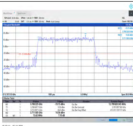
1-N77-3700-3980-PC2-30-15-L-1-DFT-QPSK-Outer_Full-36@0-Ant1-12.8-13.620-≤15-PASS
