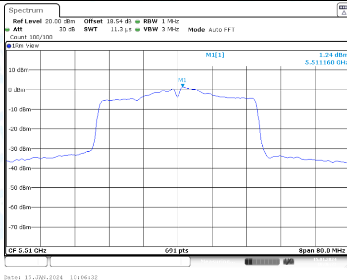
11AC40-CDD_Ant2_5510
