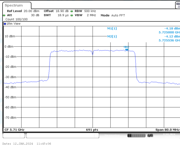
11AX40-CDD_Ant2_5710_UNII-3
