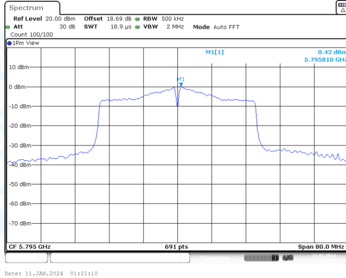
11AC40-CDD_Ant2_5795
