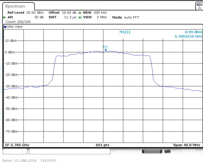
11AX20-CDD_Ant2_5785
