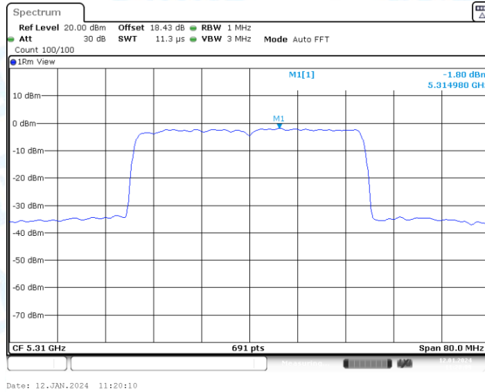
11AX40-CDD_Ant2_5310
