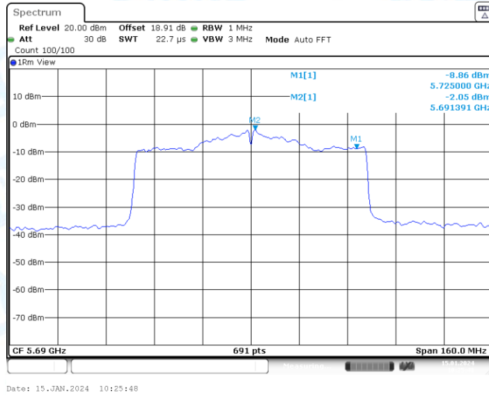
11AC80-CDD_Ant1_5690_UNII-3
