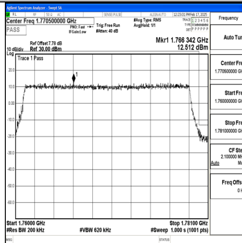
Band66_20MHz_16QAM_132572_100RB#0
