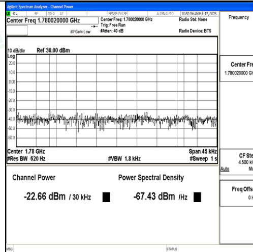
Band66_3MHz_16QAM_132657_15RB#0_Final1
