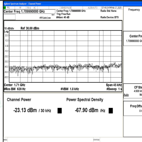
Band66_3MHz_QPSK_131987_15RB#0_Final1
