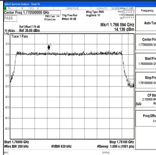
Band66_20MHz_QPSK_132572_100RB#0
