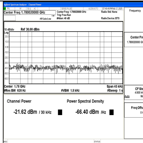
Band66_3MHz_QPSK_132657_15RB#0_Final1
