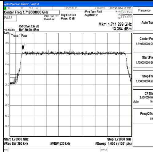
Band66_20MHz_16QAM_132072_100RB#0
