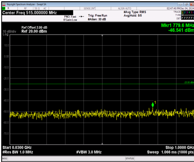
Band38-5MHz-64QAM-38225-1RB#0-Range1:30~1000MHz
