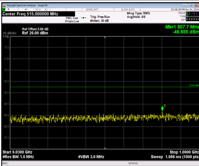
Band38-20MHz-QPSK-37850-1RB#0-Range1:30~1000MHz
