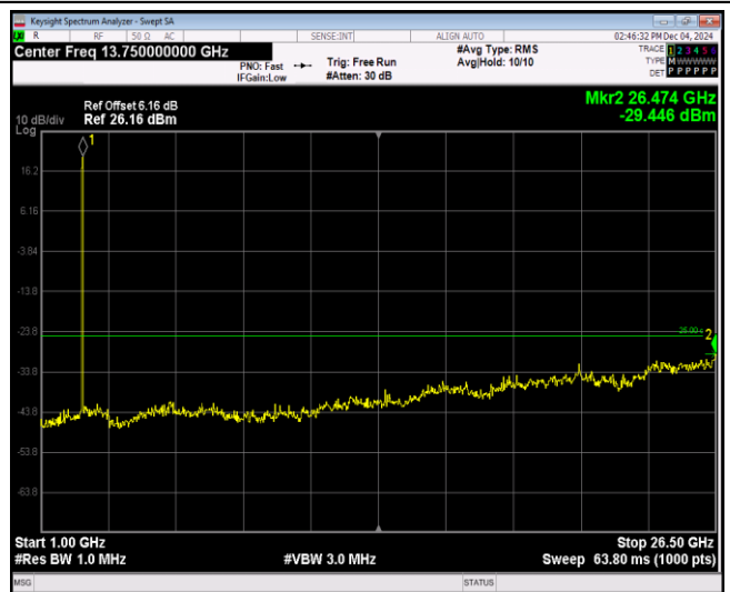
Band38-5MHz-16QAM-38000-1RB#0-Range2:1000~ 26500MHz
