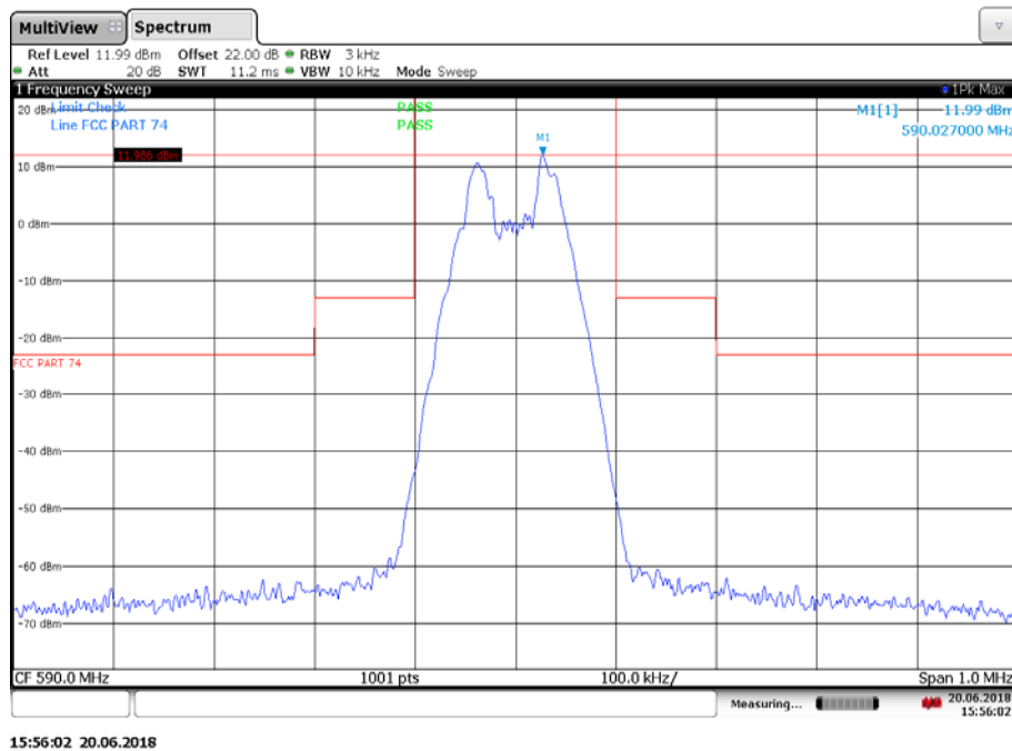
Plot 3: 590.000 MHz, spectrum mask
