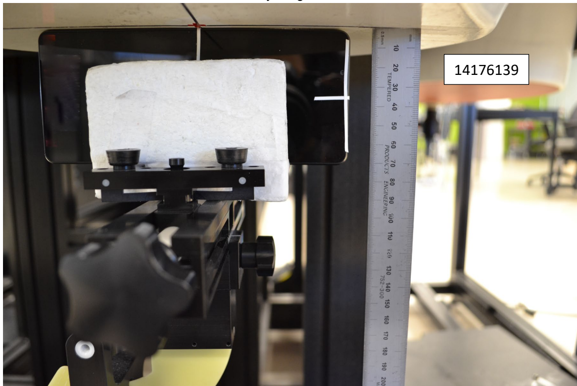
Extremity, Edge 4, 0 mm
