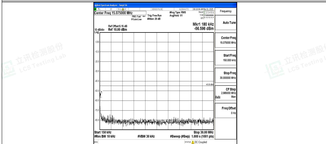
Band7_10MHz_QPSK_20800_1RB#0_0.15~30_0.15~30
