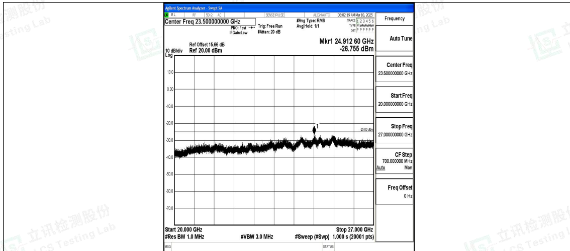
Band7_5MHz_16QAM_21425_1RB#0_20000~27000_20000~27000
