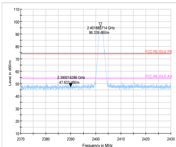
Fig.73 Radiated emission (Power): 8DPSK, low channel
