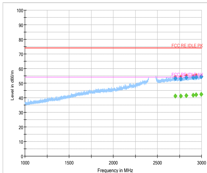
Fig.71 Radiated emission: 8DPSK, Ch0, 1GHz~3GHz
