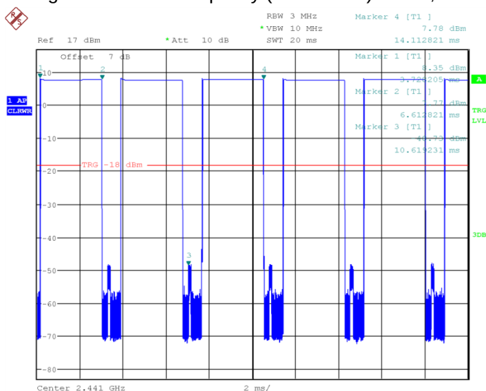
Fig 82. Time of occupancy (Dwell Time): Ch39,Packet DH5
