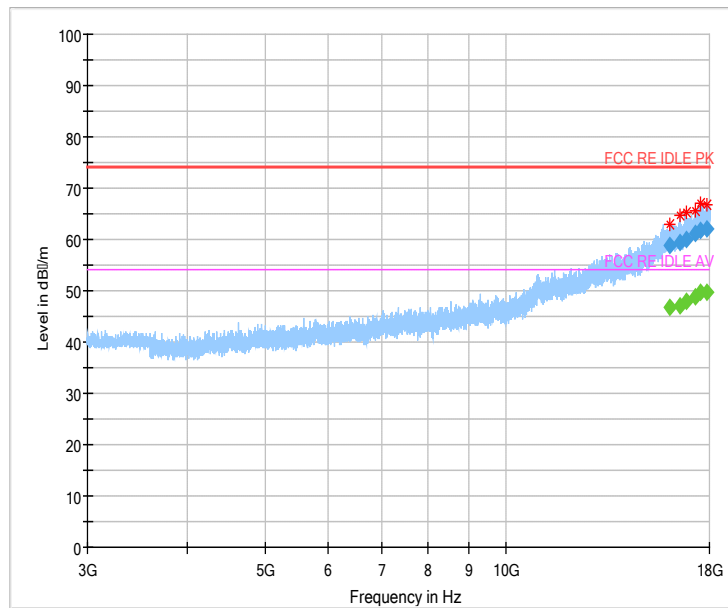
Fig.60 Radiated emission: GFSK, Ch0, 3GHz~18GHz
