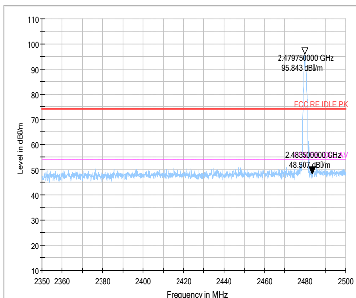
Fig.68 Radiated emission (Power): \pi/4 DQPSK, high channel
