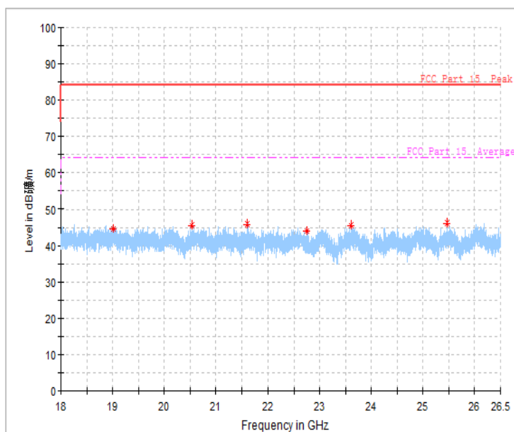
Fig.63 Radiated emission: GFSK, 18 GHz - 26 GHz
