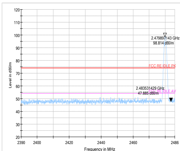
Fig.62 Radiated emission (Power): GFSK, high channel
