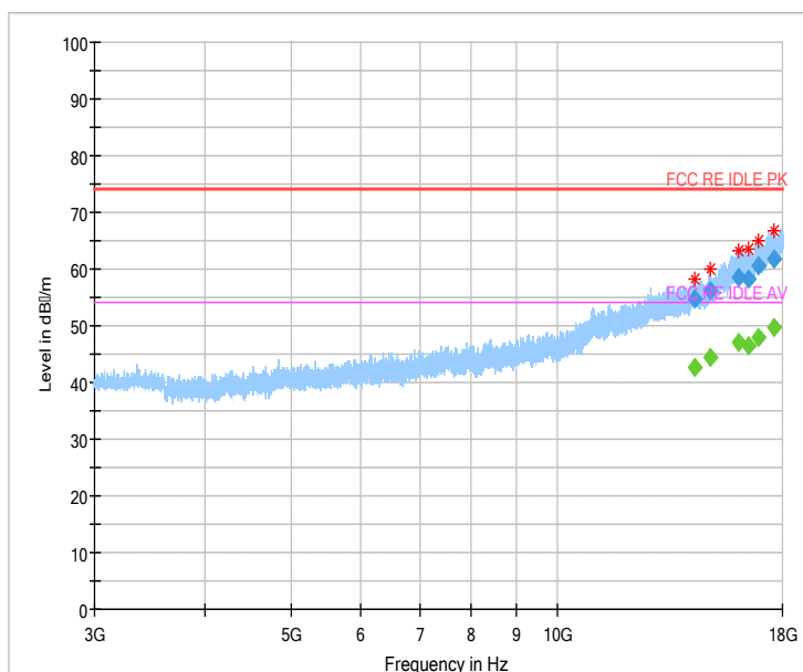
Fig.72 Radiated emission: 8DPSK, Ch0, 3GHz~18GHz
