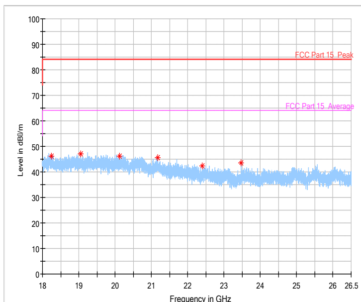
Fig.45 Radiated emission: GFSK, 18 GHz - 26 GHz
