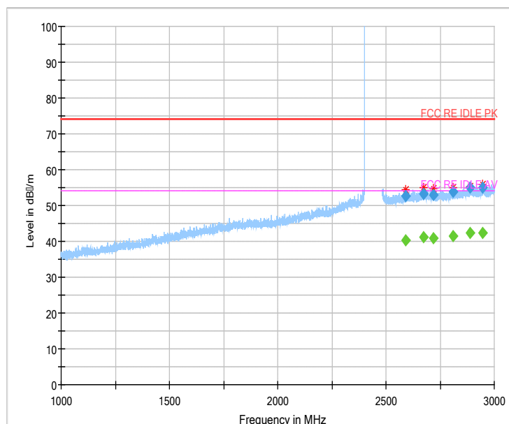
Fig.65 Radiated emission: \pi/4 DQPSK, Ch0, 1GHz~3GHz
