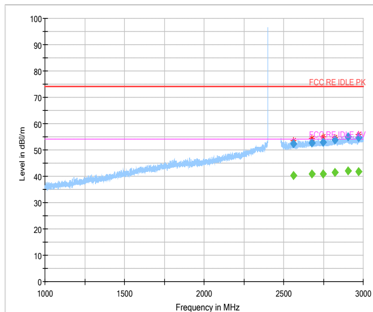
Fig.59 Radiated emission: GFSK, Ch0, 1GHz~3GHz
