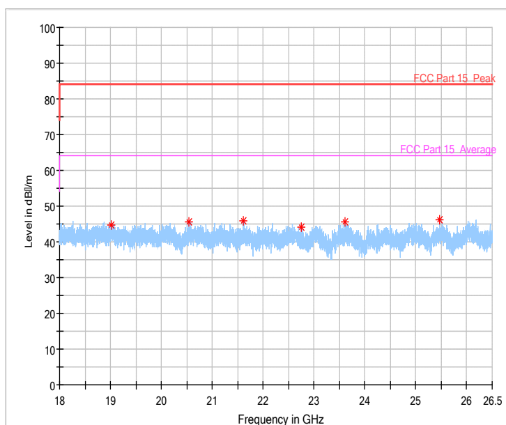
Fig.69 Radiated emission: \pi/4 DQPSK, 18 GHz - 26 GHz
