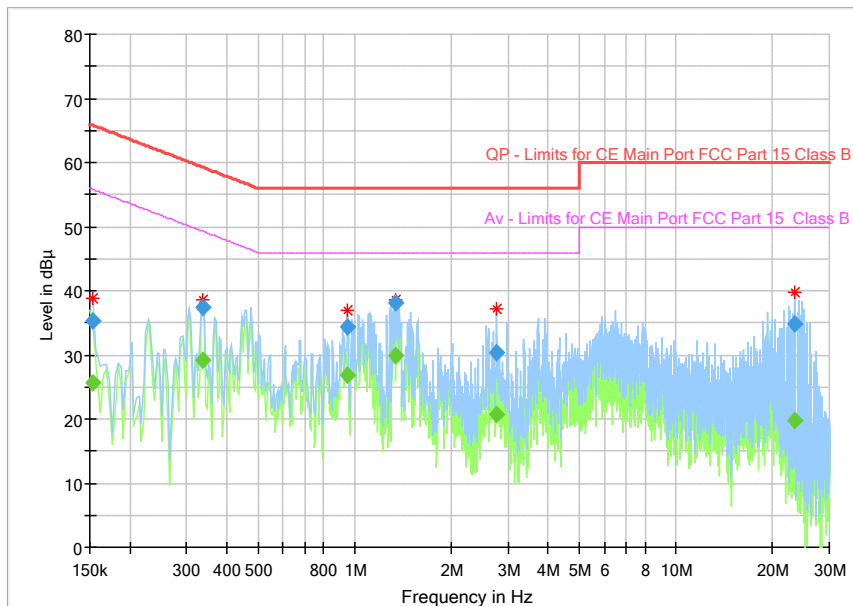
Fig.77 AC Conducted Emission
