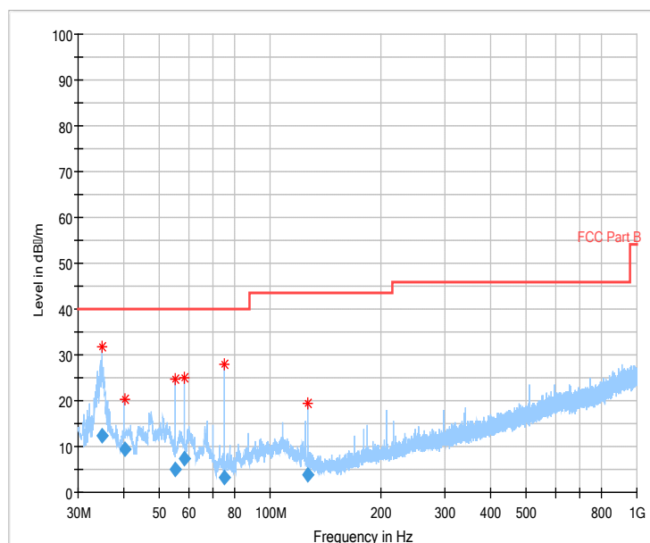
Fig.64 Radiated emission: \pi/4 DQPSK, Ch0, 30MHz~1GHz
