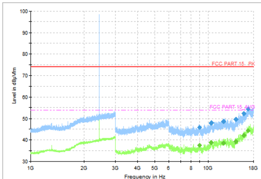
Fig.21 Radiated Spurious Emission (Ch19, 1 GHz - 18 GHz), LE 1M
