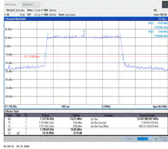
1-N66-PC3-15-15-M-3-DFT-16QAM-Outer_Full-75@ 0-Ant1-13.432-14.160-≤15-PASS
