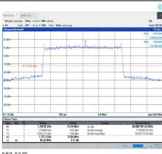
1-N66-PC3-15-40-L-3-DFT-16QAM-Outter_Full-216 @0-Ant1-38.488-40.240-≤40-PASS
