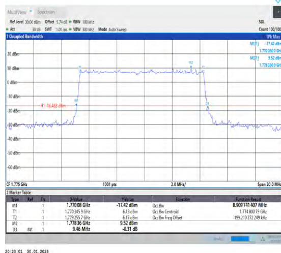
1-N66-PC3-15-10-H-5-DFT-256QAM-Outer_Full-50 @0-Ant1-8.91-9.460-≤10-PASS
