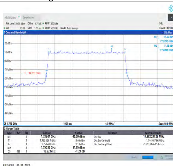
1-N66-PC3-15-20-M-4-DFT-64QAM-Outer_Full-100 @0-Ant1-17.882-18.920-≤20-PASS
