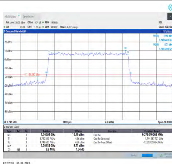
1-N66-PC3-15-10-M-8-CP-64QAM-Outer_Full-52@0 -Ant1-9.276-9.900-≤10-PASS
