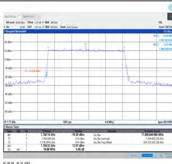
1-N66-PC3-15-20-M-1-DFT-QPSK-Outer_Full-100@ 0-Ant1-17.891-18.880-≤20-PASS
