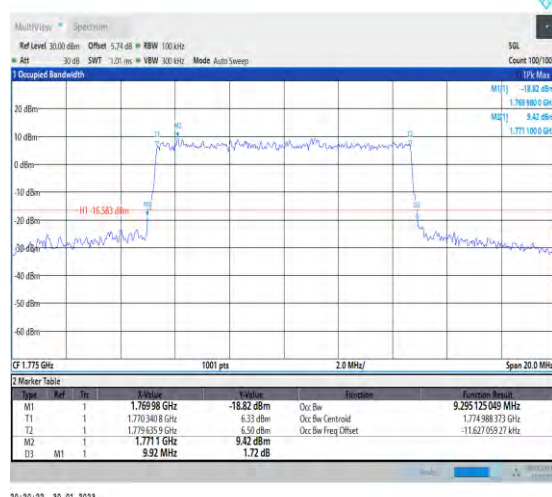
1-N66-PC3-15-10-H-7-CP-16QAM-Outer_Full-52@0 -Ant1-9.295-9.920-≤10-PASS
