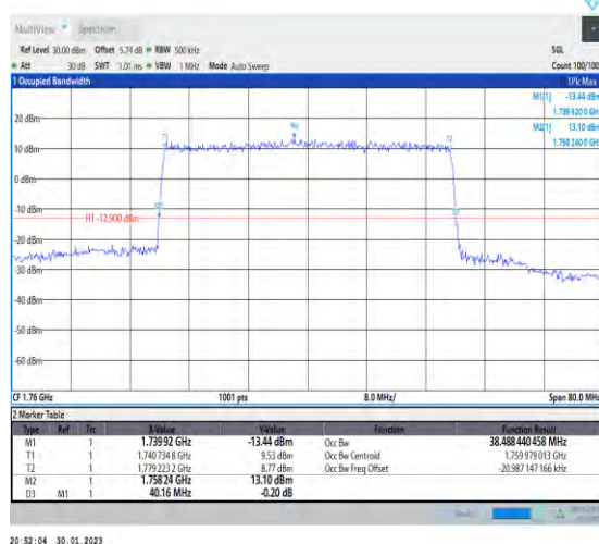
1-N66-PC3-15-40-H-6-CP-QPSK-Outer_Full-216@0 -Ant1-38.488-40.160-≤40-PASS
