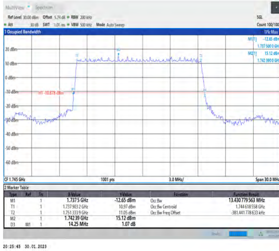
1-N66-PC3-15-15-M-2-DFT-PI2BPSK-Outer_Full-75 @0-Ant1-13.431-14.250-≤15-PASS
