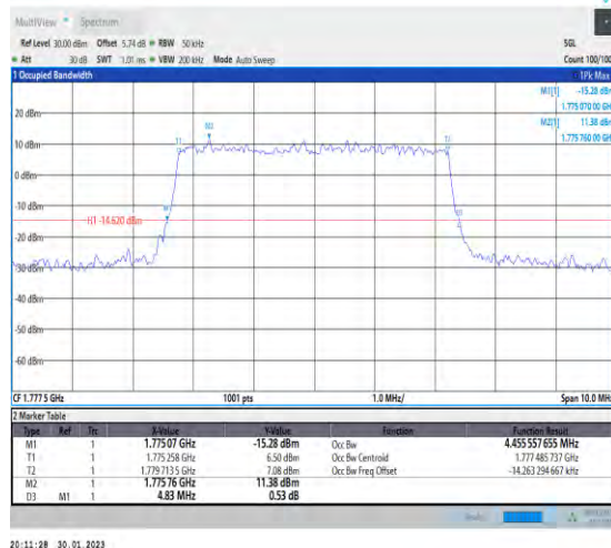
1-N66-PC3-15-5-H-4-DFT-64QAM-Outer_Full-25@0 -Ant1-4.456-4.830-≤5-PASS
