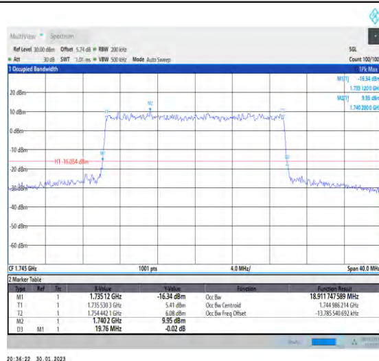
1-N66-PC3-15-20-M-6-CP-QPSK-Outer_Full-106@0-Ant1-18.912-19.760-≤20-PASS
