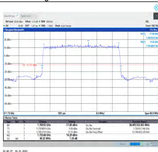
1-N66-PC3-15-40-L-2-DFT-PI2BPSK-Outter_Full-216 @0-Ant1-38.406-40.320-≤40-PASS
