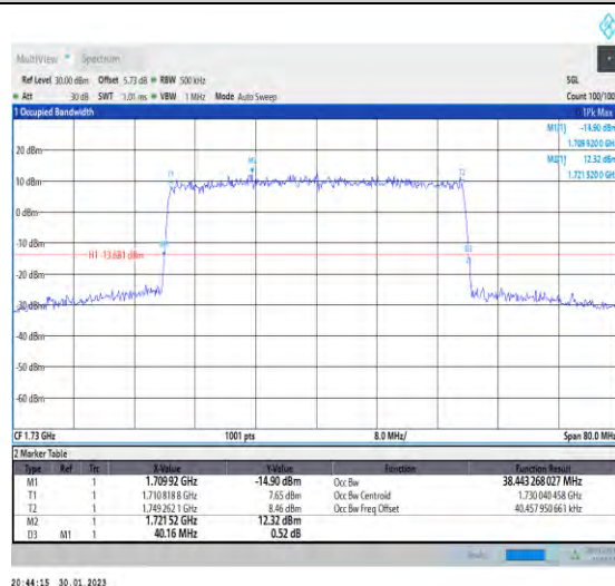
1-N66-PC3-15-40-L-4-DFT-64QAM-Outter_Full-216 @0-Ant1-38.443-40.160-≤40-PASS
