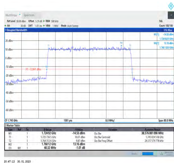
1-N66-PC3-15-40-M-3-DFT-16QAM-Outer_Full-216 @0-Ant1-38.576-40.320-≤40-PASS
