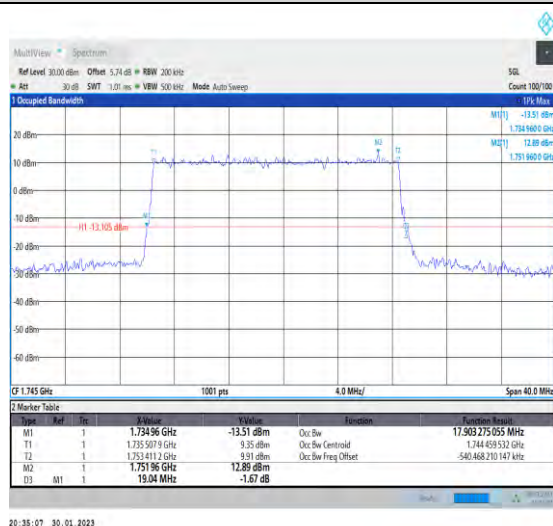
1-N66-PC3-15-20-M-1-DFT-QPSK-Outer_Full-100@ 0-Ant1-17.903-19.040-≤20-PASS
