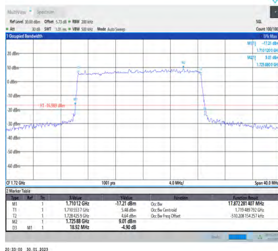
1-N66-PC3-15-20-L-5-DFT-256QAM-Outer_Full-100 @0-Ant1-17.872-18.920-≤20-PASS
