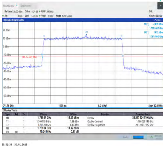
1-N66-PC3-15-40-H-3-DFT-16QAM-Outer_Full-216 @0-Ant1-38.518-40.240-≤40-PASS
