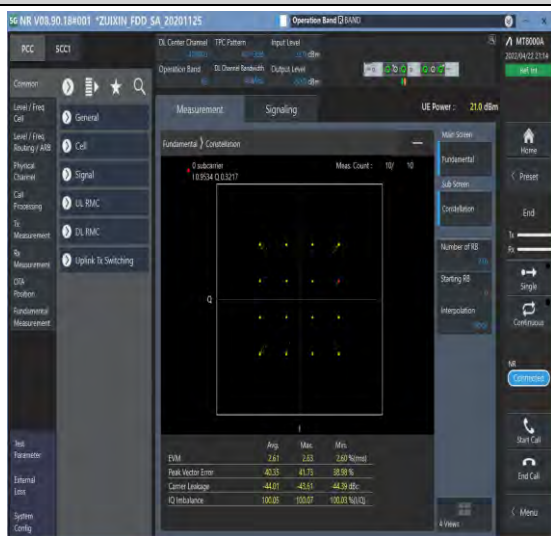
1-N66-PC3-15-40-M-3-DFT-16QAM-Out_Full-216 @0-Ant1-see graph-PASS
