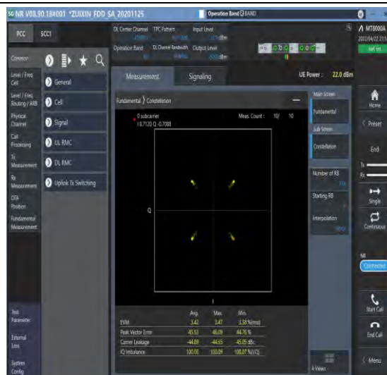
1-N66-PC3-15-40-M-2-DFT-QPSK-Out_Full-216 @0-Ant1-see graph-PASS
