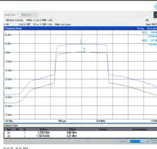
1-N66-PC3-15-40-L-2-CP-256QAM-Outer_Full-216 @0-Ant1-9.62-100%-0.00-9.62-PASS≤13
