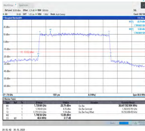
1-N66-PC3-15-40-H-4-DFT-64QAM-Outer_Full-216 @0-Ant1-38.642-40.400-≤40-PASS
