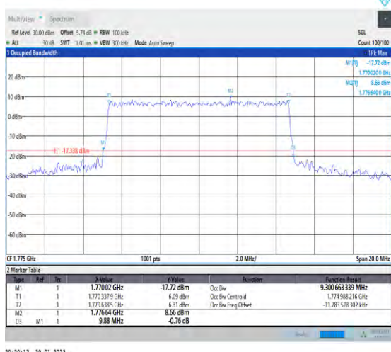
1-N66-PC3-15-10-H-6-CP-QPSK-Outer_Full-52@0- Ant1-9.301-9.880-≤10-PASS
