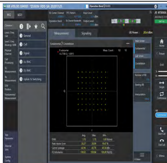
1-N66-PC3-15-40-M-4-DFT-64QAM-Out_Full-216 @0-Ant1-see graph-PASS
