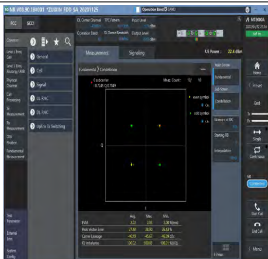
1-N66-PC3-15-40-M-1-DFT-PI2BPSK-Out_Full-216 @0-Ant1-see graph-PASS
