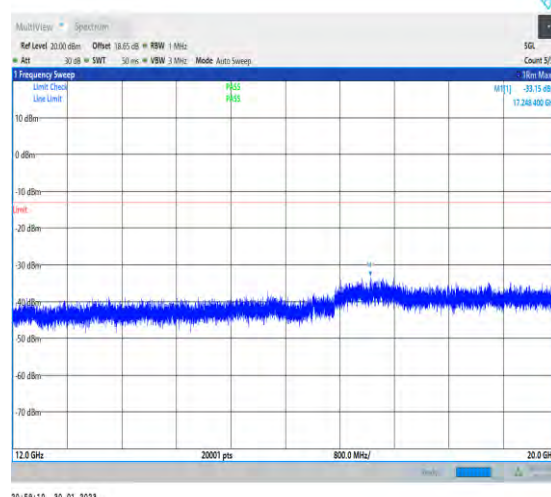
1-N66-PC3-15-40-M-1-DFT-PI2BPSK-Inner_1RB_L ef t-1@1-12000-20000-Ant1-17248.40--33.15--13-PASS
