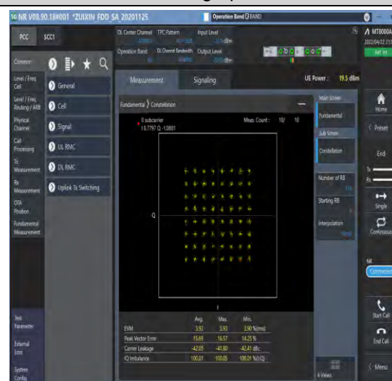
1-N66-PC3-15-40-M-8-CP-64QAM-Outer_Full-216 @0-Ant1-see graph-PASS
