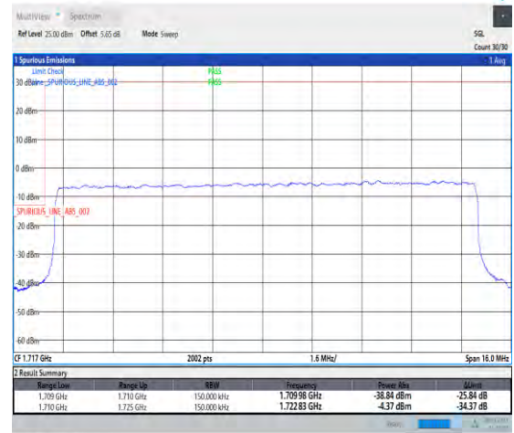
1-N66-PC3-15-15-L-3-DFT-PI2BPSK-Outer_Full-75@0-Ant1-1-seegraph-PASS-see graph
