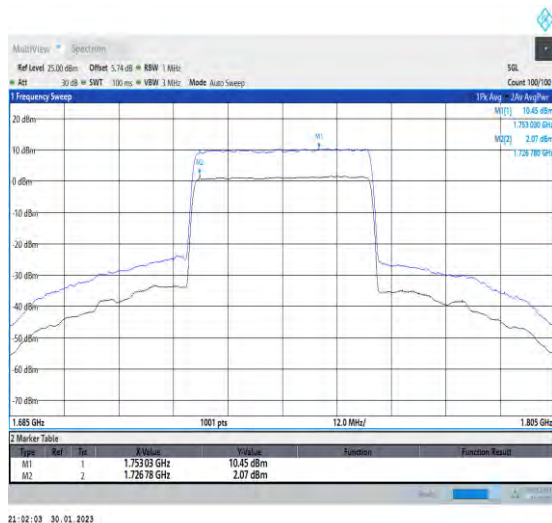
1-N66-PC3-15-40-M-1-DFT-256QAM-Outer_Full-216 @0-Ant1-8.38-100%-0.00-8.38-PASS≤13
