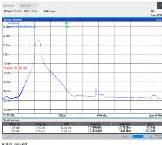
1-N66-PC3-15-5-L-4-CP-QPSK-Edge_1RB_Left-1@0-Ant1-1-seegraph-PASS-see graph
