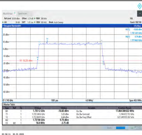
1-N66-PC3-15-20-M-5-DFT-256QAM-Outer_Full-100 @0-Ant1-17.864-18.800-≤20-PASS
