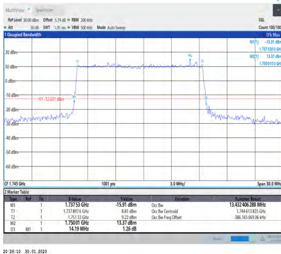
1-N66-PC3-15-15-M-4-DFT-64QAM-Outer_Full-75@ 0-Ant1-13.432-14.190-≤15-PASS
