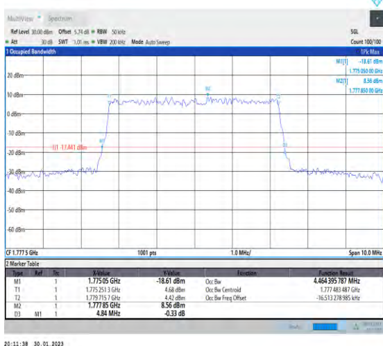
1-N66-PC3-15-5-H-5-DFT-256QAM-Outer_Full-25@0 0-Ant1-4.464-4.840-≤5-PASS
