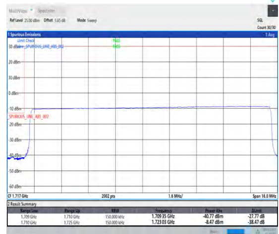
1-N66-PC3-15-15-L-6-CP-QPSK-Outer_Full-79@0-Ant1-1-seegraph-PASS-see graph
