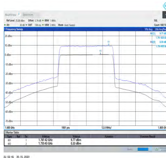
1-N66-PC3-15-40-M-2-CP-256QAM-Outer_Full-216 @0-Ant1-9.44-100%-0.00-9.44-PASS≤13
