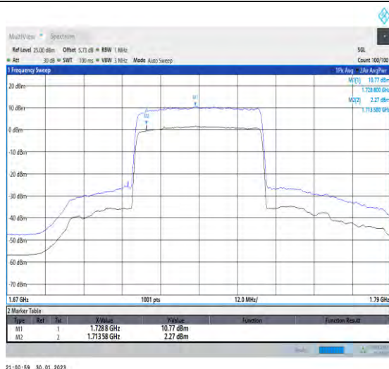
1-N66-PC3-15-40-L-1-DFT-256QAM-Outer_Full-216 @0-Ant1-8.50-100%-0.00-8.50-PASS≤13
