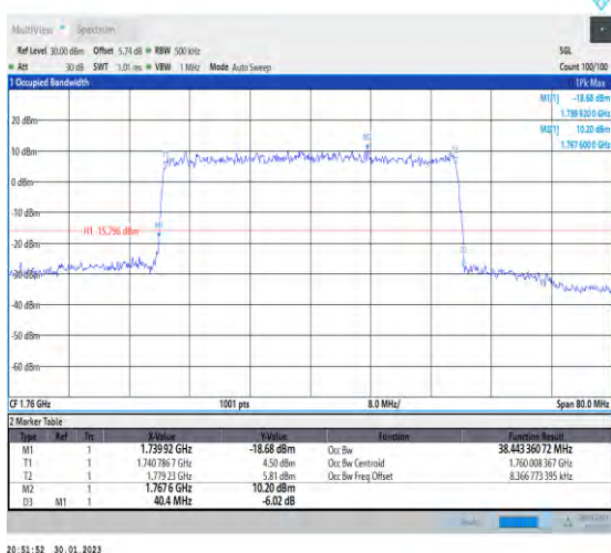
1-N66-PC3-15-40-H-5-DFT-256QAM-Outer_Full-216 @0-Ant1-38.443-40.400-≤40-PASS
