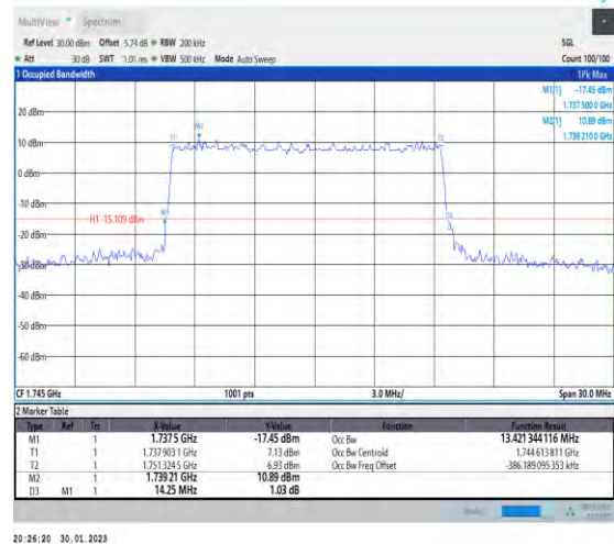
1-N66-PC3-15-15-M-5-DFT-256QAM-Outer_Full-75 @0-Ant1-13.421-14.250-≤15-PASS
