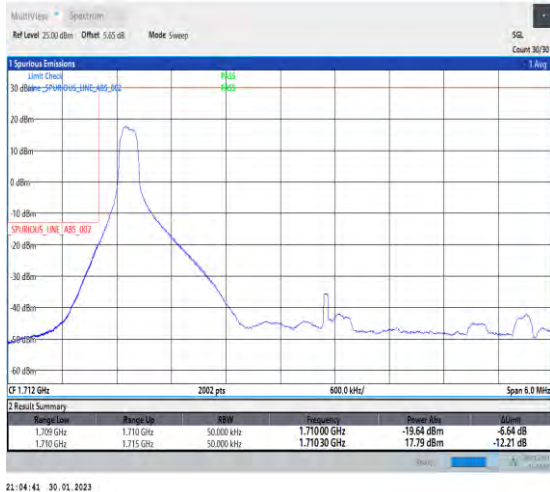
1-N66-PC3-15-5-L-1-DFT-PI2BPSK-Edge_1RB_Left-1 @0-Ant1-1-seegraph-PASS-see graph
