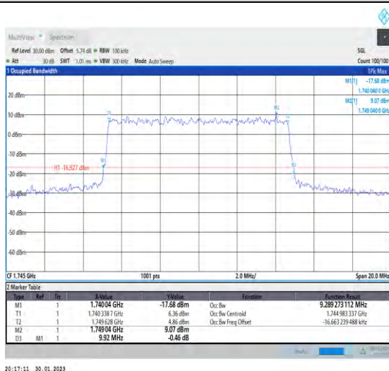
1-N66-PC3-15-10-M-7-CP-16QAM-Outer_Full-52@0 -Ant1-9.289-9.920-≤10-PASS
