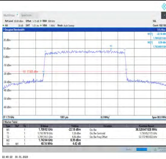
1-N66-PC3-15-40-L-9-CP-256QAM-Outer_Full-216 @0-Ant1-38.529-40.160-≤40-PASS
