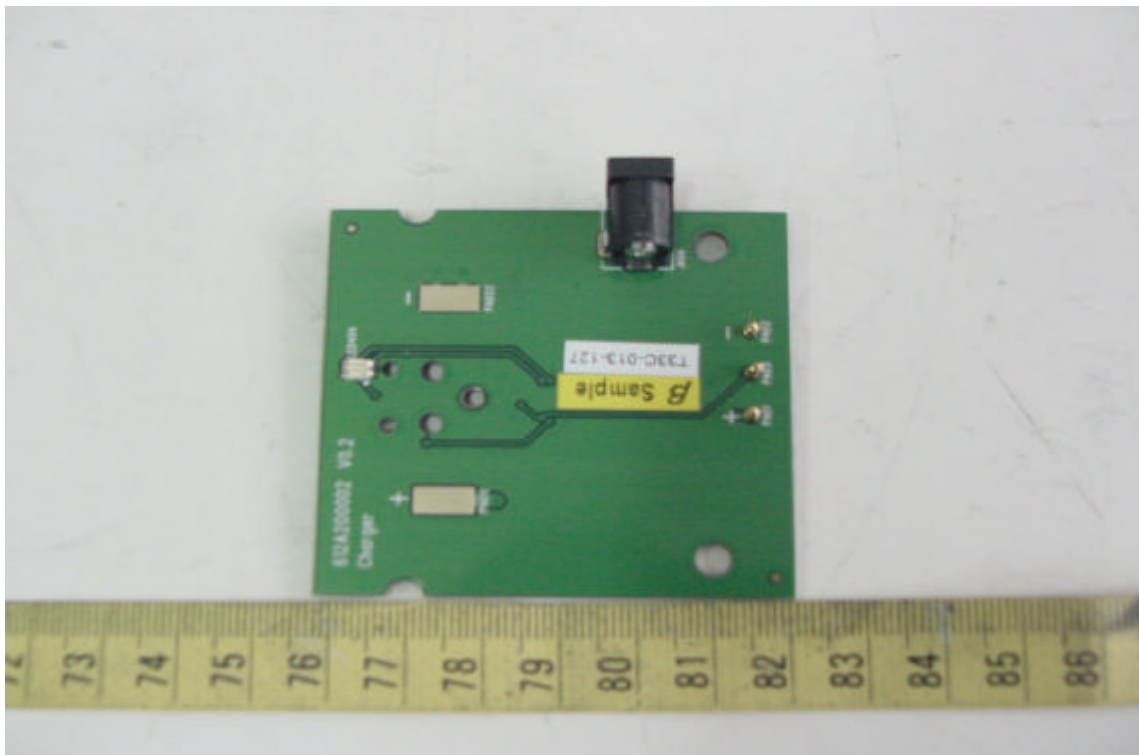
Component View of PCB (Charger)
