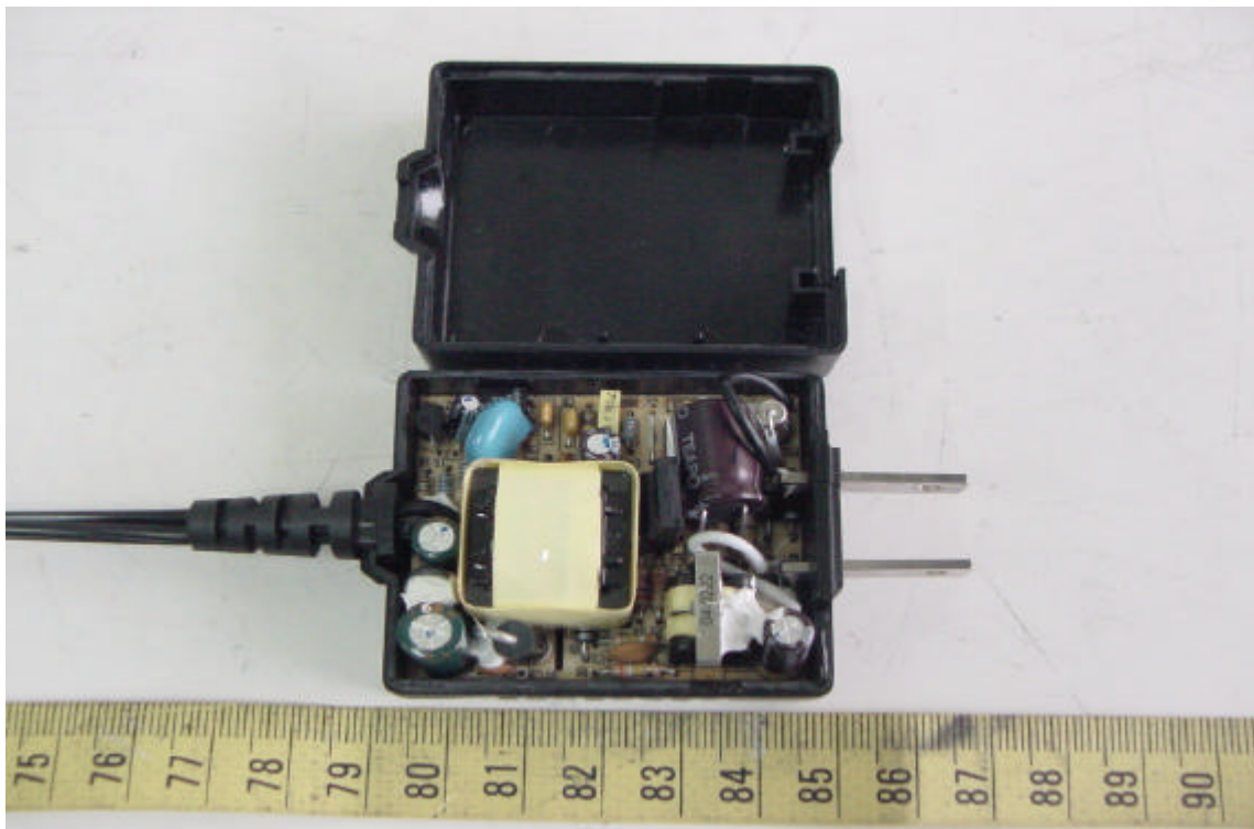
Internal View of Adapter
