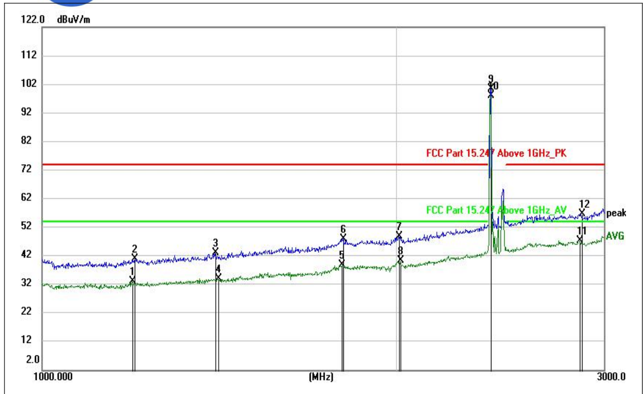
(LE 1M PHY _2405MHz, Antenna Vertical , 1GHz to 3GHz)
