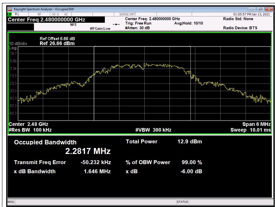
(Channel 26: 2480MHz)
