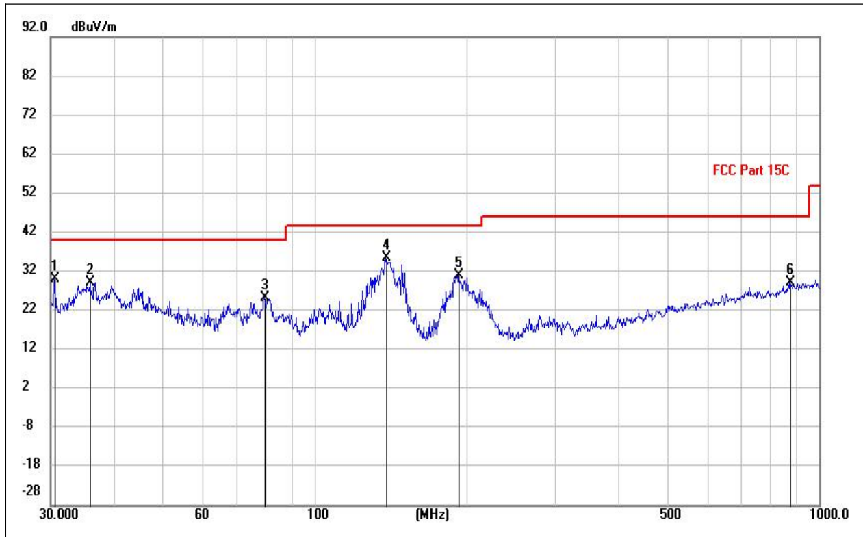
(LE 1M PHY _2480MHz, Antenna Vertical, 30MHz to 1GHz)
