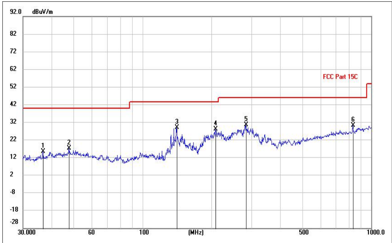
(LE 1M PHY_2405MHz, Antenna Horizontal, 30MHz to 1GHz)
