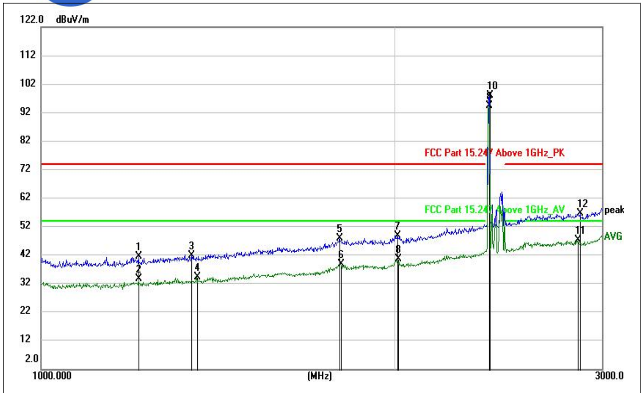
(LE 1M PHY _2405MHz, Antenna Horizontal, 1GHz to 3GHz)
