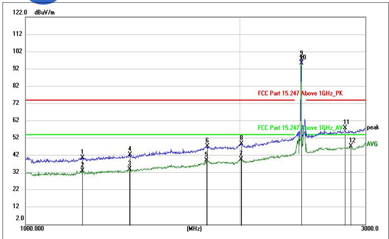
(LE 1M PHY _2440MHz, Antenna Horizontal, 1GHz to 3GHz)
