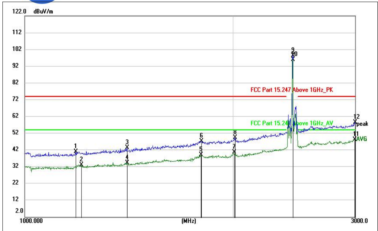
(LE 1M PHY_2440MHz, Antenna Vertical , 1GHz to 3GHz)
