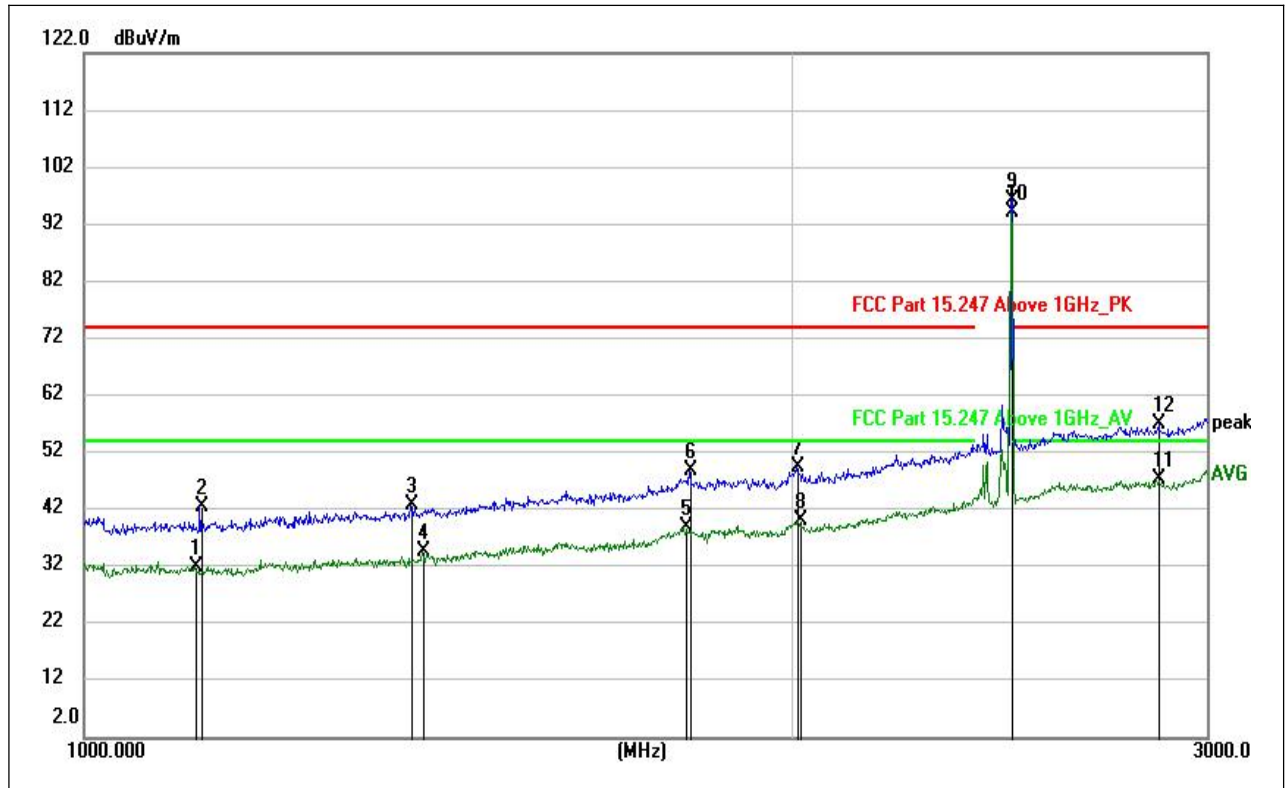
(LE 1M PHY _2480MHz, Antenna Vertical , 1GHz to 3GHz)
