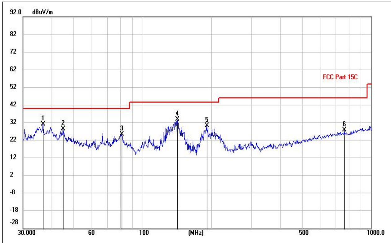
(LE 1M PHY _2440MHz, Antenna Vertical, 30MHz to 1GHz)
