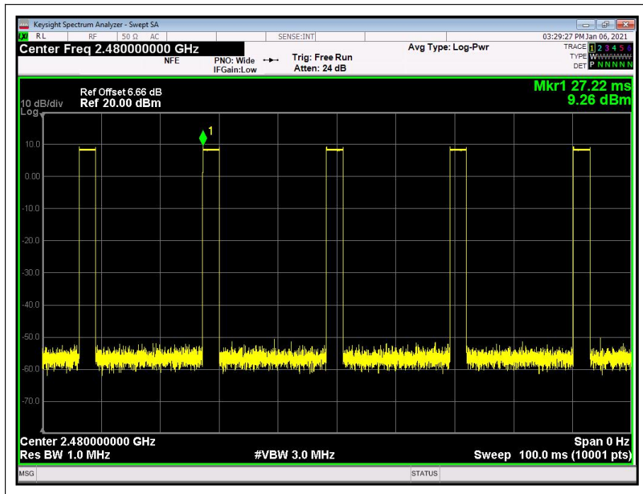
(Channel 39,2480MHz)
