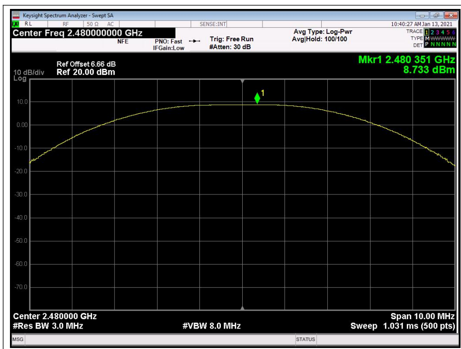
(Channel 26, 2480MHz)
