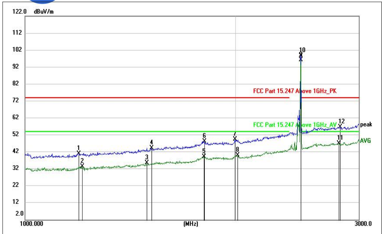
(LE 1M PHY _2480MHz, Antenna Horizontal, 1GHz to 3GHz)
