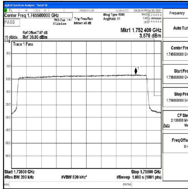
Band4_20MHz_QPSK_20300_100RB#0
