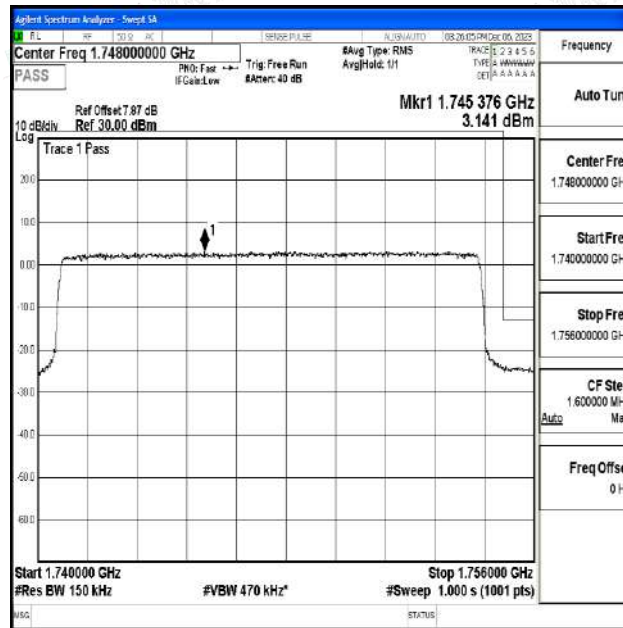
Band4_15MHz_QPSK_20325_75RB#0
