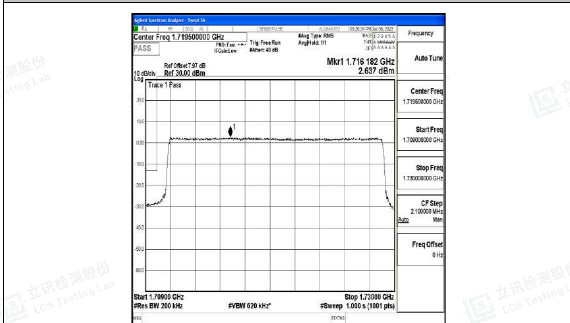
Band4_20MHz_QPSK_20050_100RB#0
