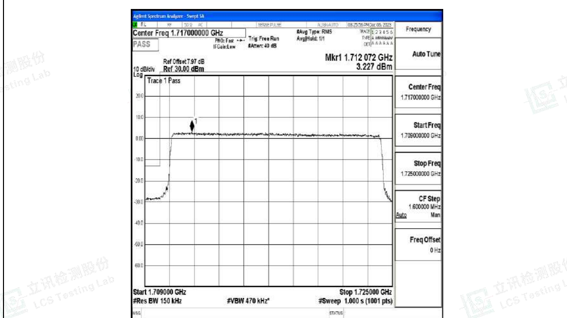
Band4_15MHz_16QAM_20025_75RB#0
