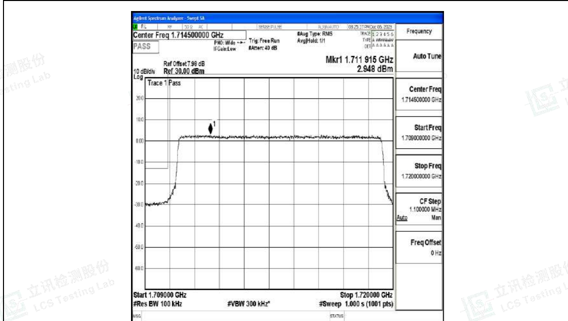
Band4_10MHz_16QAM_20000_50RB#0
