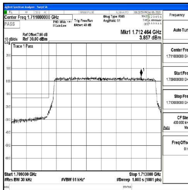
Band4_3MHz_16QAM_19965_15RB#0
