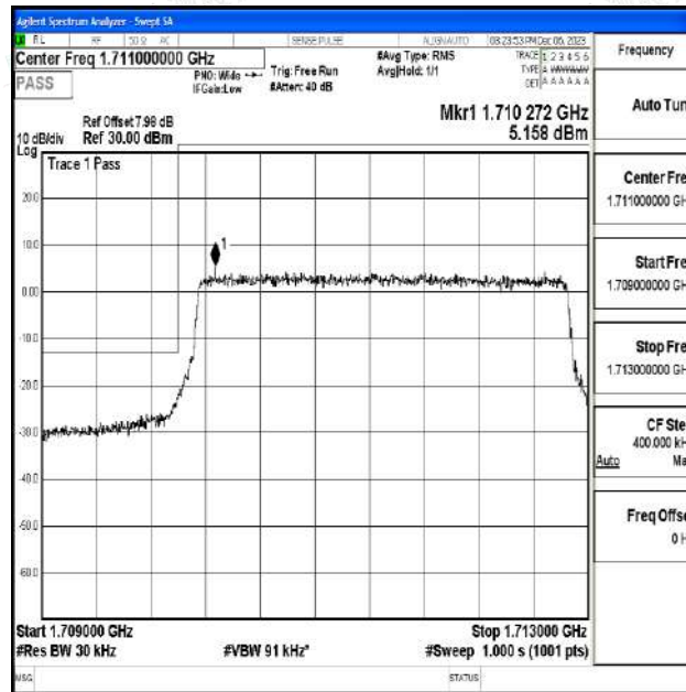
Band4_3MHz_QPSK_19965_15RB#0
