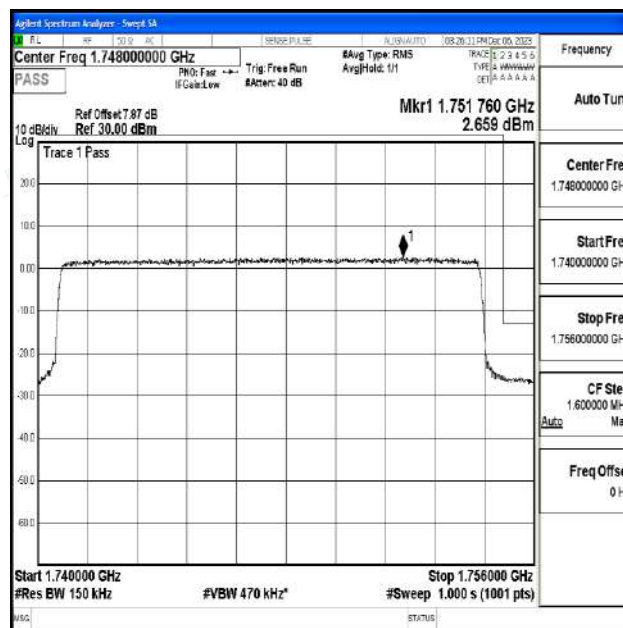
Band4_15MHz_16QAM_20325_75RB#0
