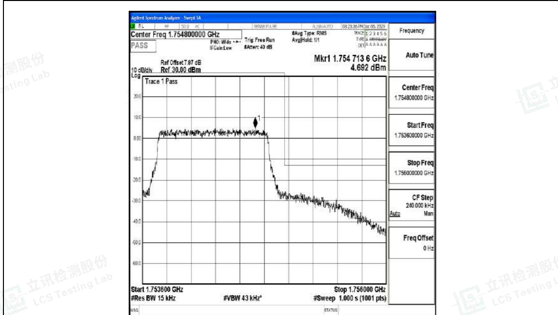
Band4_1.4MHz_16QAM_20393_6RB#0
