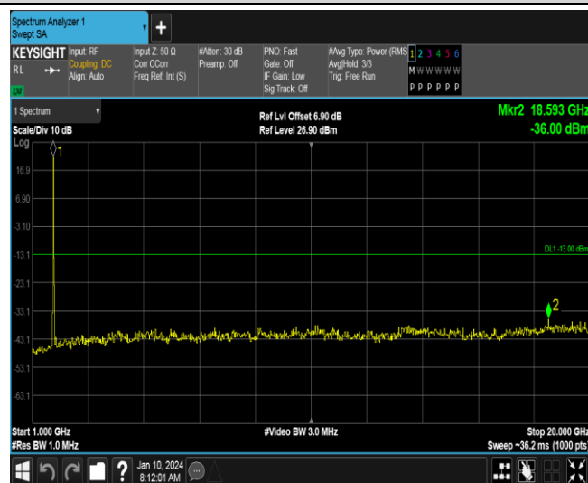
Band4-20MHz-16QAM-20175-1RB#0-Range2:1000~20000MHz
