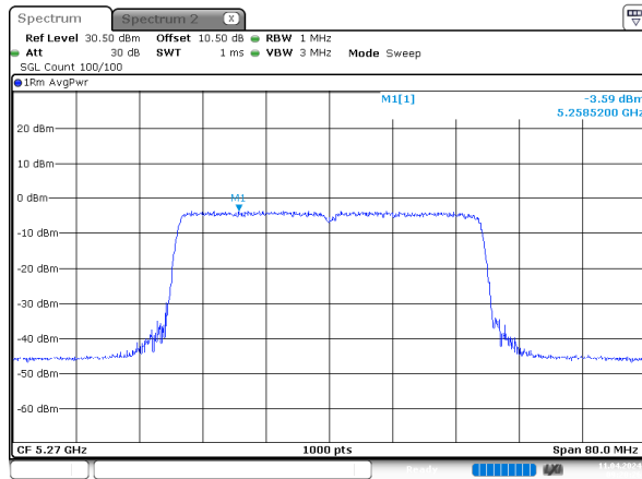
ax40_5270MHz_RU_Full_Chain 0
