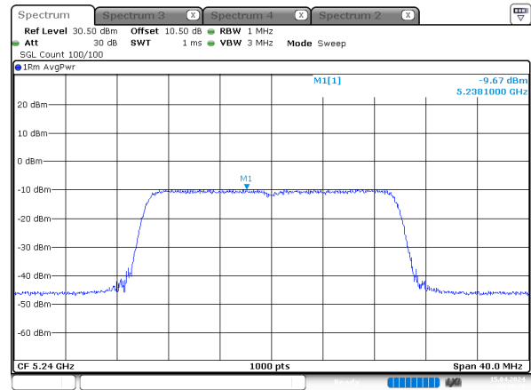
ax20_5240MHz_RU_Full_Chain 1
