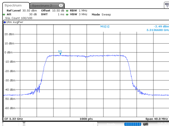
ax20_5320MHz_RU_Full_Chain 0
