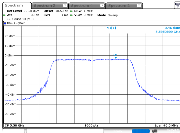
n20_5580MHz_Chain 2
