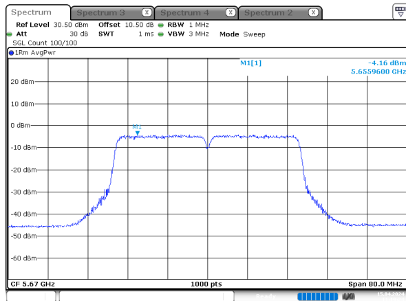
n40_5670MHz_Chain 0
