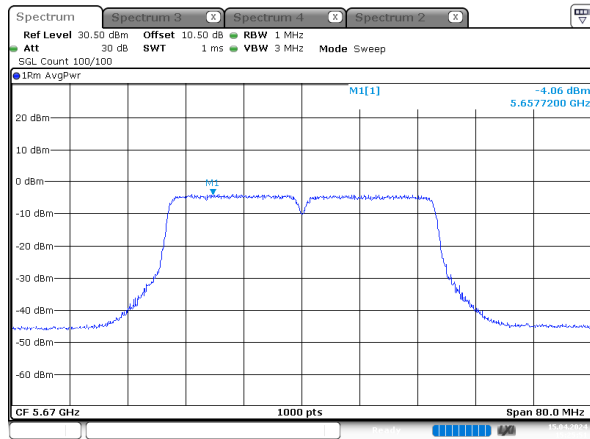
n40_5670MHz_Chain 2
