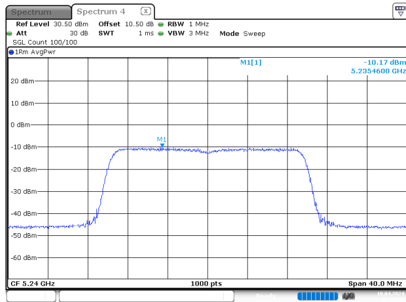
ax20_5240MHz_RU_Full_Chain 0
