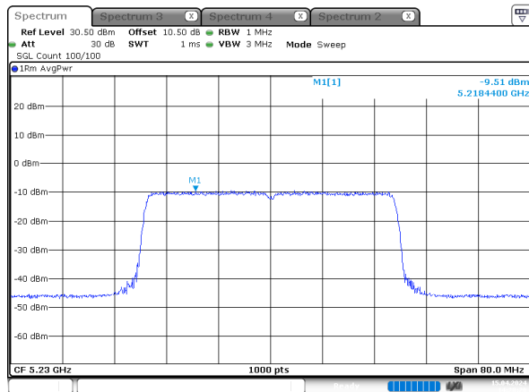
ax40_5230MHz_RU_Full_Chain 2
