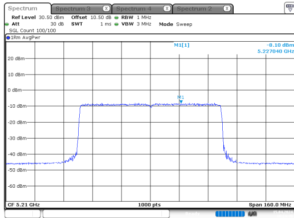
ax80_5210MHz_RU_Full_Chain 0
