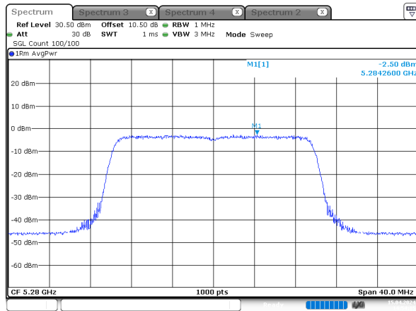
ax20_5280MHz_RU_Full_Chain 2
