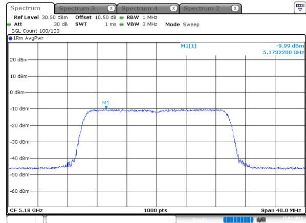
ax20_5180MHz_RU_Full_Chain 1
