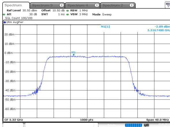
ax20_5320MHz_RU_Full_Chain 2
