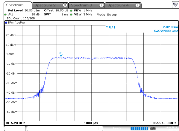
ax20_5280MHz_RU_Full_Chain 3
