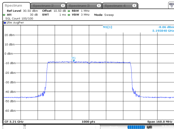
ax80_5210MHz_RU_Full_Chain 2
