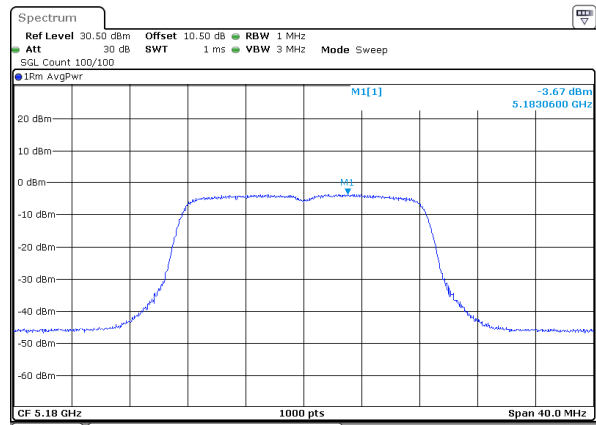
a_5180MHz_Chain 1
