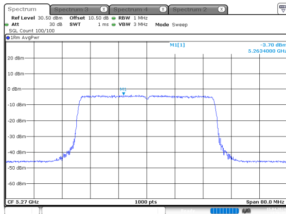
ax40_5270MHz_RU_Full_Chain 2
