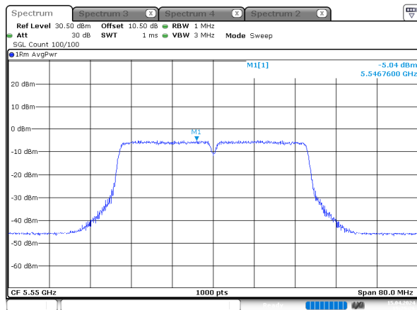
n40_5550MHz_Chain 2
