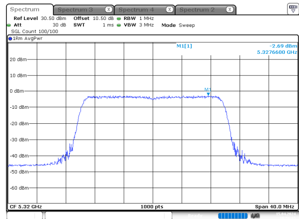
ax20_5320MHz_RU_Full_Chain 1
