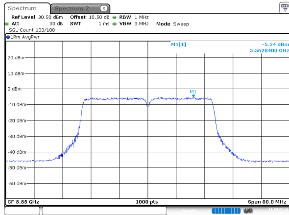
n40_5550MHz_Chain 0
