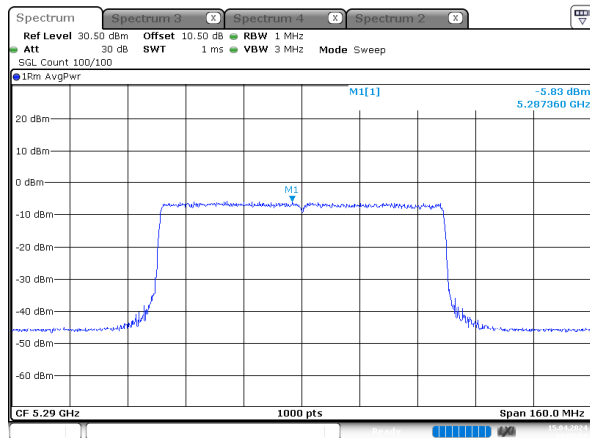
ax80_5290MHz_RU_Full_Chain 2
