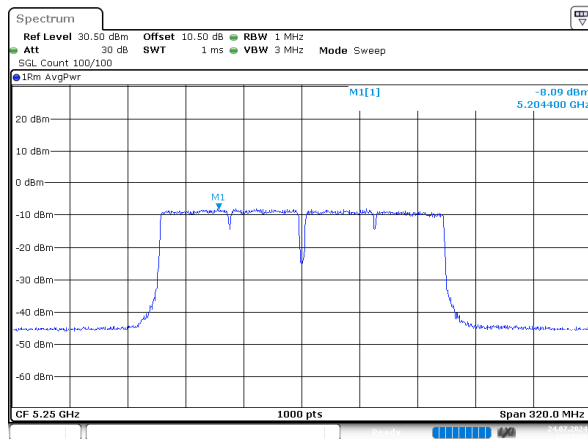
ac160_5250MHz_Chain 2
