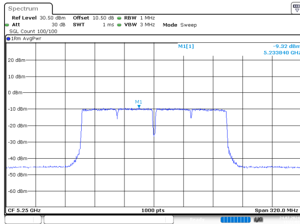
ac160_5250MHz_Chain 0
