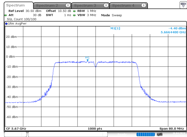
n40_5670MHz_Chain 3
