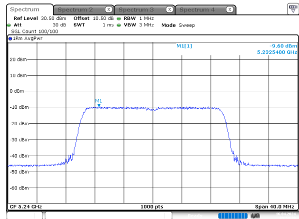
ax20_5240MHz_RU_Full_Chain 3
