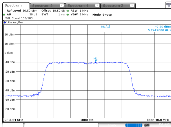
ax20_5240MHz_RU_Full_Chain 2
