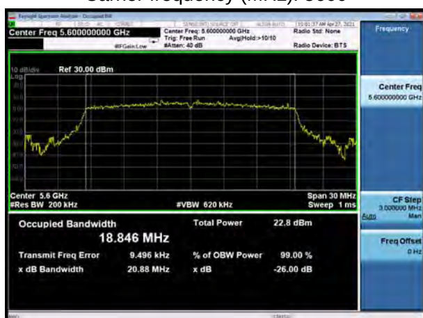
U-NII-2C, 802.11ax HE20 Carrier frequency (MHz): 5600
