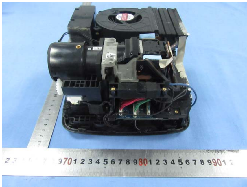
EUT – Uncovered 6 View
