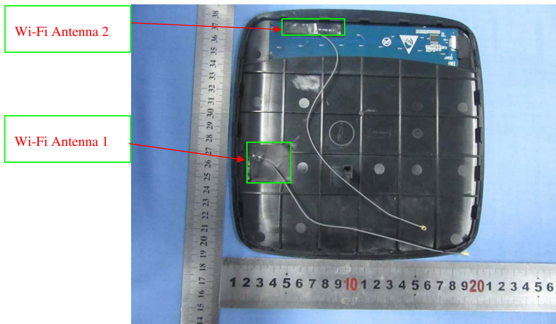
EUT – Wi-Fi Antenna View
