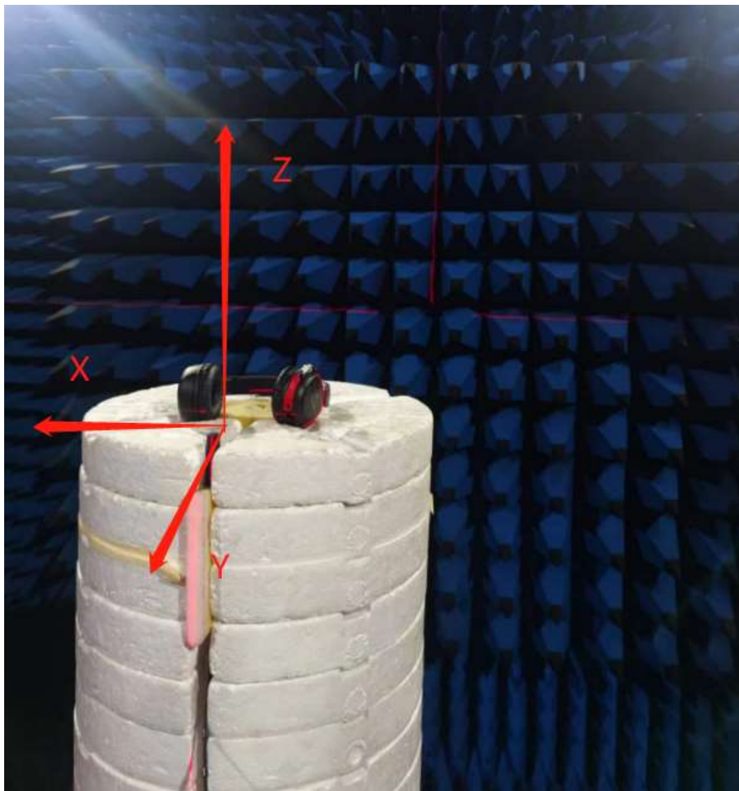
Test setup photos
