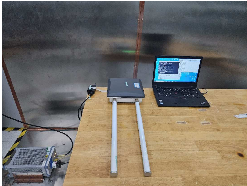
Photograph 1: Set-up for Conducted Emissions, AC Mains
