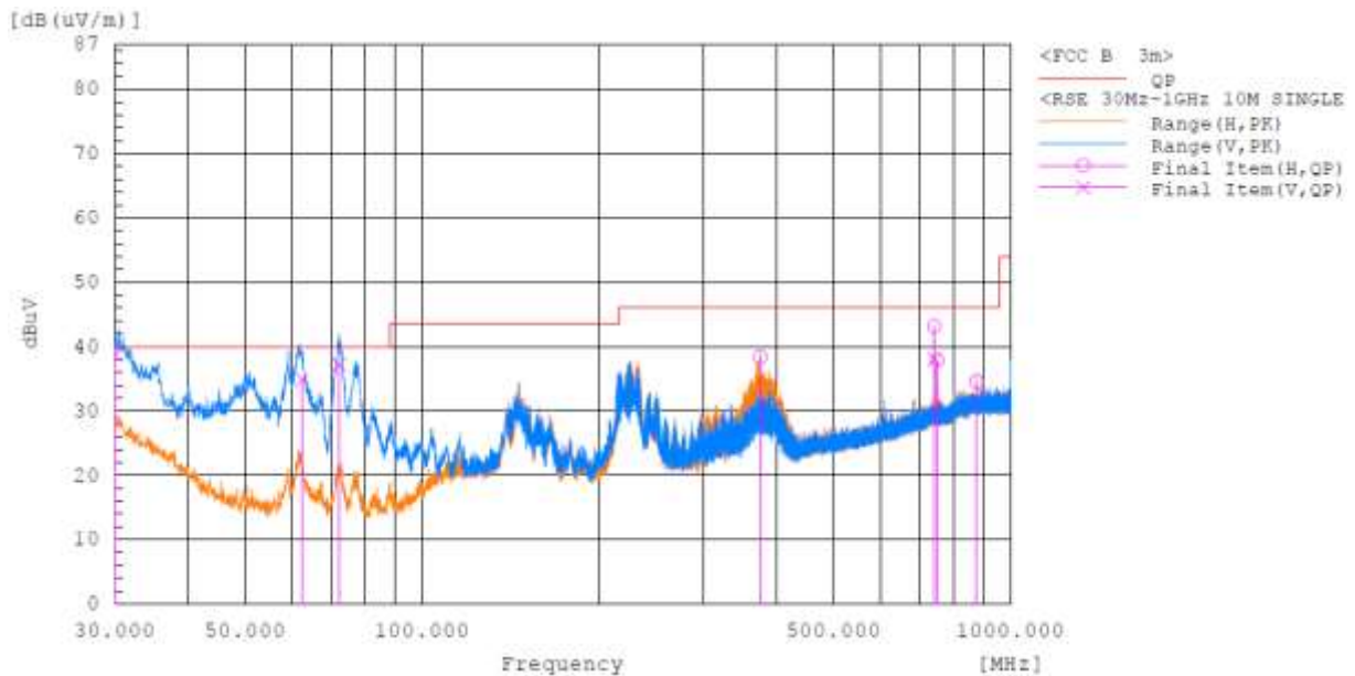
Radiated Spurious Emission 30 MHz – 1 GHz : Contiguous (CH 36+40)
