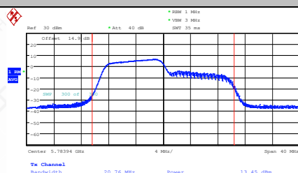
11AX20SISO-Ant1-5785-106Tone-RU53-PASS
