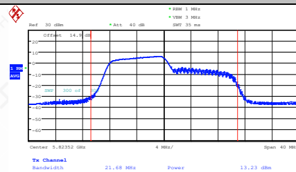
11AX20MIMO-Ant1-5825-106Tone-RU53-PASS
