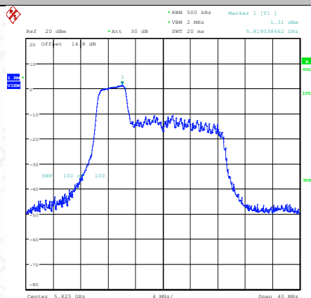
11AX20MIMO-Ant1-5825-52Tone-RU37-PASS
