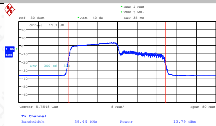
11AX40SISO-Ant2-5755-242Tone-RU61-PASS
