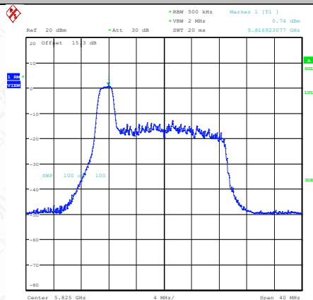
11AX20MIMO-Ant1-5825-26Tone-RU0-PASS
