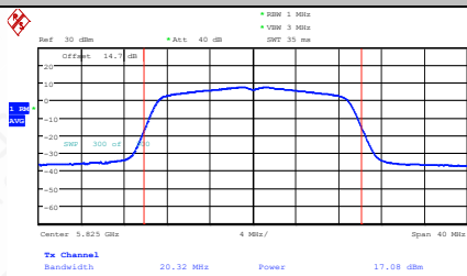
11AC20MIMO-Ant1-5825-PASS
