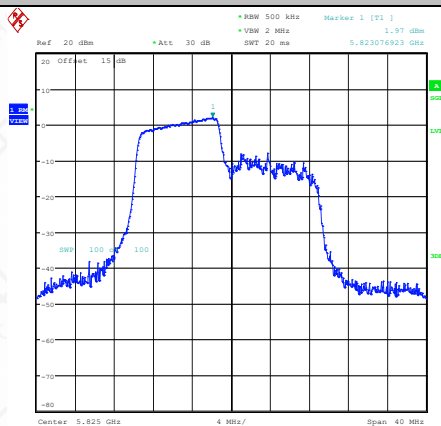
11AX20MIMO-Ant2-5825-106Tone-RU53-PASS
