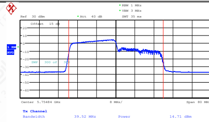
11AX40SISO-Ant1-5755-242Tone-RU61-PASS
