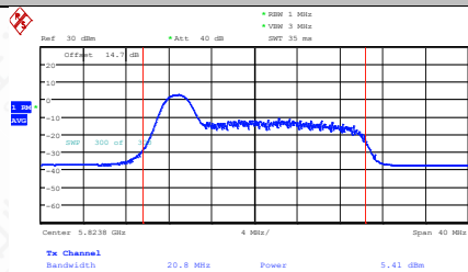
11AX20MIMO-Ant2-5825-26Tone-RU0-PASS
