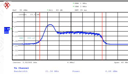
11AX20MIMO-Ant1-5825-26Tone-RU0-PASS
