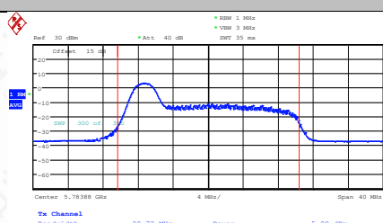
11AX20SISO-Ant2-5785-26Tone-RU0-PASS
