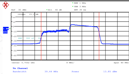
11AX40SISO-Ant2-5755-242Tone-RU62-PASS
