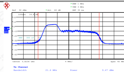
11AX20MIMO-Ant1-5825-52Tone-RU37-PASS
