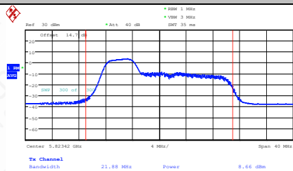
11AX20MIMO-Ant2-5825-52Tone-RU37-PASS
