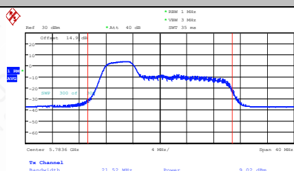
11AX20SISO-Ant2-5785-52Tone-RU37-PASS
