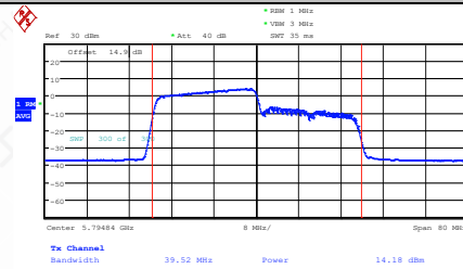
11AX40SISO-Ant1-5795-242Tone-RU61-PASS
