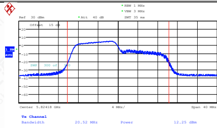
11AX20MIMO-Ant2-5825-106Tone-RU53-PASS
