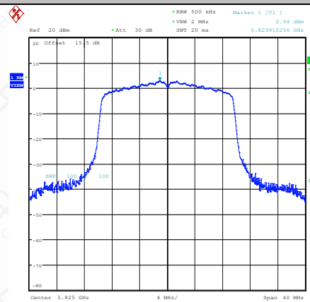
11AX20MIMO-Ant2-5825-PASS
