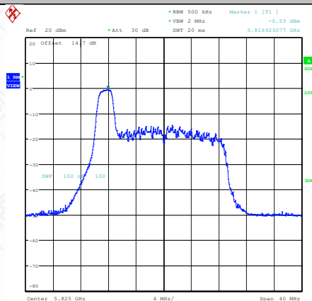
11AX20MIMO-Ant2-5825-26Tone-RU0-PASS
