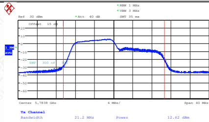
11AX20MIMO-Ant2-5785-106Tone-RU53-PASS
