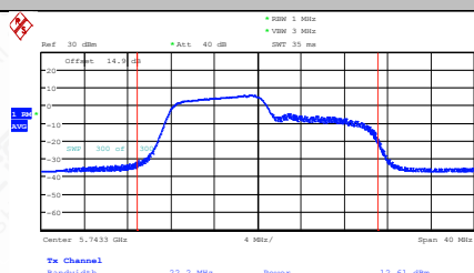
11AX20SISO-Ant2-5745-106Tone-RU53-PASS
