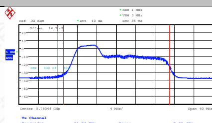
11AX20SISO-Ant1-5785-52Tone-RU37-PASS
