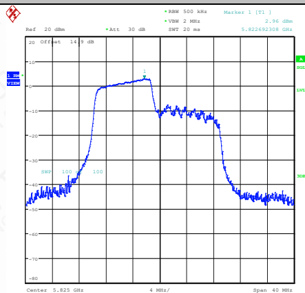
11AX20MIMO-Ant1-5825-106Tone-RU53-PASS
