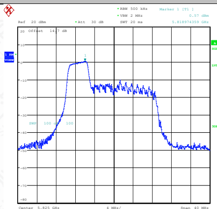
11AX20MIMO-Ant2-5825-52Tone-RU37-PASS
