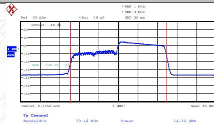
11AX40SISO-Ant1-5755-242Tone-RU62-PASS
