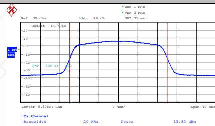
11AC20MIMO-Ant2-5825-PASS
