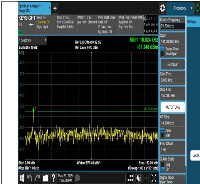
Band7_15MHz_QPSK_20825_1RB#0_0.009~0.15_0.009~0.15
