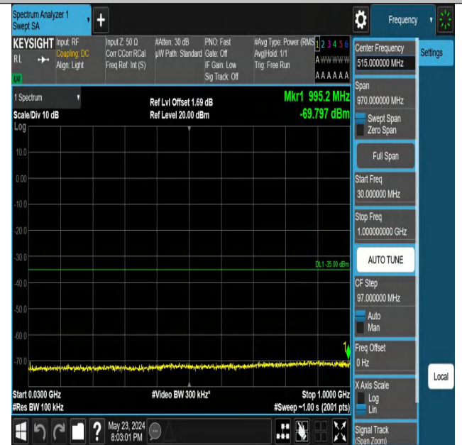
Band7_20MHz_QPSK_21100_1RB#99_30~1000_30~1000
