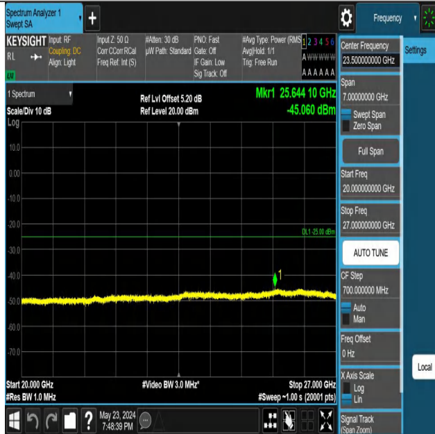
Band7_10MHz_QPSK_21400_1RB#0_20000~27000_20000~270
