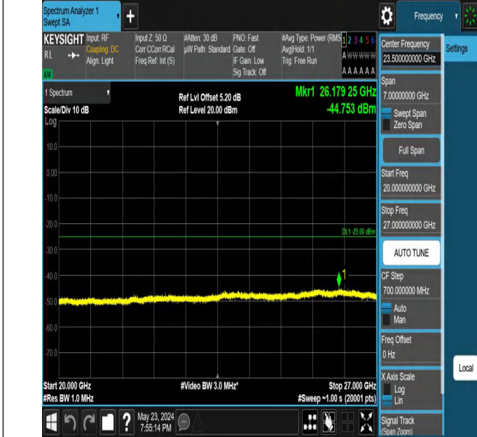
Band7_15MHz_QPSK_21100_1RB#0_20000~27000_20000~270
