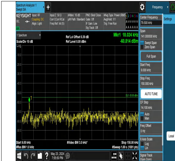
Band7_15MHz_QPSK_21375_1RB#0_0.009~0.15_0.009~0.15
