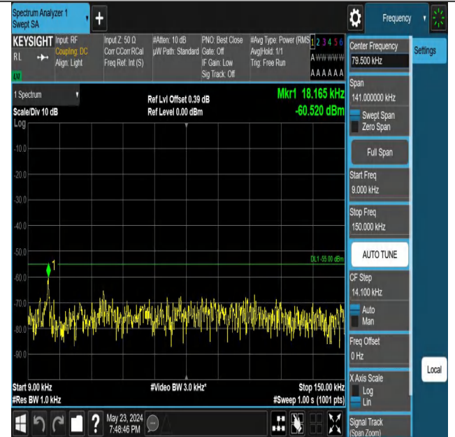
Band7_10MHz_QPSK_21400_1RB#49_0.009~0.15_0.009~0.15
