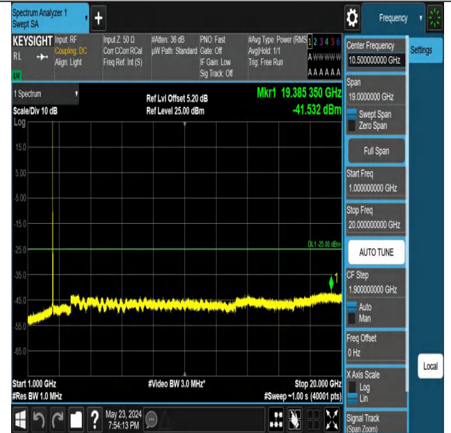
Band7_15MHz_QPSK_20825_1RB#0_1000~20000_1000~20000
