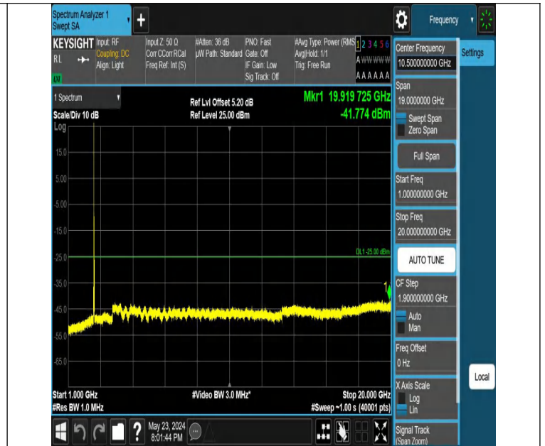
Band7_20MHz_QPSK_20850_1RB#0_1000~20000_1000~20000
