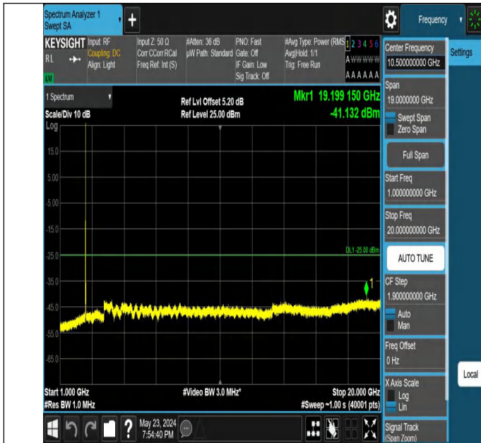
Band7_15MHz_QPSK_20825_1RB#74_1000~20000_1000~2000
