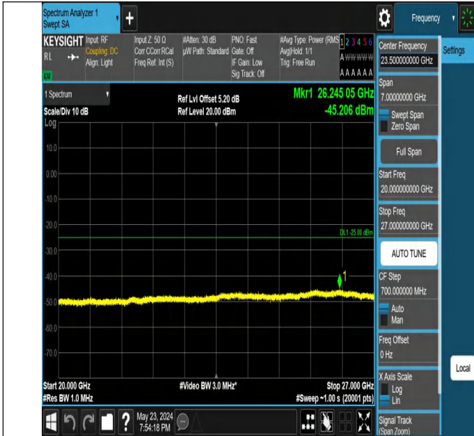
Band7_15MHz_QPSK_20825_1RB#0_20000~27000_20000~27000
