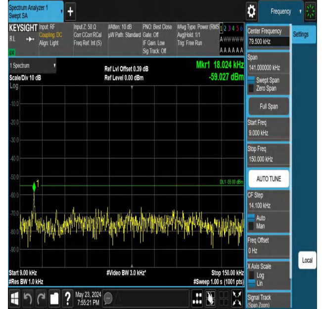
Band7_15MHz_QPSK_21100_1RB#74_0.009~0.15_0.009~0.15
