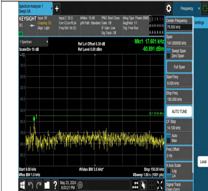
Band7_20MHz_QPSK_21350_1RB#0_0.009~0.15_0.009~0.15
