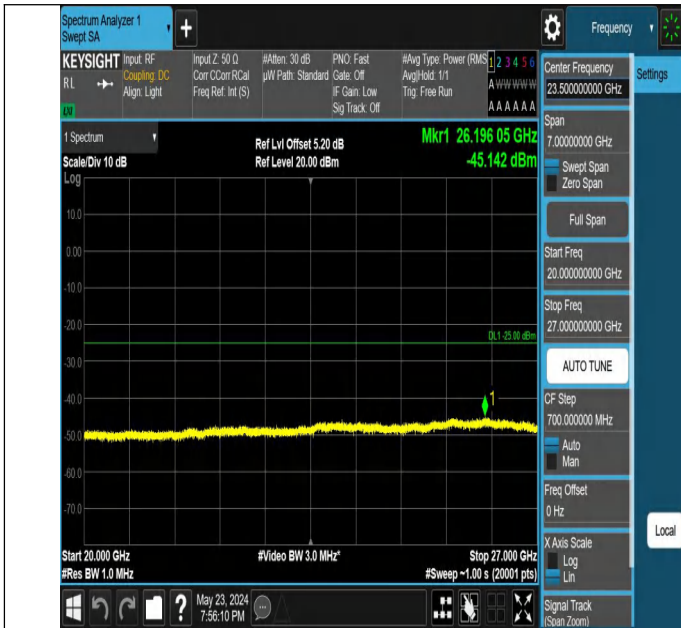
Band7_15MHz_QPSK_21375_1RB#0_20000~27000_20000~27000
