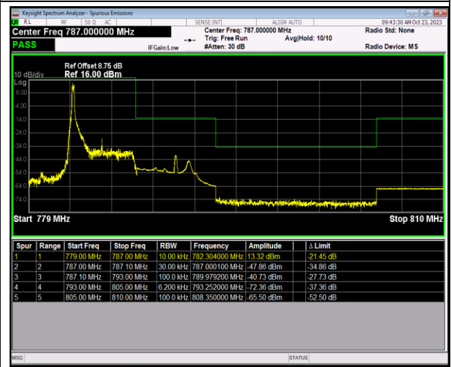
Band13-5MHz-64QAM-23255-25RB#0
