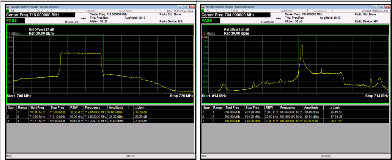
Band17-5MHz-16QAM-23755-1RB#24
