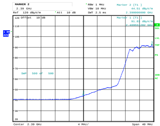
Lower Band Edge, 2412 MHz, 802.11n MIMO, Average
