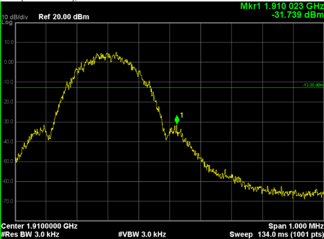
GSM1900 (EDGE 8 Link), Channel 810
