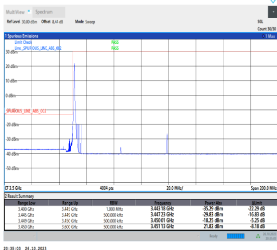
1-N78-3450-3550-PC2-30-70-L-1-DFT-PI2BPSK-Edge_1RB_Left-1@0-Ant0-1--PASS-see graph
