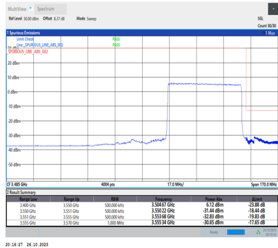
1-N78-3450-3550-PC2-30-50-H-3-DFT-PI2BPSK-Outer_Full-128@0-Ant0-1--PASS-see graph
