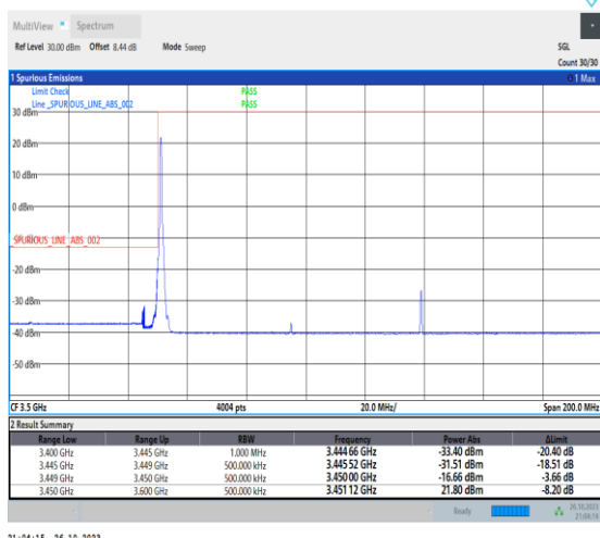
1-N78-3450-3550-PC2-30-90-L-1-DFT-PI2BPSK-Edge_1RB_Left-1@0-Ant0-1--PASS-see graph
