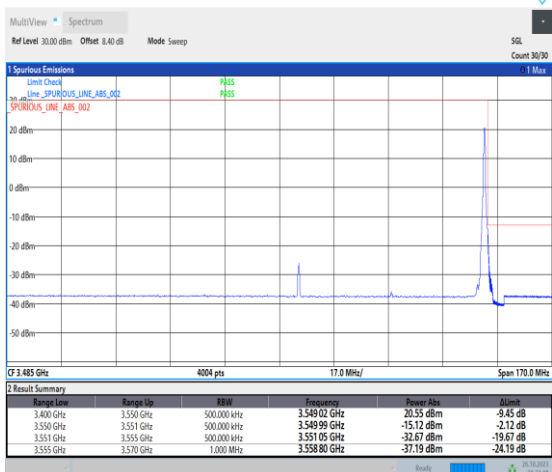
1-N78-3450-3550-PC2-30-60-H-5-CP-QPSK-Edge_1RB_Right-1@161-Ant0-1--PASS-see graph
