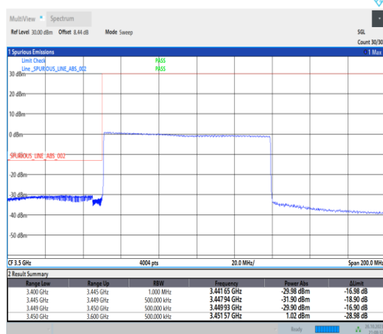
1-N78-3450-3550-PC2-30-90-L-6-CP-QPSK-Outer_Full-245@0-Ant0-1--PASS-see graph
