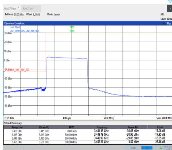
1-N78-3450-3550-PC2-30-50-L-6-CP-QPSK-Outer_Full-133@0-Ant0-1--PASS-see graph
