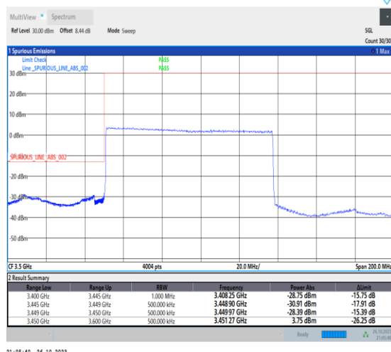
1-N78-3450-3550-PC2-30-90-L-3-DFT-PI2BPSK-Outer_Full-240@0-Ant0-1--PASS-see graph
