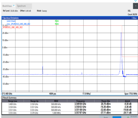
1-N78-3450-3550-PC2-30-100-H-5-CP-QPSK-Edge_1RB_Right-1@272-Ant0-1--PASS-see graph
