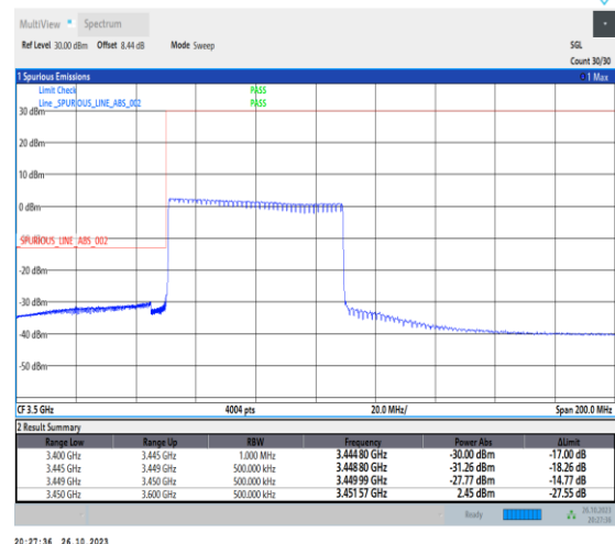
1-N78-3450-3550-PC2-30-60-L-6-CP-QPSK-Outer_Full-162@0-Ant0-1--PASS-see graph
