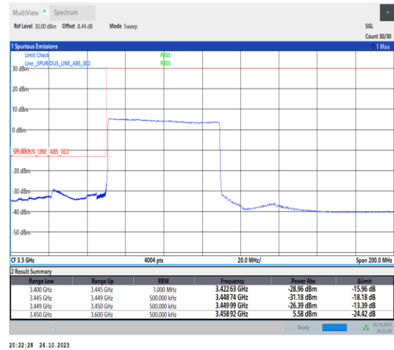
1-N78-3450-3550-PC2-30-60-L-3-DFT-PI2BPSK-Outer_Full-162@0-Ant0-1--PASS-see graph
