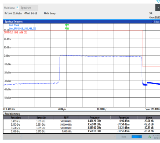
1-N78-3450-3550-PC2-30-90-H-6-CP-QPSK-Outer_Full-245@0-Ant0-1--PASS-see graph
