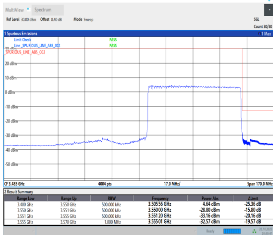
1-N78-3450-3550-PC2-30-60-H-3-DFT-PI2BPSK-Outer_Full-162@0-Ant0-1--PASS-see graph
