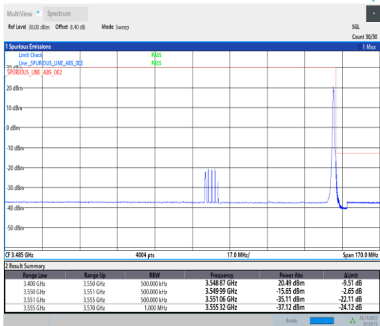
1-N78-3450-3550-PC2-30-60-H-2-DFT-PI2BPSK-Edge_1RB_Right-1@161-Ant0-1--PASS-see graph
