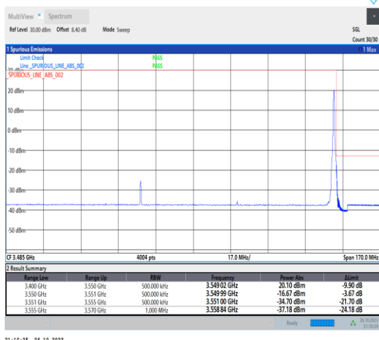
1-N78-3450-3550-PC2-30-90-H-2-DFT-PI2BPSK-Edge_1RB_Right-1@244-Ant0-1--PASS-see graph
