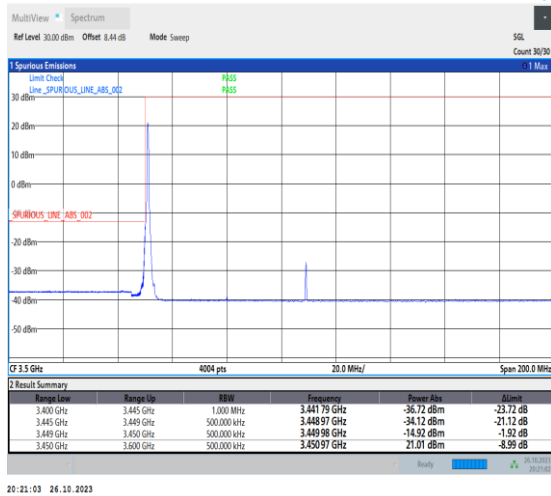
1-N78-3450-3550-PC2-30-60-L-1-DFT-PI2BPSK-Edge_1RB_Left-1@0-Ant0-1--PASS-see graph
