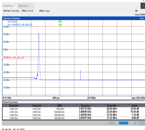
1-N78-3450-3550-PC2-30-60-L-4-CP-QPSK-Edge_1RB_Left-1@0-Ant0-1--PASS-see graph
