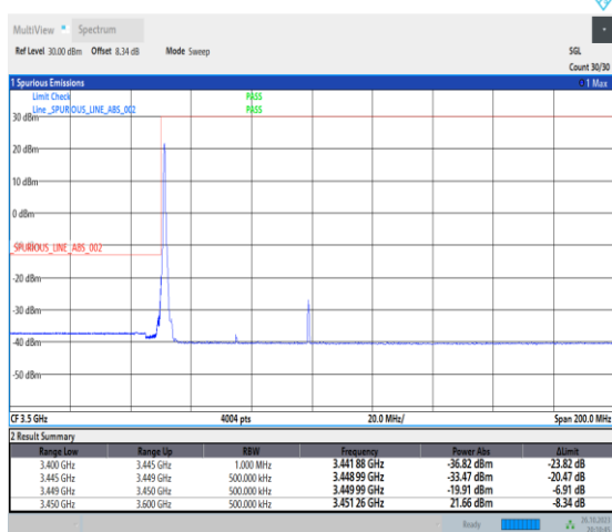
1-N78-3450-3550-PC2-30-50-L-4-CP-QPSK-Edge_1RB_Left-1@0-Ant0-1--PASS-see graph
