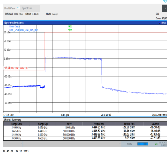
1-N78-3450-3550-PC2-30-70-L-6-CP-QPSK-Outer_Full-189@0-Ant0-1--PASS-see graph
