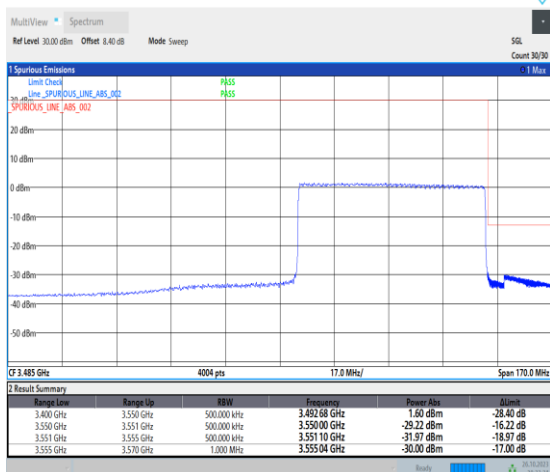
1-N78-3450-3550-PC2-30-60-H-6-CP-QPSK-Outer_Full-162@0-Ant0-1--PASS-see graph
