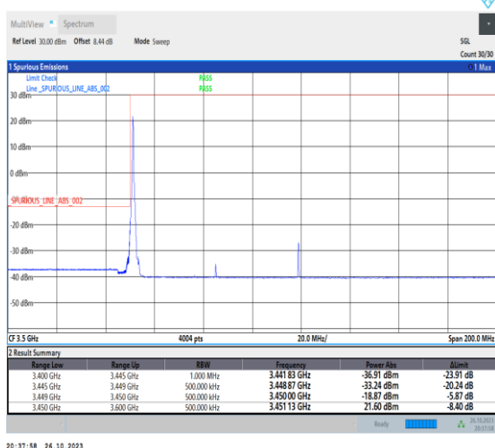
1-N78-3450-3550-PC2-30-70-L-4-CP-QPSK-Edge_1RB_Left-1@0-Ant0-1--PASS-see graph
