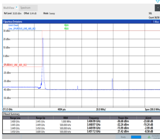
1-N78-3450-3550-PC2-30-90-L-4-CP-QPSK-Edge_1RB_Left-1@0-Ant0-1--PASS-see graph
