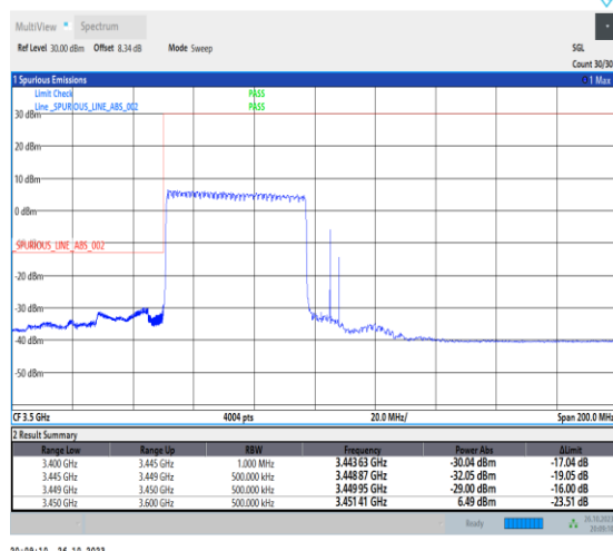
1-N78-3450-3550-PC2-30-50-L-3-DFT-PI2BPSK-Outer_Full-128@0-Ant0-1--PASS-see graph
