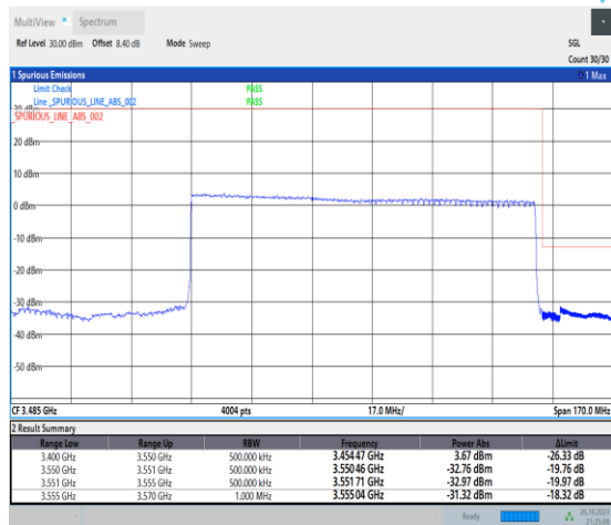
1-N78-3450-3550-PC2-30-100-H-3-DFT-PI2BPSK-Outer_Full-270@0-Ant0-1--PASS-see graph
