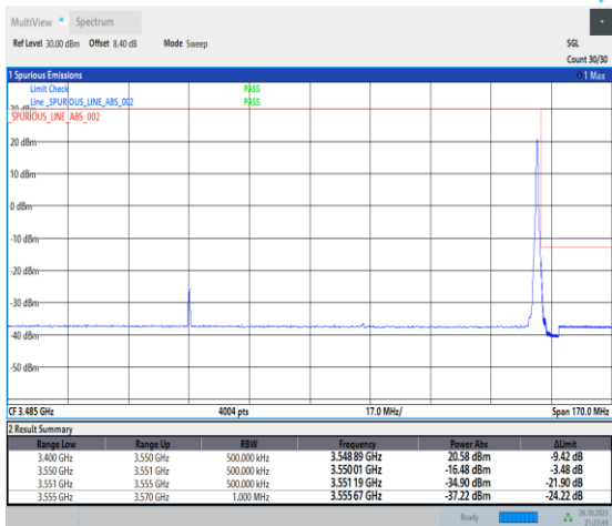
1-N78-3450-3550-PC2-30-100-H-2-DFT-PI2BPSK-Edge_1RB_Right-1@272-Ant0-1--PASS-see graph
