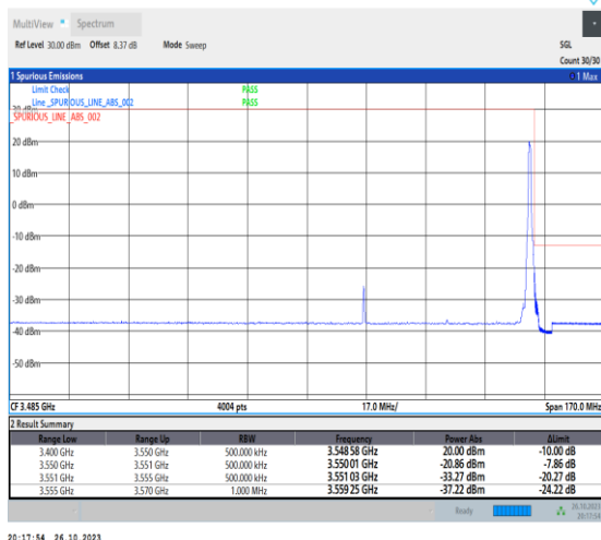
1-N78-3450-3550-PC2-30-50-H-5-CP-QPSK-Edge_1RB_Right-1@132-Ant0-1--PASS-see graph
