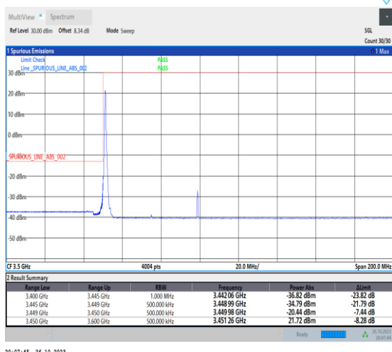
1-N78-3450-3550-PC2-30-50-L-1-DFT-PI2BPSK-Edge_1RB_Left-1@0-Ant0-1--PASS-see graph
