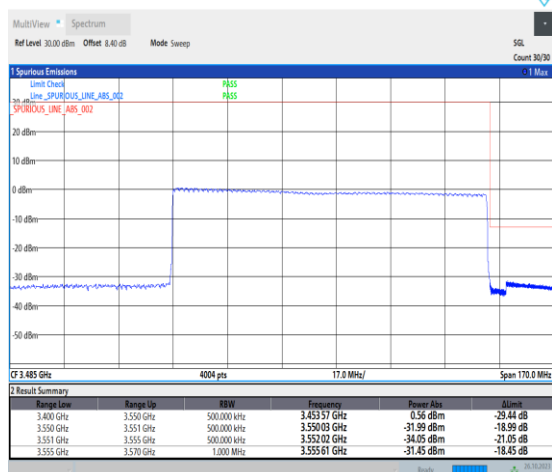
1-N78-3450-3550-PC2-30-100-H-6-CP-QPSK-Outer_Full-273@0-Ant0-1--PASS-see graph
