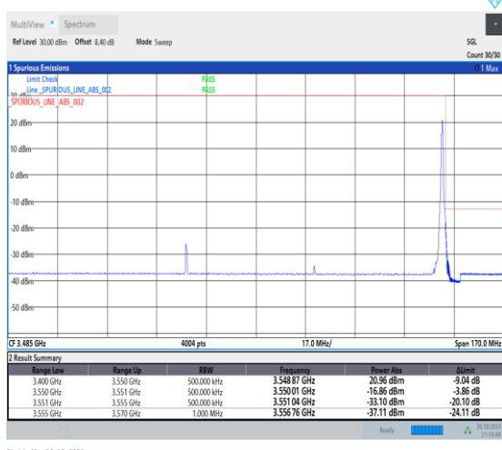
1-N78-3450-3550-PC2-30-90-H-5-CP-QPSK-Edge_1RB_Right-1@244-Ant0-1--PASS-see graph
