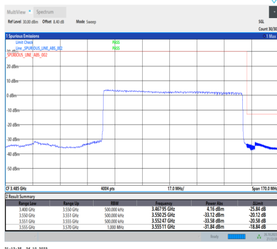
1-N78-3450-3550-PC2-30-90-H-3-DFT-PI2BPSK-Outer_Full-240@0-Ant0-1--PASS-see graph
