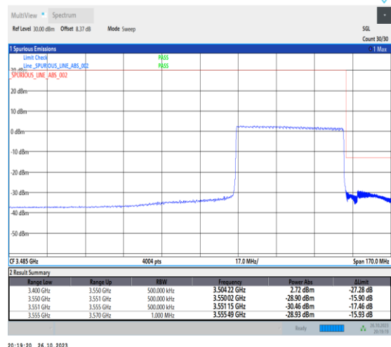
1-N78-3450-3550-PC2-30-50-H-6-CP-QPSK-Outer_Full-133@0-Ant0-1--PASS-see graph
