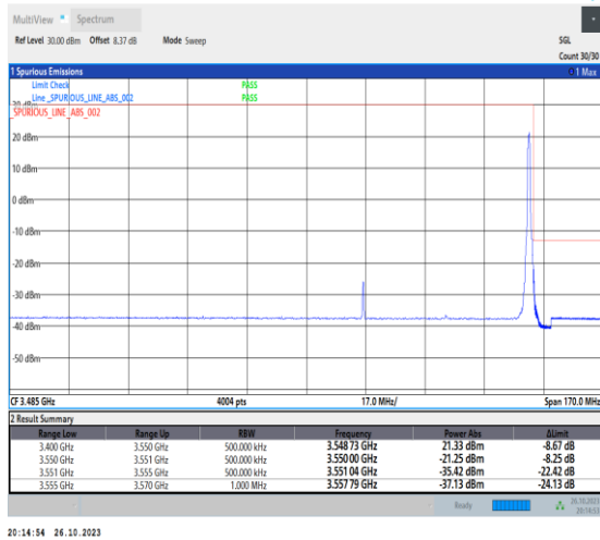
1-N78-3450-3550-PC2-30-50-H-2-DFT-PI2BPSK-Edge_1RB_Right-1@132-Ant0-1--PASS-see graph
