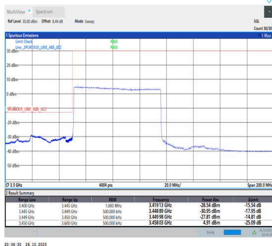
1-N78-3450-3550-PC2-30-70-L-3-DFT-PI2BPSK-Outer_Full-180@0-Ant0-1--PASS-see graph
