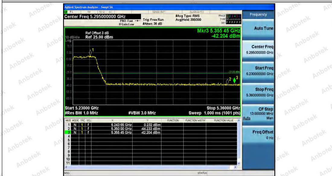
11AC40SISO_Ant1_High_5230
