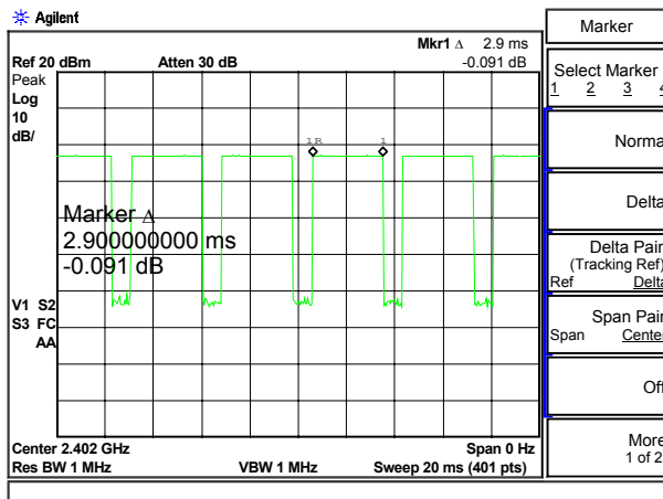
CH 00 2402MHz
