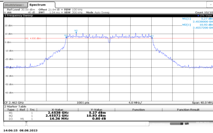
11G-CDD_Ant3_2462
