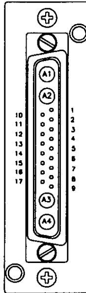
Figure 2-1. Amplifier Connector (on Rear of MCA 9503-60 Module)
