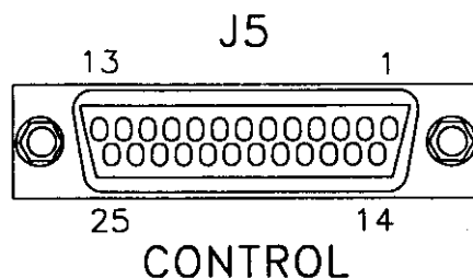
Figure 3-2. Connector J5
