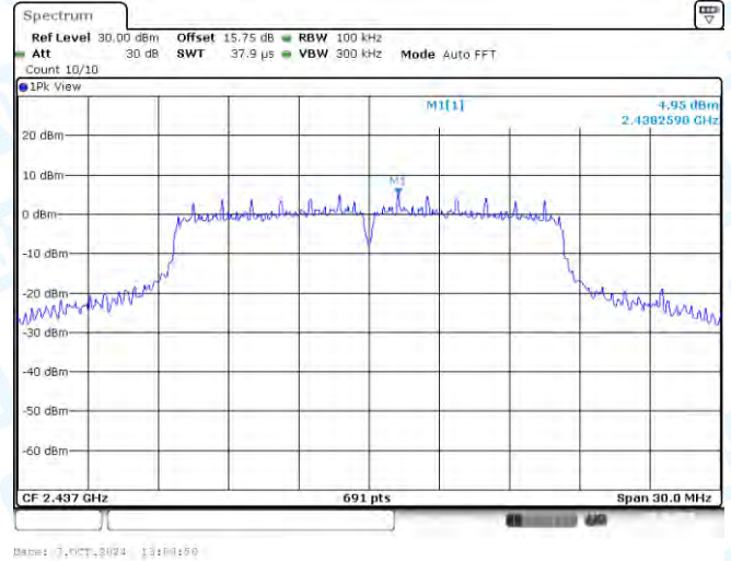
11G-Ant2-2437-0~Reference-PASS
