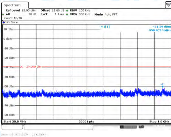
11AX40-CDD-Ant1-2437-30~1000-PASS
