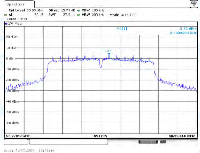
11G-Ant2-2462-0~Reference-PASS
