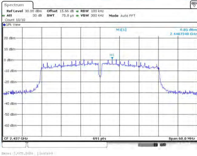
11N40-CDD-Ant1-2437-0~Reference-PASS
