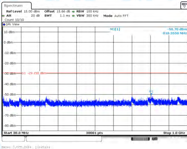
11N40-CDD-Ant1-2437-30~1000-PASS
