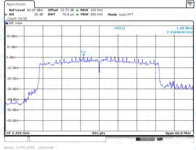
11AX40-CDD-Ant2-2422-0~Reference-PASS
