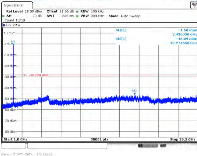
11G-CDD-Ant1-2437-1000~26500-PASS
