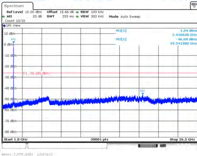
11G-Ant1-2412-1000~26500-PASS
