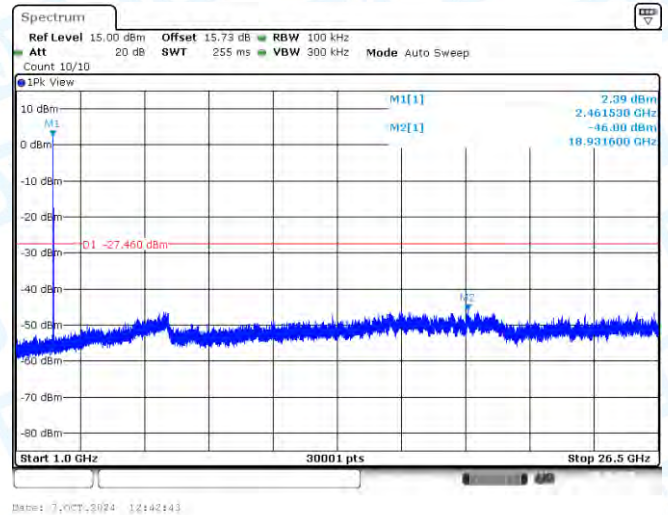
11B-Ant2-2462-1000~26500-PASS
