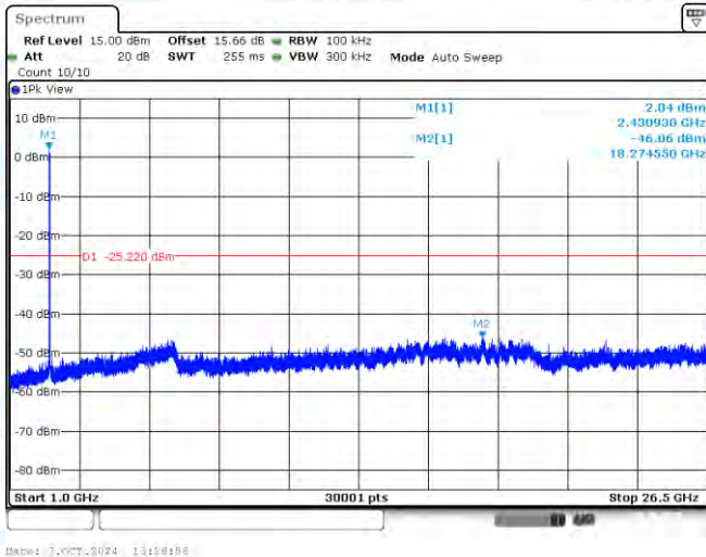
11N20-CDD-Ant1-2437-1000~26500-PASS
