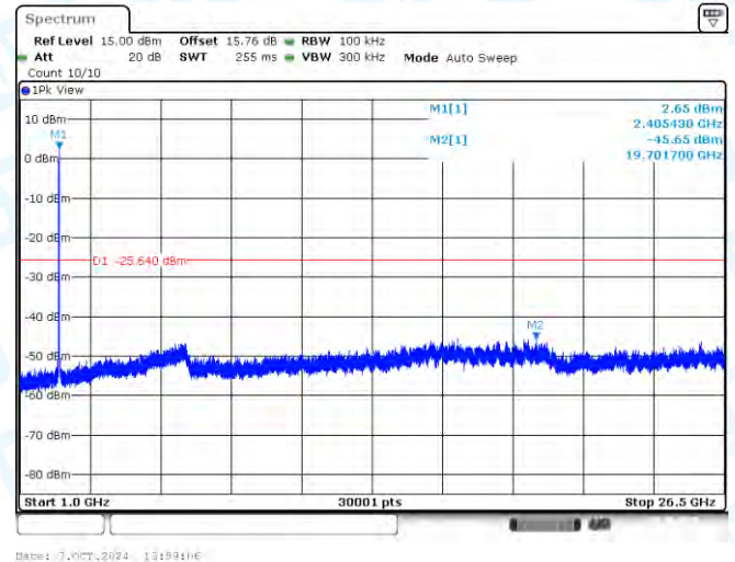
11AX20-CDD-Ant2-2412-1000~26500-PASS
