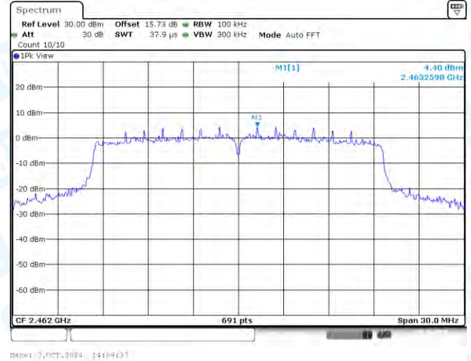
11AX20-CDD-Ant2-2462-0~Reference-PASS
