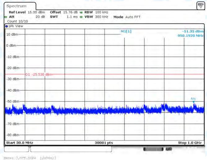
11G-Ant2-2412-30~1000-PASS
