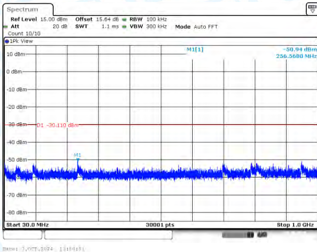
11N40-CDD-Ant1-2452-30~1000-PASS
