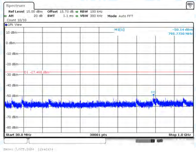
11B-Ant2-2462-30~1000-PASS
