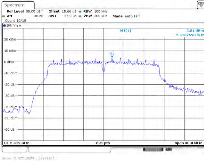
11G-Ant1-2412-0~Reference-PASS
