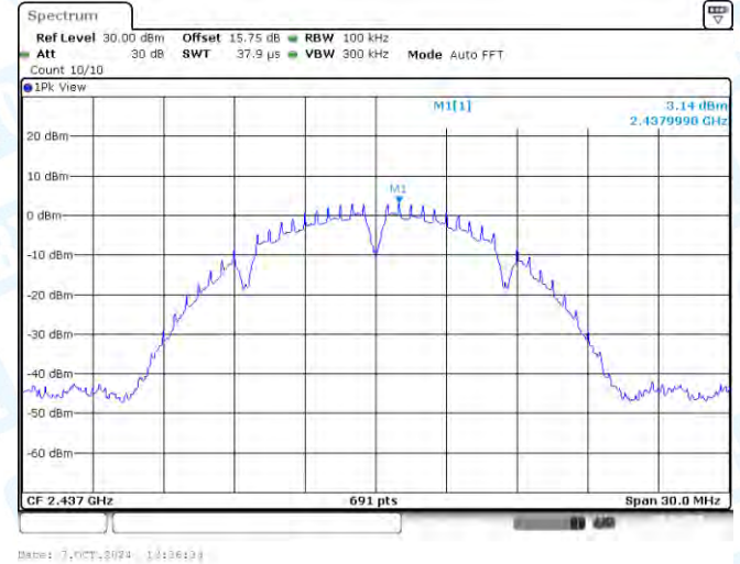
11B-CDD-Ant2-2437-0~Reference-PASS
