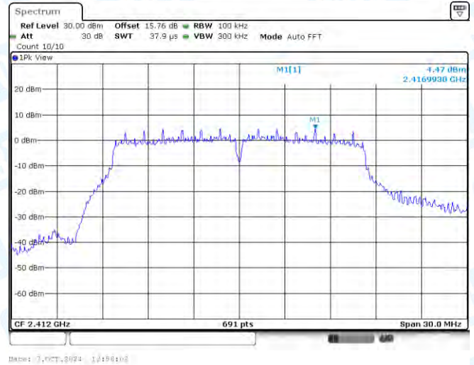
11G-Ant2-2412-0~Reference-PASS
