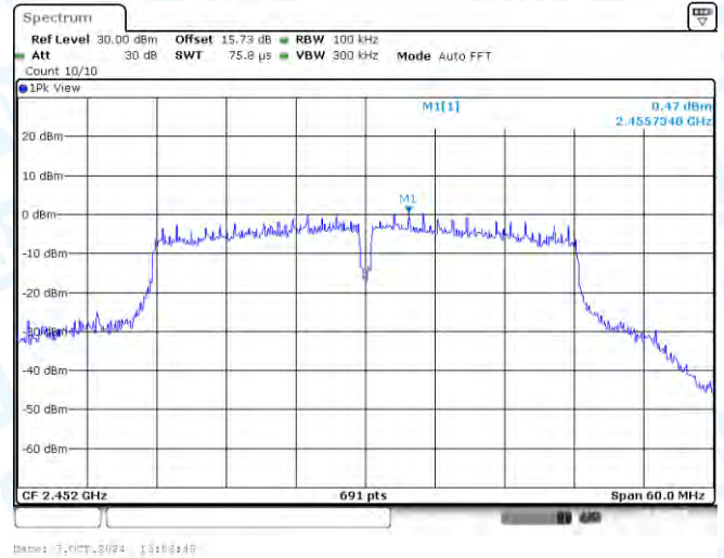
11N40-CDD-Ant2-2452-0~Reference-PASS
