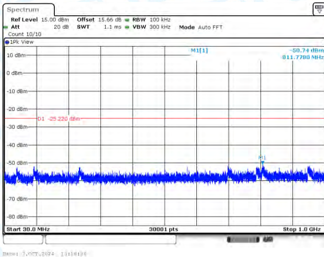
11N20-CDD-Ant1-2437-30~1000-PASS
