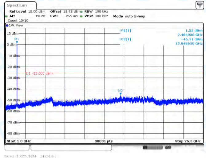
11AX20-CDD-Ant2-2462-1000~26500-PASS
