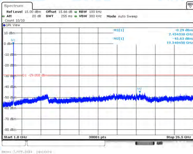
11AX40-CDD-Ant1-2437-1000~26500-PASS
