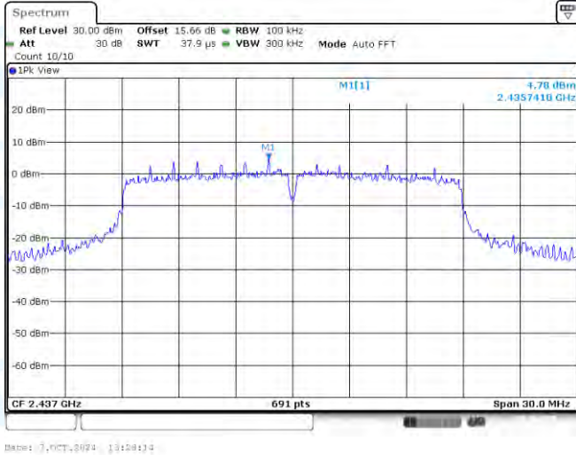
11N20-CDD-Ant1-2437-0~Reference-PASS
