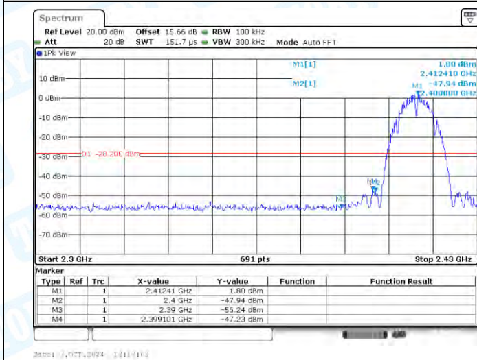
11B-CDD-Ant1-2412-PASS
