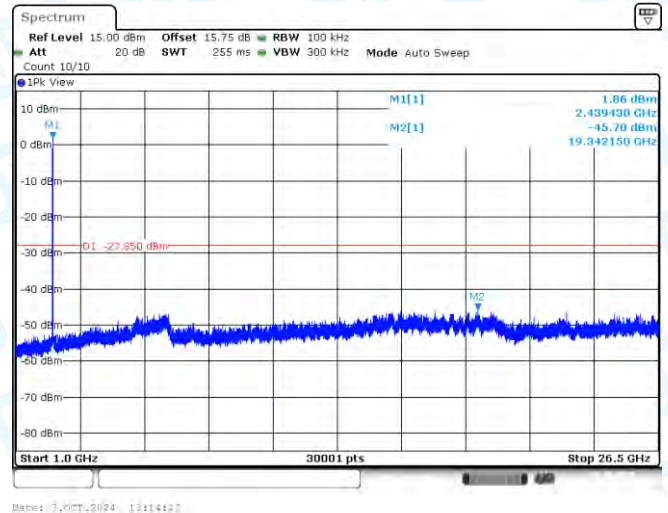
11G-CDD-Ant2-2437-1000~26500-PASS
