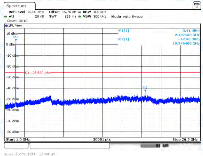
11G-Ant2-2412-1000~26500-PASS
