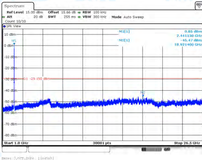
11N40-CDD-Ant1-2437-1000~26500-PASS
