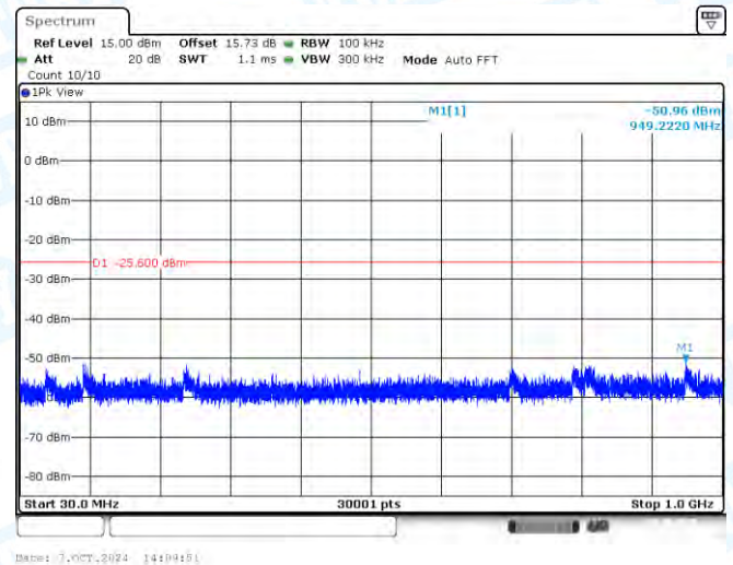
11AX20-CDD-Ant2-2462-30~1000-PASS
