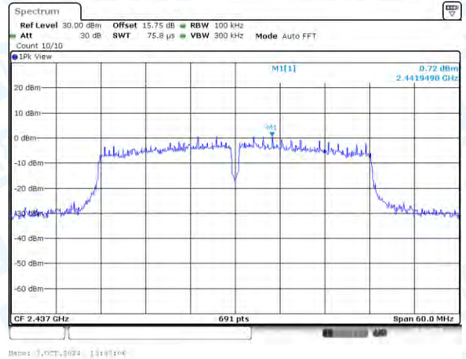
11N40-CDD-Ant2-2437-0~Reference-PASS
