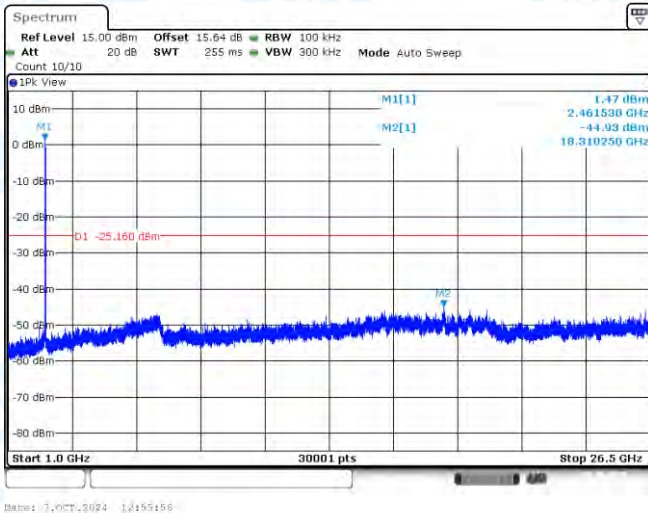
11G-Ant1-2462-1000~26500-PASS
