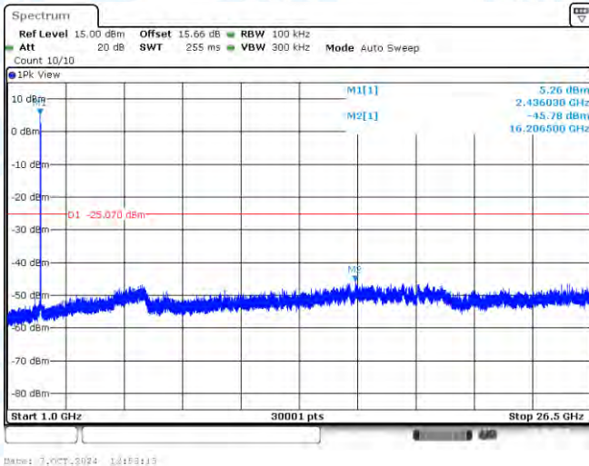
11G-Ant1-2437-1000~26500-PASS
