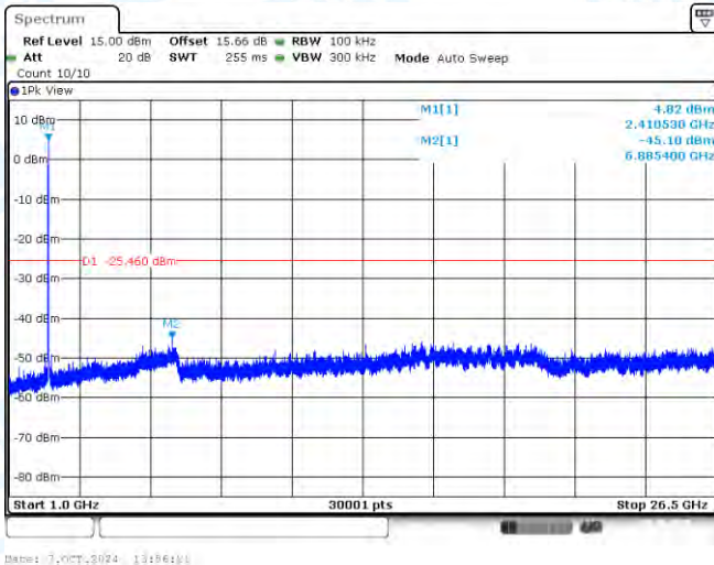
11AX20-CDD-Ant1-2412-1000~26500-PASS
