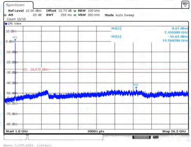
11G-Ant2-2462-1000~26500-PASS
