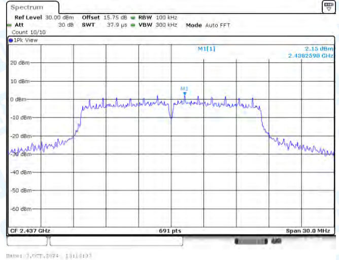
11G-CDD-Ant2-2437-0~Reference-PASS
