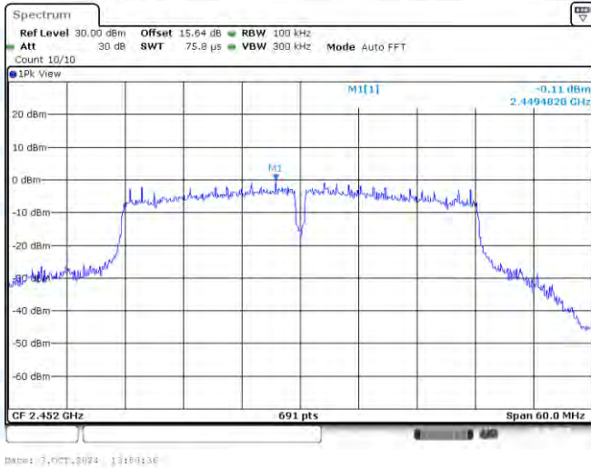
11N40-CDD-Ant1-2452-0~Reference-PASS
