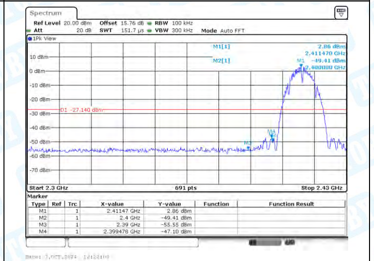
11B-CDD-Ant2-2412-PASS
