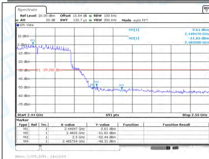
11AX40-CDD-Ant1-2452-PASS
