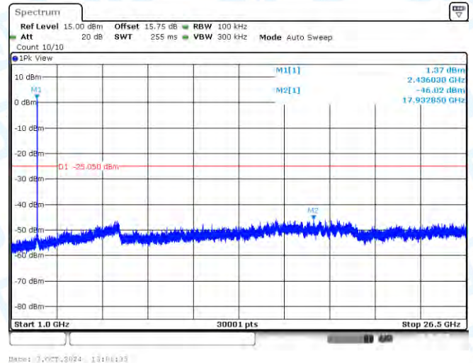
11G-Ant2-2437-1000~26500-PASS
