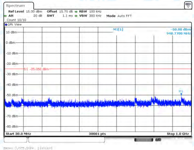
11G-Ant2-2437-30~1000-PASS
