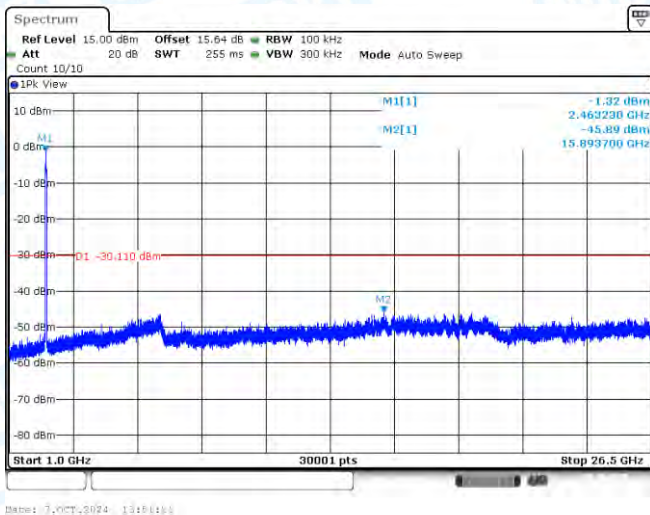
11N40-CDD-Ant1-2452-1000~26500-PASS
