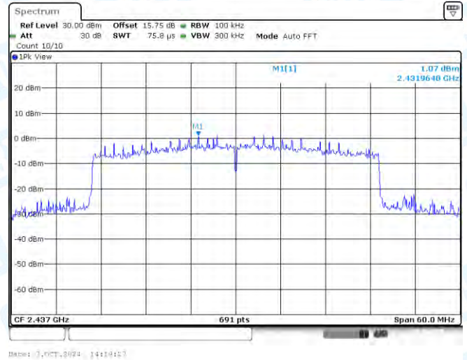
11AX40-CDD-Ant2-2437-0~Reference-PASS
