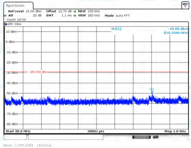
11AX40-CDD-Ant2-2437-30~1000-PASS
