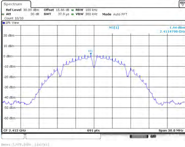
11B-CDD-Ant1-2412-0~Reference-PASS
