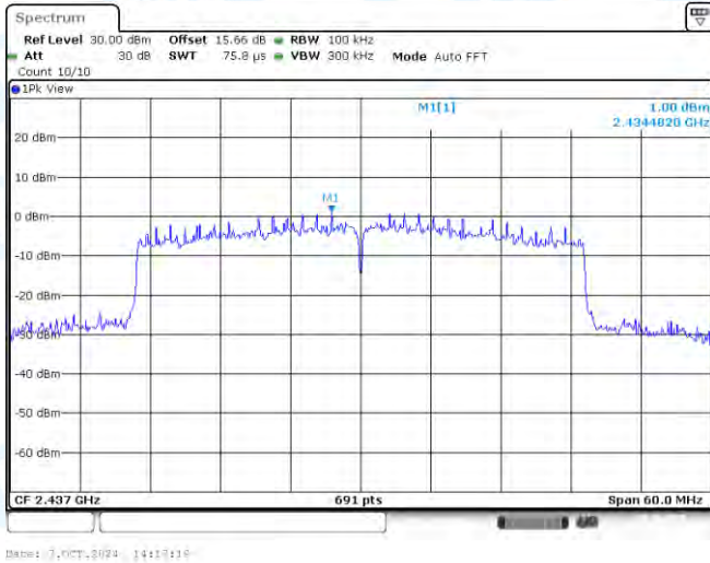
11AX40-CDD-Ant1-2437-0~Reference-PASS
