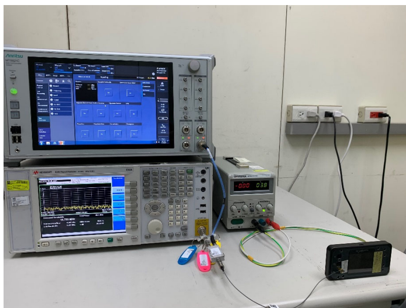
Conducted Setup Photo (Measurement at Antenna Port)
