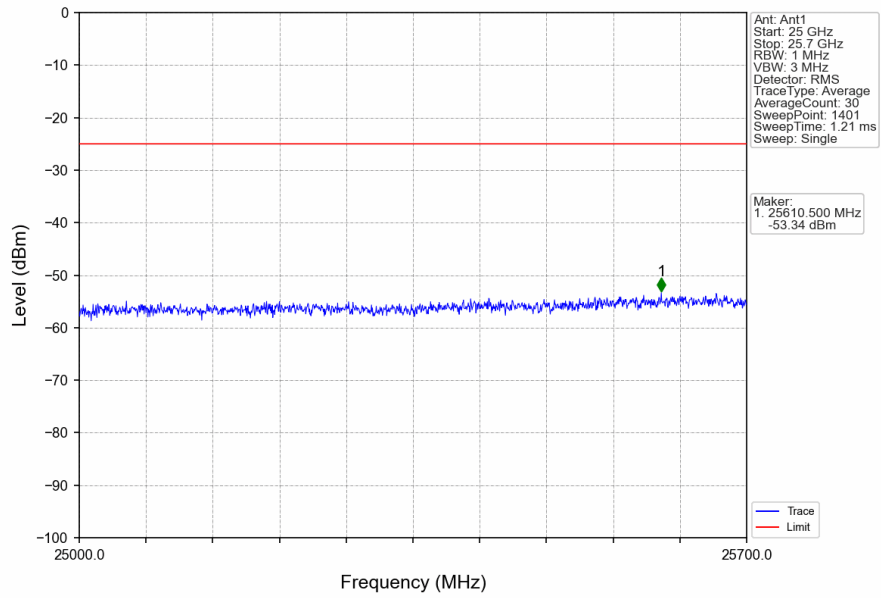
Band7_10MHz_16QAM_HCH_2565MHz_RB_1_0_NTNV
