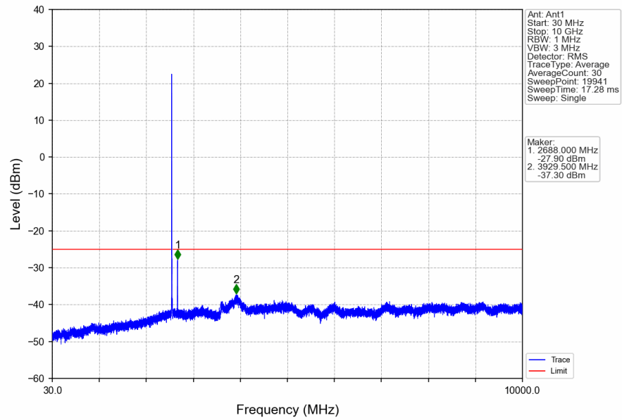
Band7_10MHz_16QAM_HCH_2565MHz_RB_1_0_NTNV
