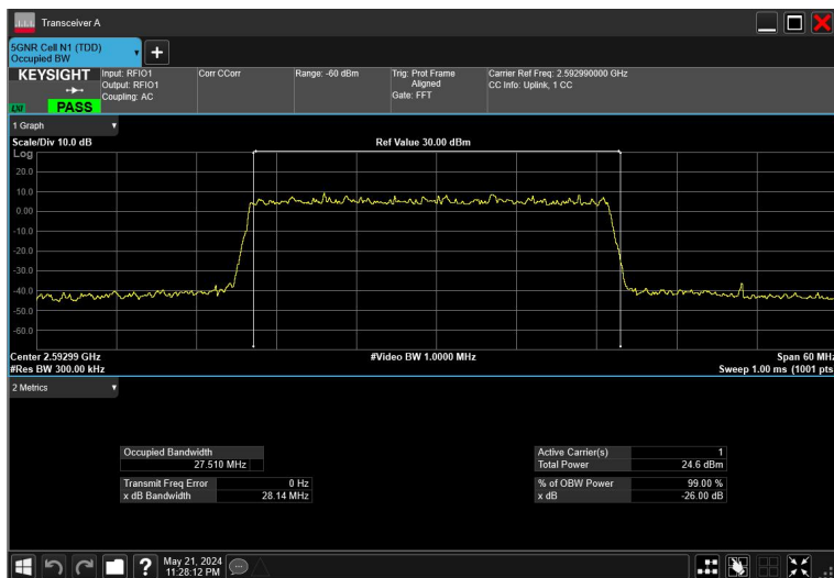
30MHz_30kHz_2592.99MHz_DFT-s-OFDM 256 QAM_RB75@0
