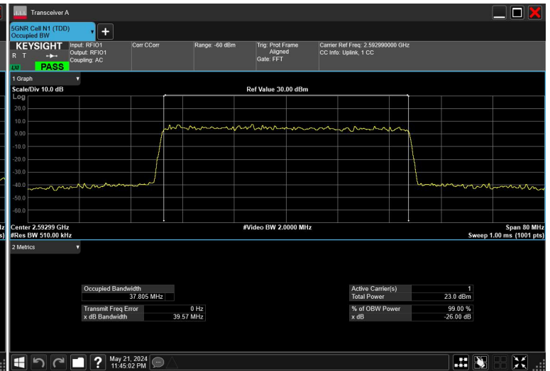
40MHz_30kHz_2592.99MHz_CP-OFDM 256 QAM_RB106@0
