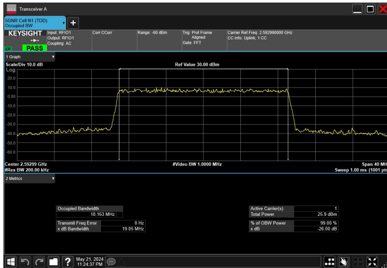
20MHz_30kHz_2592.99MHz_CP-OFDM 16 QAM_RB51@0
