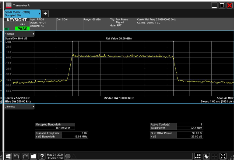
20MHz_30kHz_2592.99MHz_CP-OFDM 256 QAM_RB51@0
