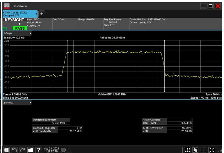
30MHz_30kHz_2592.99MHz_DFT-s-OFDM 64 QAM_RB75@0
