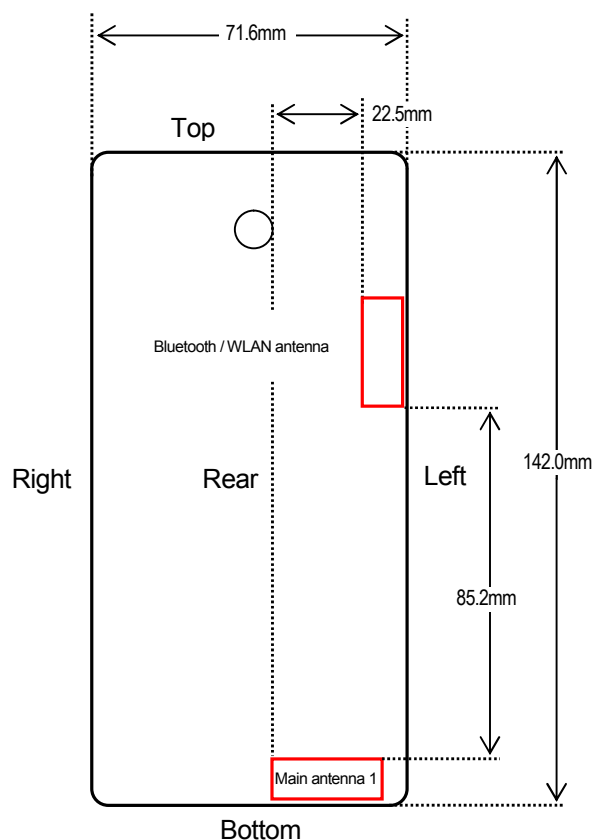
Main antenna 1 (GSM1900)
