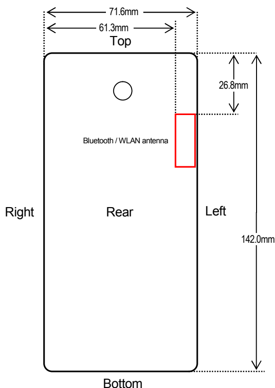
Bluetooth / WLAN antenna
