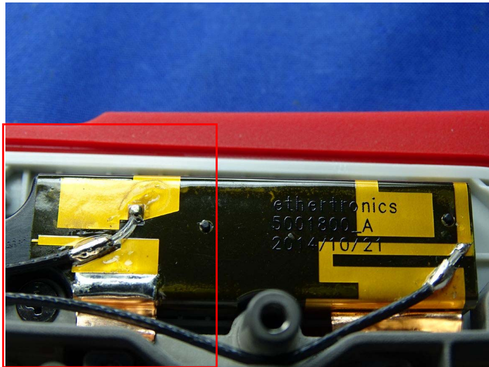
(39) EUT Photo - left GPS Ant
