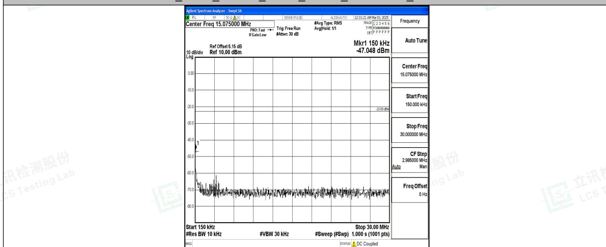
Band5_3MHz_16QAM_20525_1RB#0_0.15~30_0.15~30
