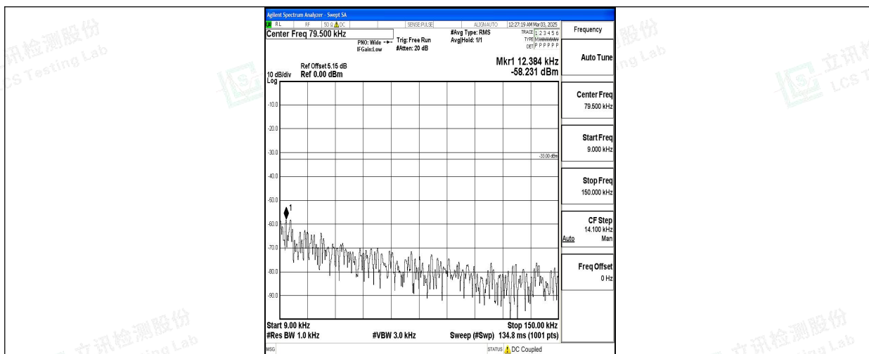
Band5_1.4MHz_16QAM_20525_1RB#0_0.009~0.15_0.009~0.15
