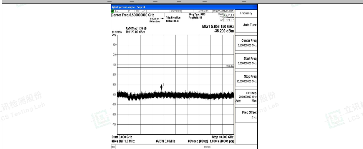
Band5_3MHz_QPSK_20415_1RB#0_3000~10000_3000~10000
