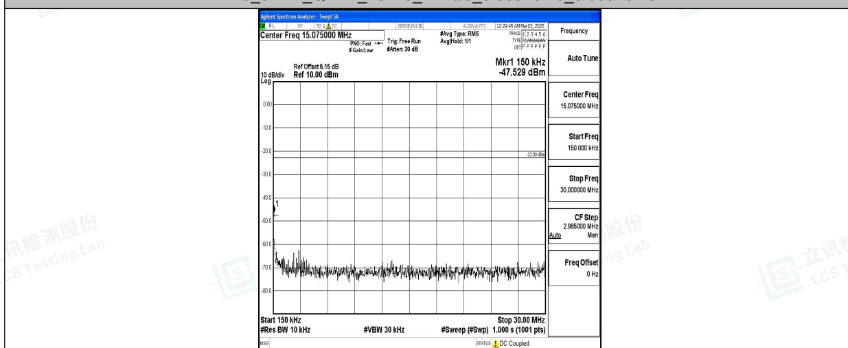
Band5_3MHz_QPSK_20415_1RB#0_0.15~30_0.15~30
