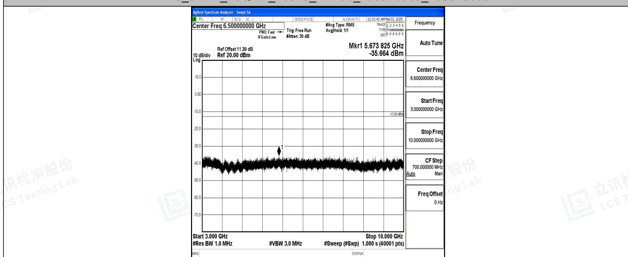
Band5_3MHz_16QAM_20525_1RB#0_3000~10000_3000~10000
