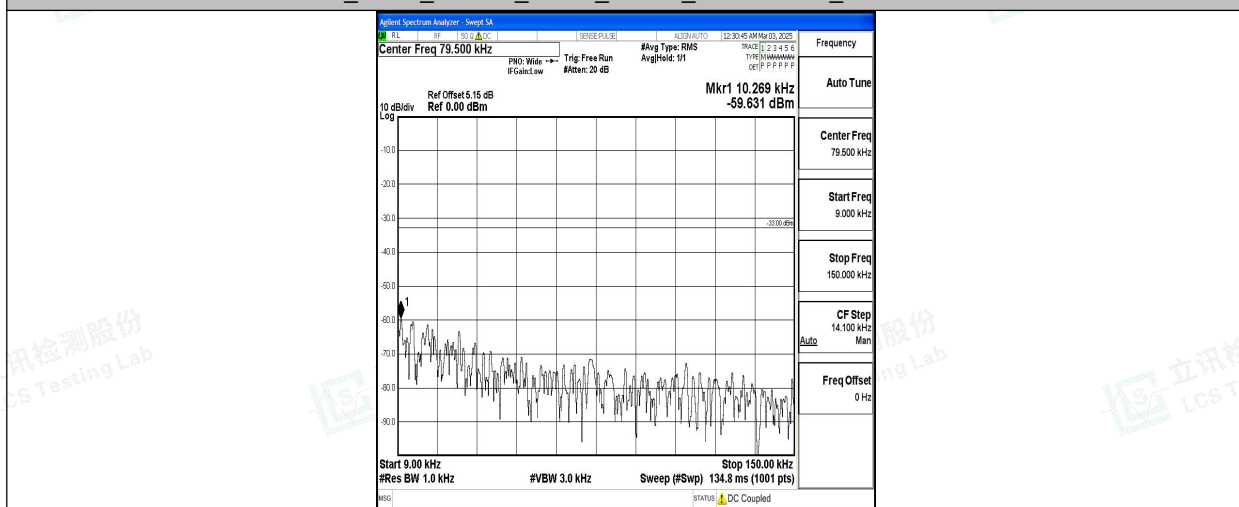
Band5_3MHz_QPSK_20525_1RB#0_0.009~0.15_0.009~0.15
