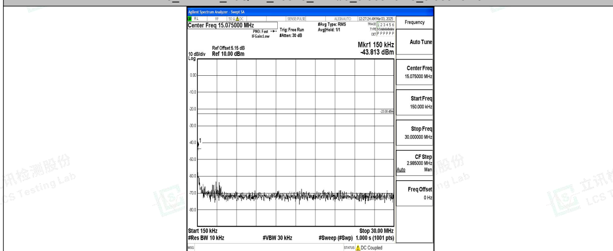
Band5_1.4MHz_16QAM_20525_1RB#0_0.15~30_0.15~30
