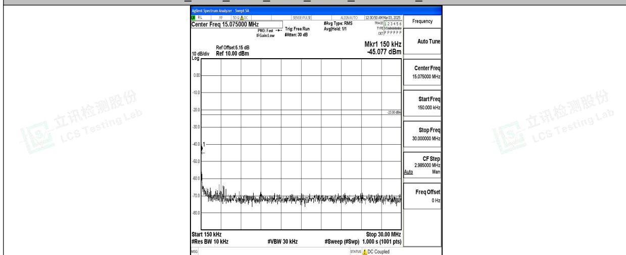
Band5_3MHz_QPSK_20525_1RB#0_0.15~30_0.15~30
