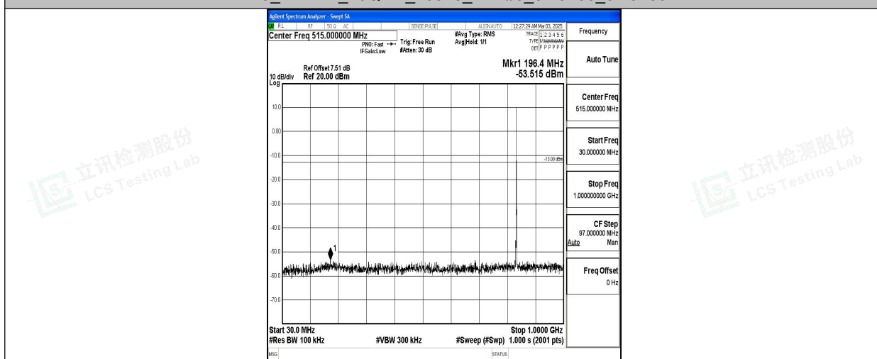
Band5_1.4MHz_16QAM_20525_1RB#0_30~1000_30~1000
