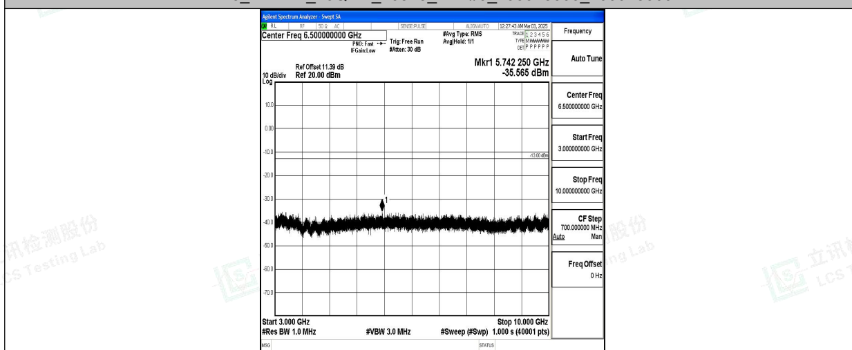
Band5_1.4MHz_16QAM_20525_1RB#0_3000~10000_3000~10000
