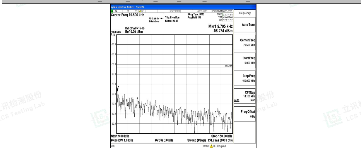
Band5_1.4MHz_QPSK_20525_1RB#0_0.009~0.15_0.009~0.15
