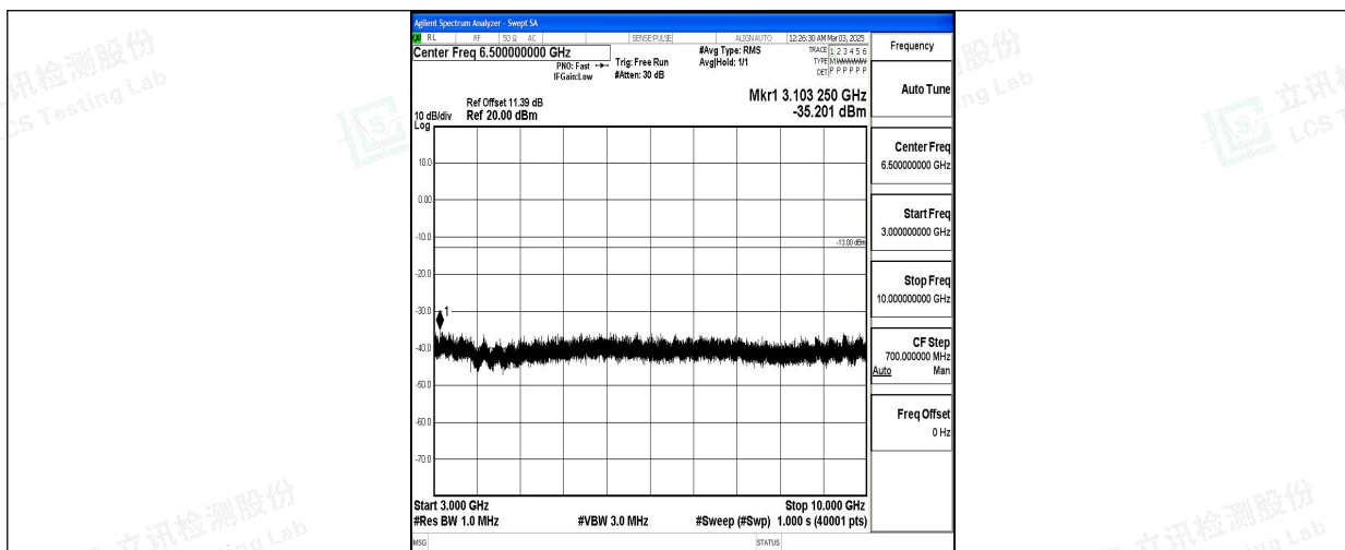
Band5_1.4MHz_16QAM_20407_1RB#0_3000~10000_3000~10000
