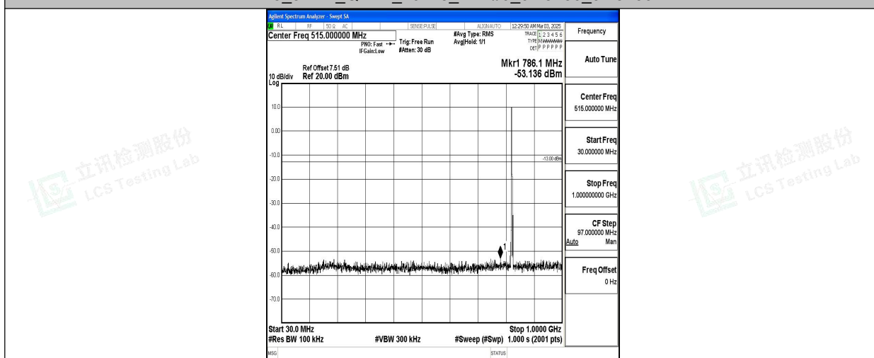
Band5_3MHz_QPSK_20415_1RB#0_30~1000_30~1000
