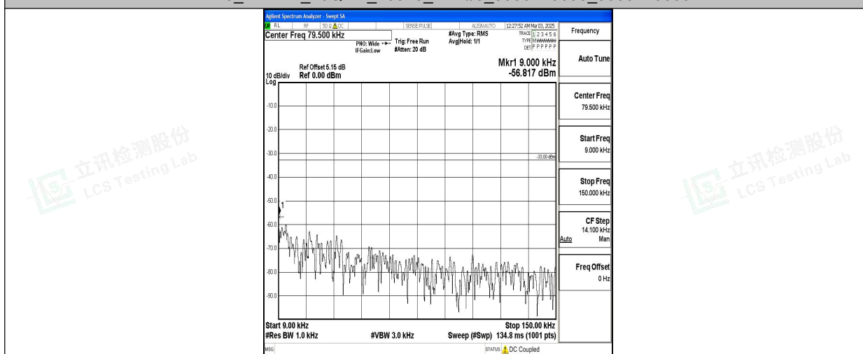
Band5_1.4MHz_QPSK_20643_1RB#0_0.009~0.15_0.009~0.15
