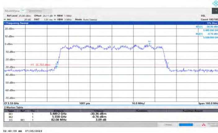
11AC80SISO_Ant3_5530
