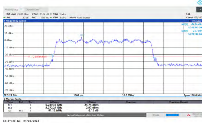
11AC80SISO_Ant3_5290
