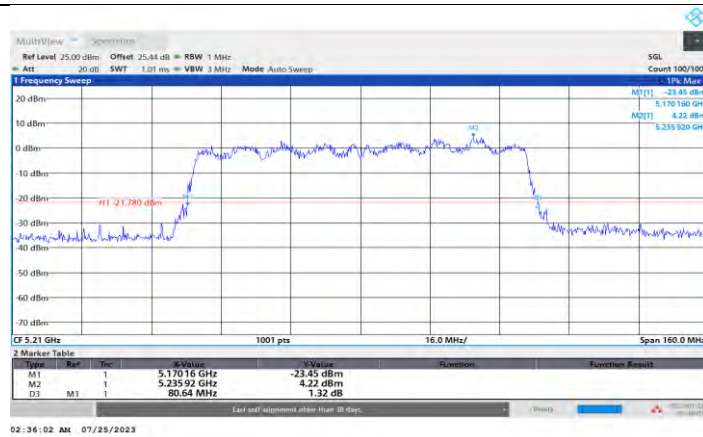
11AC80SISO_Ant3_5210
