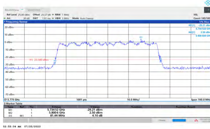
11AC80SISO_Ant3_5775
