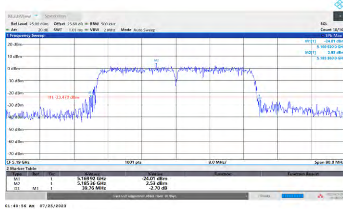
11N40SISO_Ant3_5190
