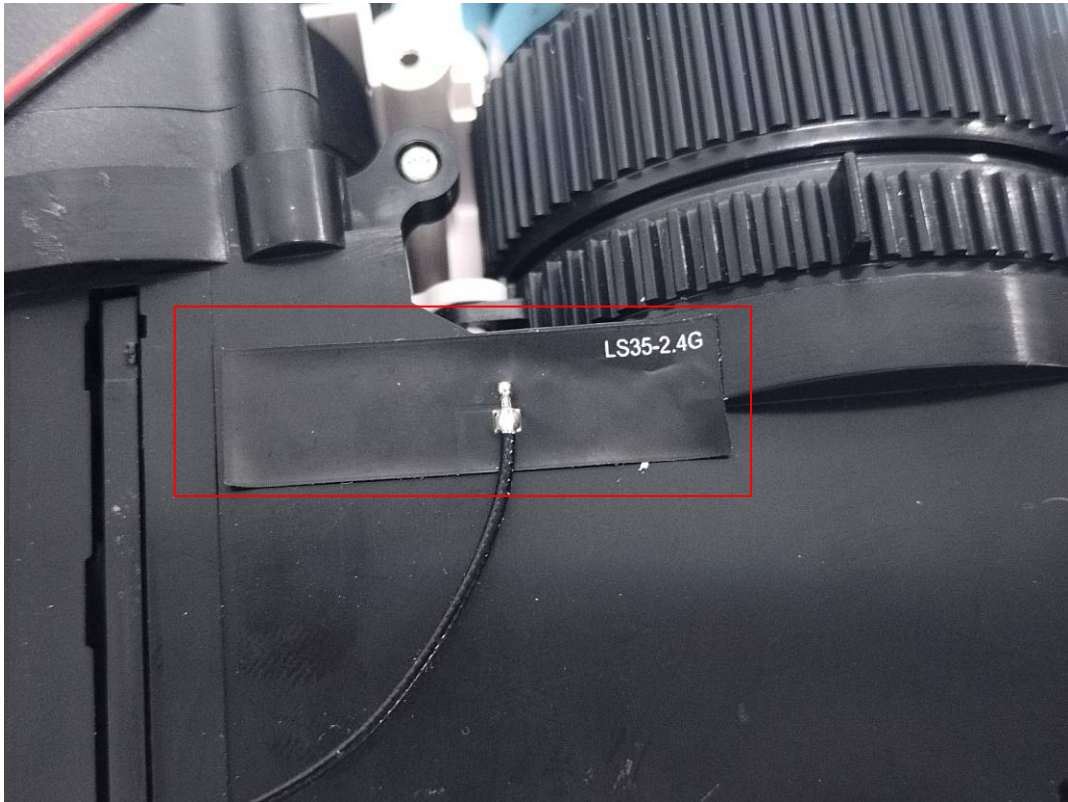
ANT WiFi
