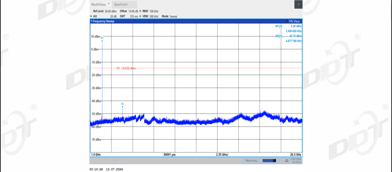
2.4G SRD_Ant1_2479_0~Reference
