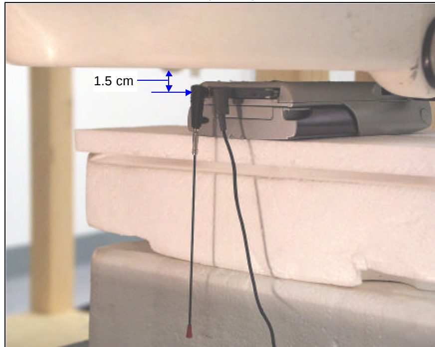
EUT Set-up Configuration 2
