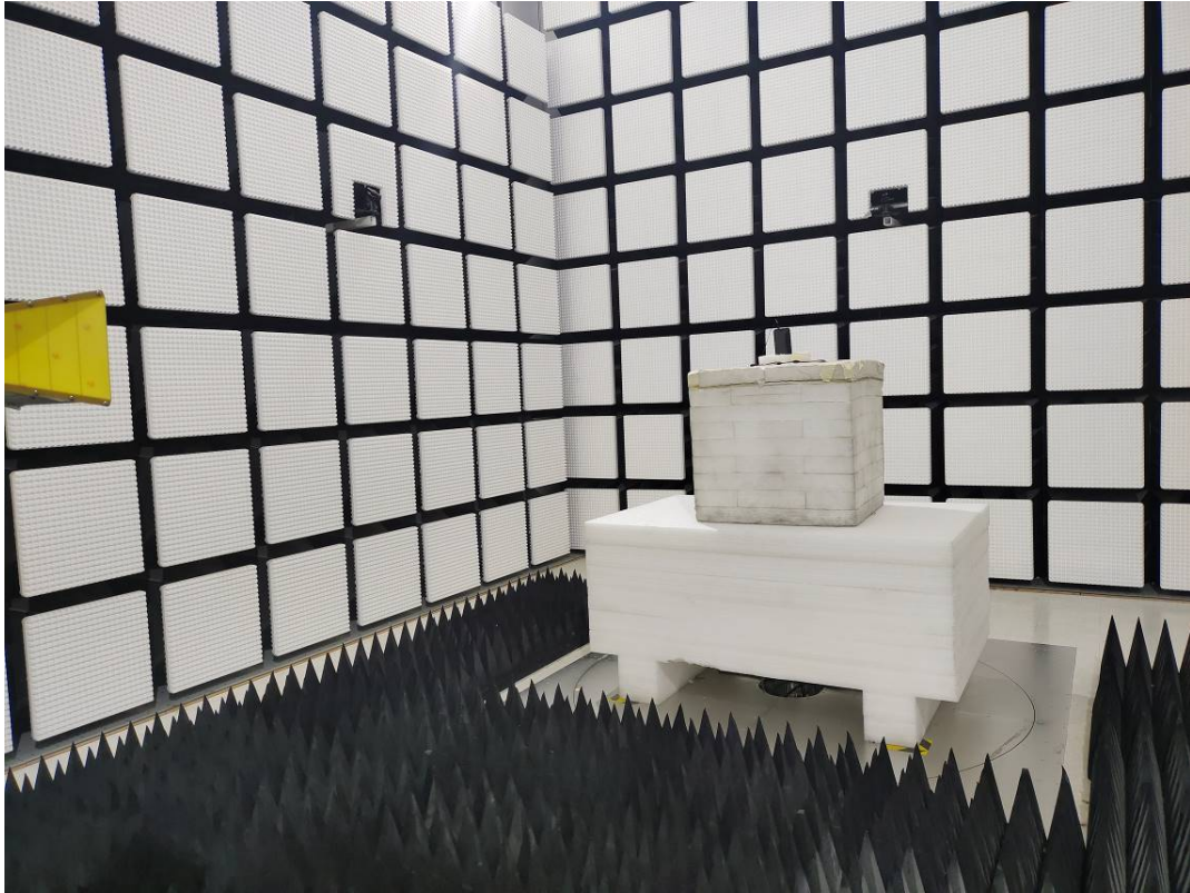
Radiated Emission Above 1GHz View Adapter 1
