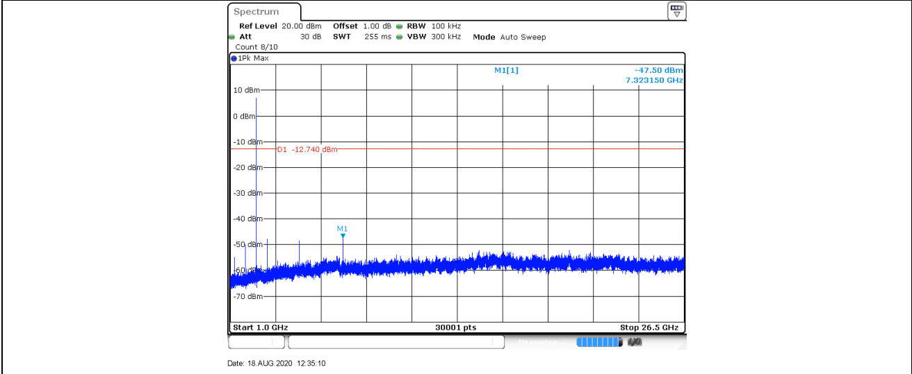
2DH5_Ant1_2480_0-Reference
