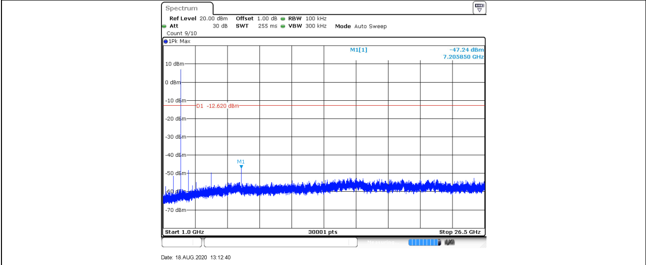
3DH5_Ant1_2441_0-Reference
