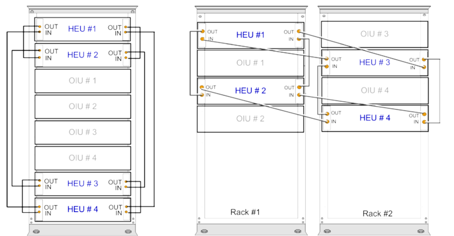
Figure 5-14. Pilot Clock Connections Diagram Figure 5-15 Pilot Clock Connections Diagram – (4x4) Dedicated Rack – (4x4) Shared Rack
