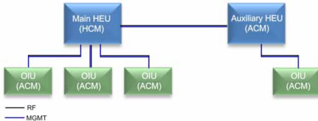
Figure 5-1. Example of Management and RF Connections for Main and Auxiliary HEU Units
