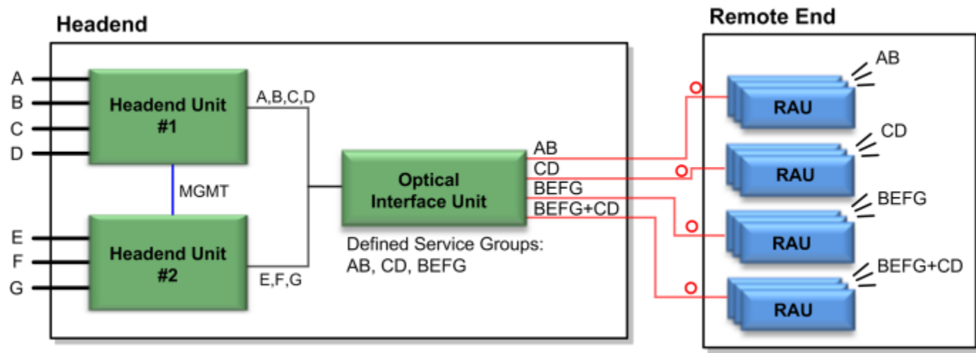
Figure 1-12. Example of Tri-Service Group Configuration with Two HEUs
