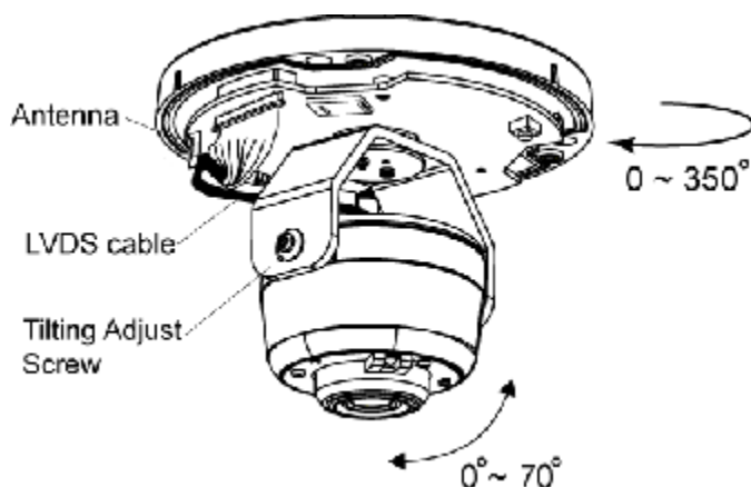
Figure 6: Angle Adjustment
