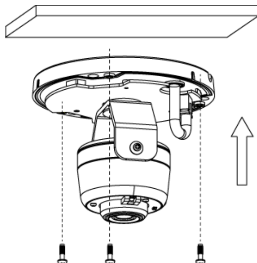
Figure 5: Ceiling Installation
