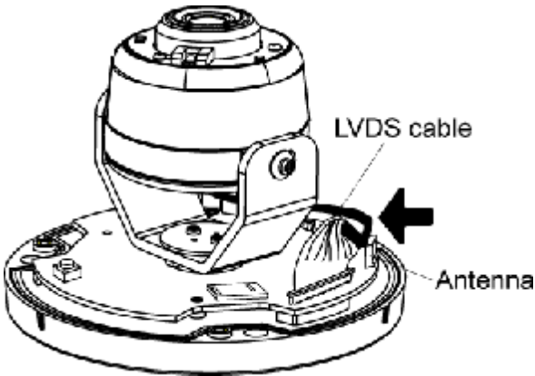
Figure 7: LVDS Cable
