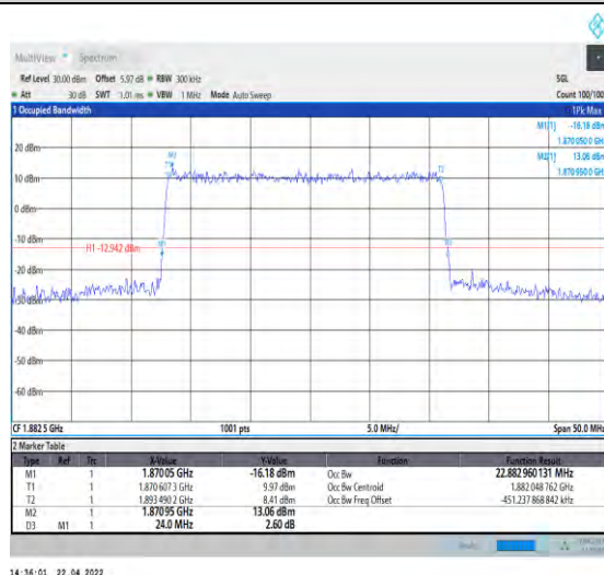
1-N25--15-25-M-3-DFT-16QAM-Outer_Full-128@0-A nt1-22.883-24.000-≤25-PASS
