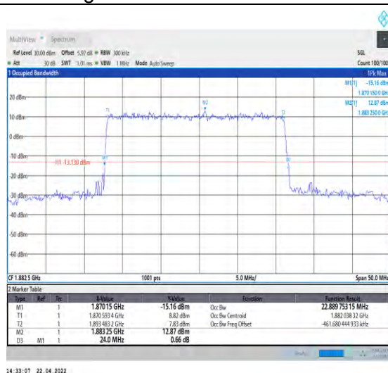
1-N25--15-25-M-1-DFT-QPSK-Outer_Full-128@0-An t1-22.89-24.000-≤25-PASS
