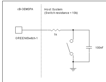
Figure 26: A low resistance restore switch used. Notice the 10k \Omega serial resistor.
