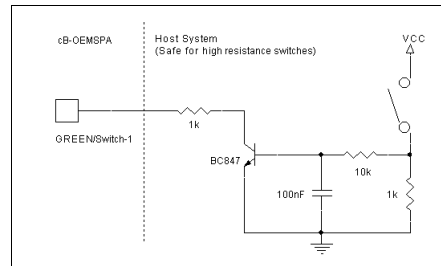
Figure 27: If the resistance in the switch is not guaranteed to be low enough, a safer design can be used. Notice the 10k \Omega serial resistor.
