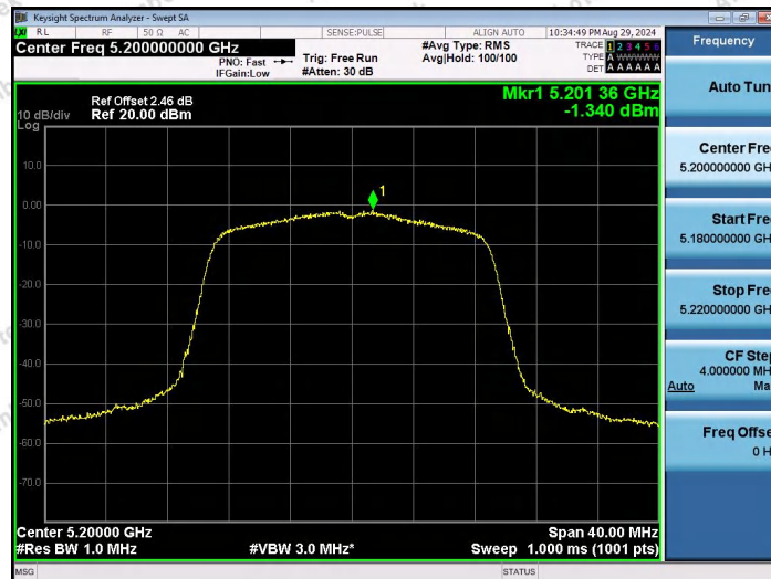
11N20SISO-Ant1-5200-PASS
