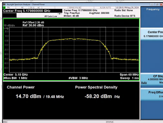
11A-Ant1-5180-PASS
