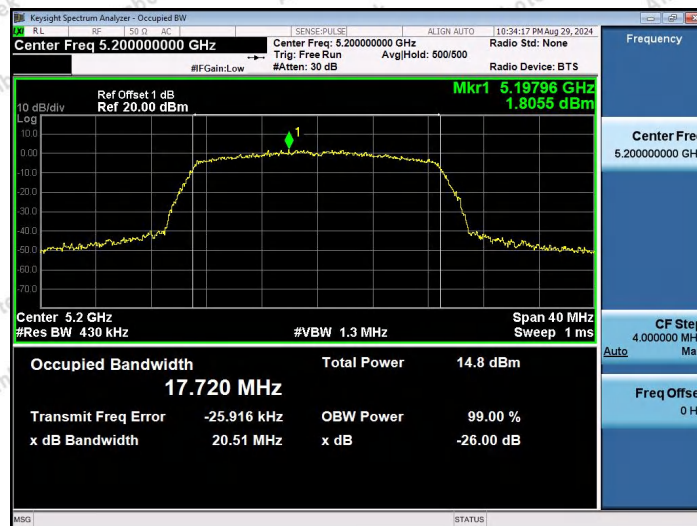
11N20SISO-Ant1-5200
