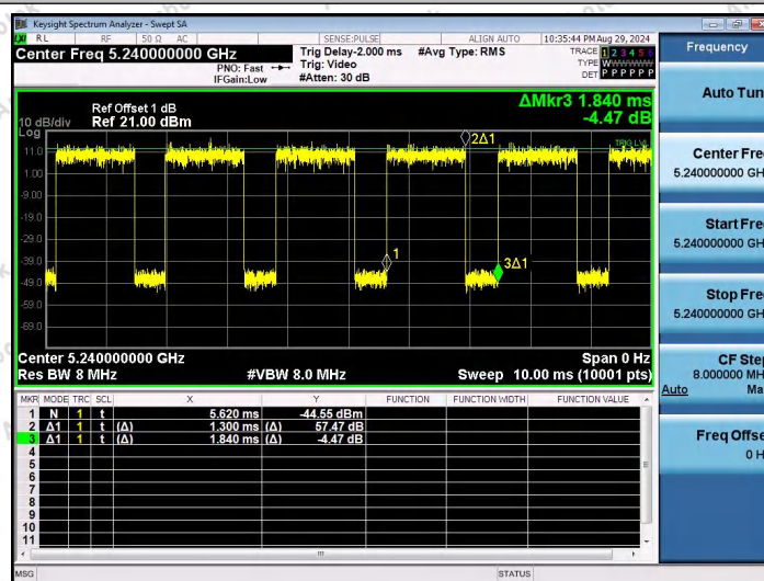
NTNV-11N20SISO-Ant1-5240
