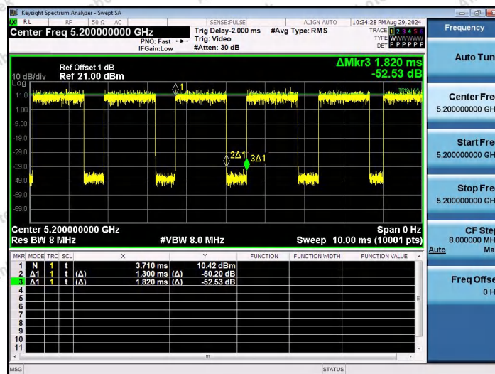
NTNV-11N20SISO-Ant1-5200
