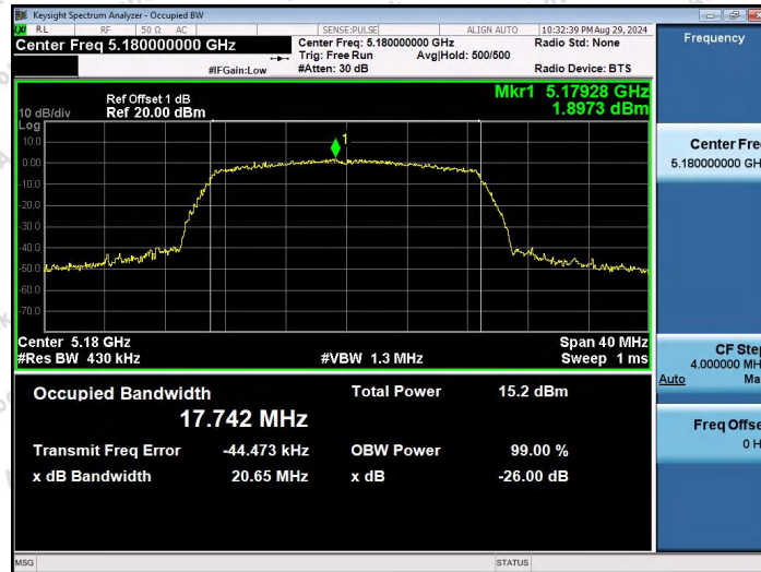
11N20SISO-Ant1-5180
