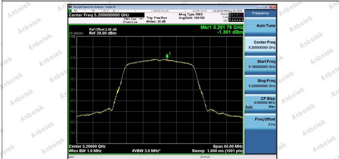
11A-Ant1-5200-PASS
