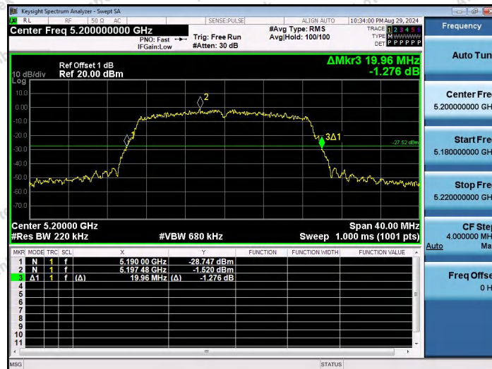
11N20SISO-Ant1-5200
