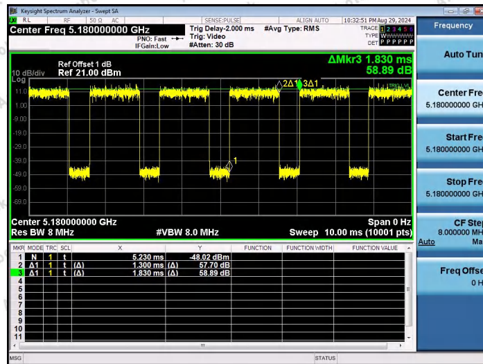
NTNV-11N20SISO-Ant1-5180
